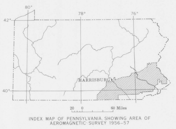
INDEX MAP OF PENNSYLVANIA SHOWING AREA OF AEROMAGNETIC SURVEY 1956-57
