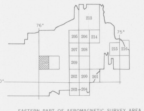
EASTERN PART OF AEROMAGNETIC SURVEY AREA SHOWING LOCATION OF THIS REPORT
