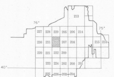
EASTERN PART OF AEROMAGNETIC SURVEY AREA SHOWING LOCATION OF THIS REPORT
