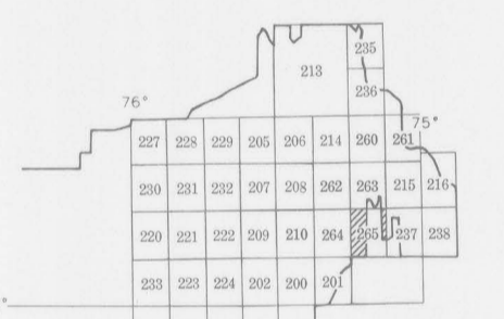
EASTERN PART OF AEROMAGNETIC SURVEY AREA SHOWING LOCATION OF THIS REPORT
