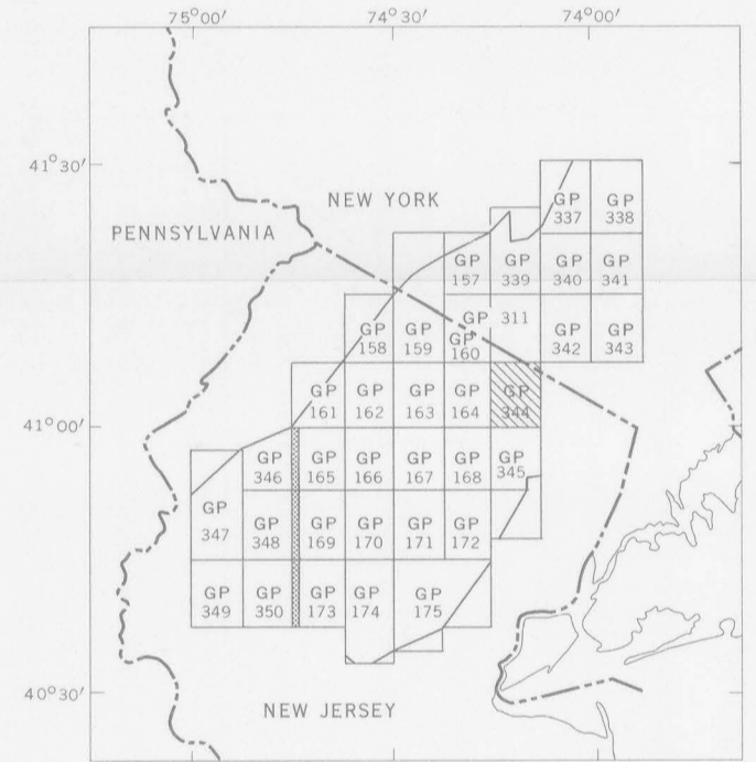
INDEX MAP SHOWING LOCATION OF AEROMAGNETIC MAPS PUBLISHED BY THE U.S. GEOLOGICAL SURVEY IN THE NEW YORK-NEW JERSEY HIGHLANDS AREA
