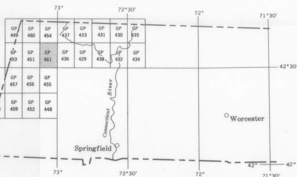
INDEX MAP OF WESTERN MASSACHUSETTS SHOWING AEROMAGNETIC MAPS PUBLISHED BY THE U.S. GEOLOGICAL SURVEY. AREA OF GP-461 SHADED
