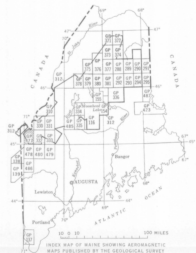
INDEX MAP OF MAINE SHOWING AEROMAGNETIC MAPS PUBLISHED BY THE GEOLOGICAL SURVEY AREA OF GP-477 SHADED
