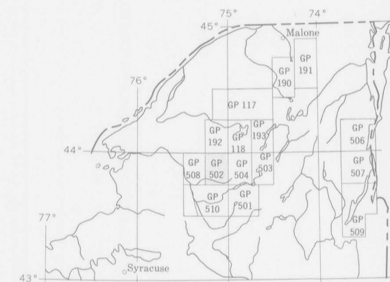
INDEX MAP OF NORTHERN NEW YORK SHOWING AEROMAGNETIC MAPS PUBLISHED BY THE U.S. GEOLOGICAL SURVEY AREA OF GP-502 SHADED
