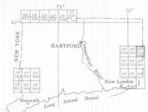
INDEX MAP OF CONNECTICUT SHOWING AEROMAGNETIC MAPS PUBLISHED BY THE U.S. GEOLOGICAL SURVEY. AREA OF GP-542 SHADED
