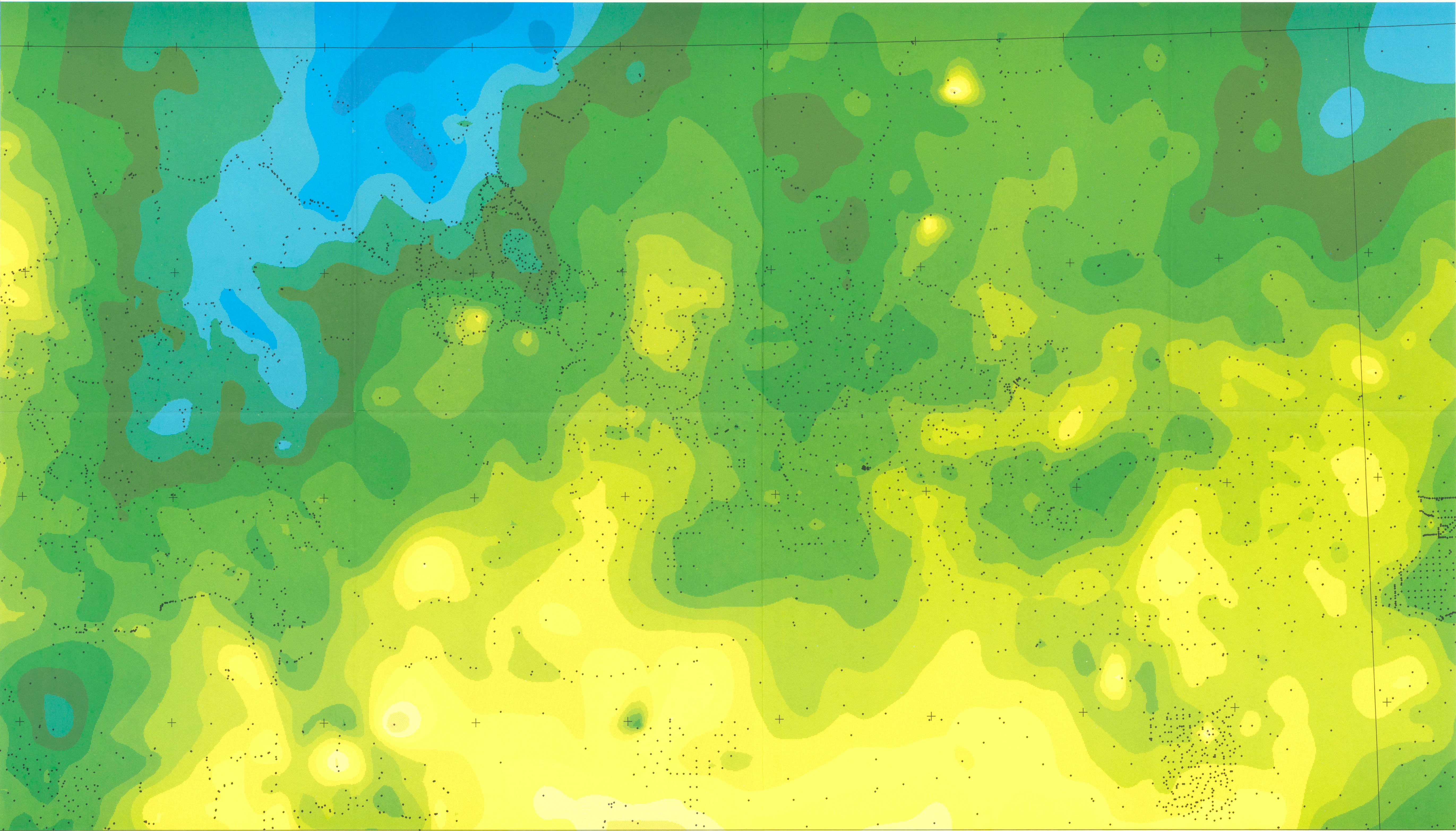
MAP C3. NORTHEAST SECTION OF COMPLETE BOUGUER GRAVITY ANOMALY
