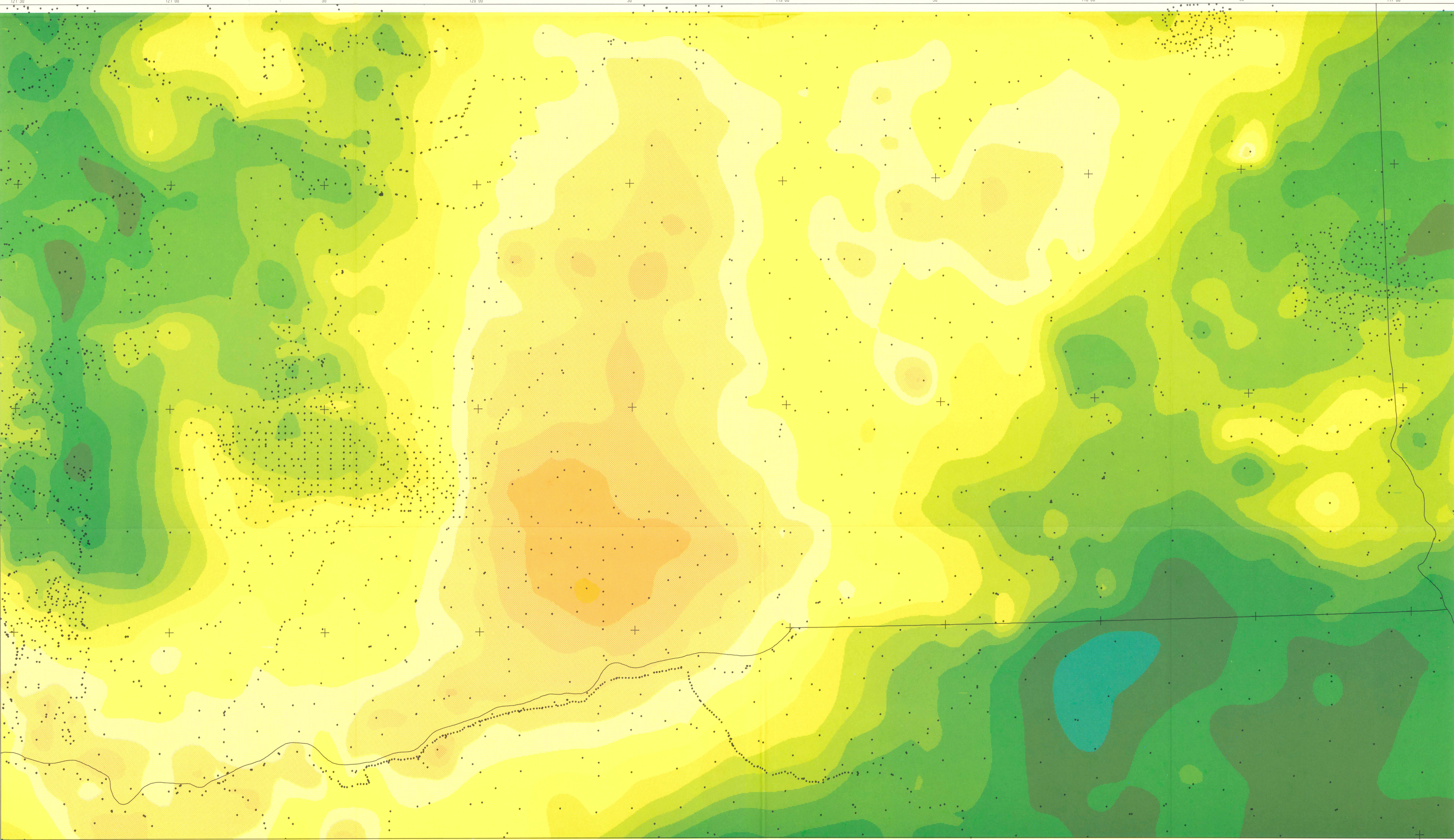
MAP C4. SOUTHEAST SECTION OF COMPLETE BOUGUER GRAVITY ANOMALY
