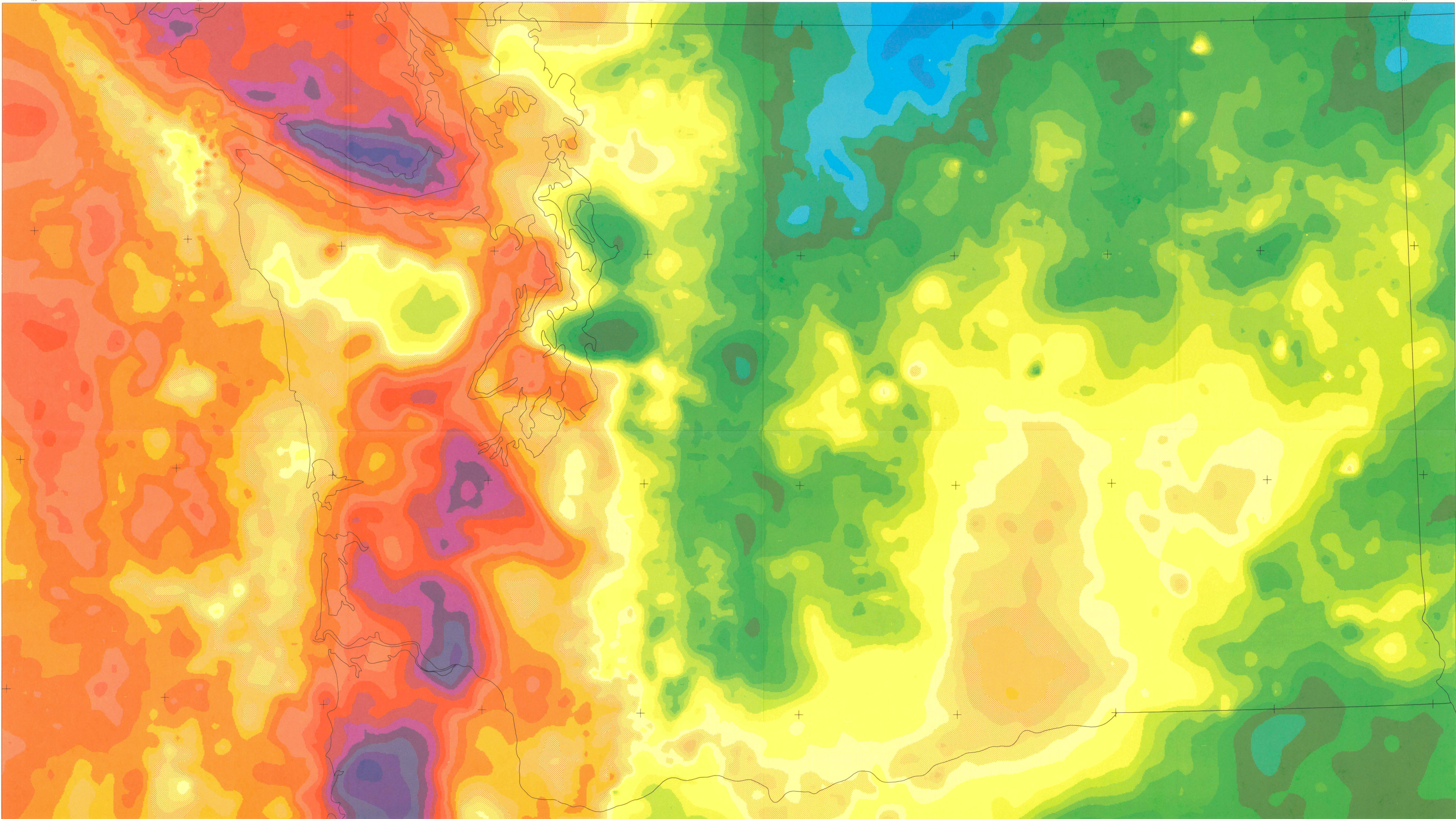
MAP D. COMPLETE BOUGUER GRAVITY ANOMALY
