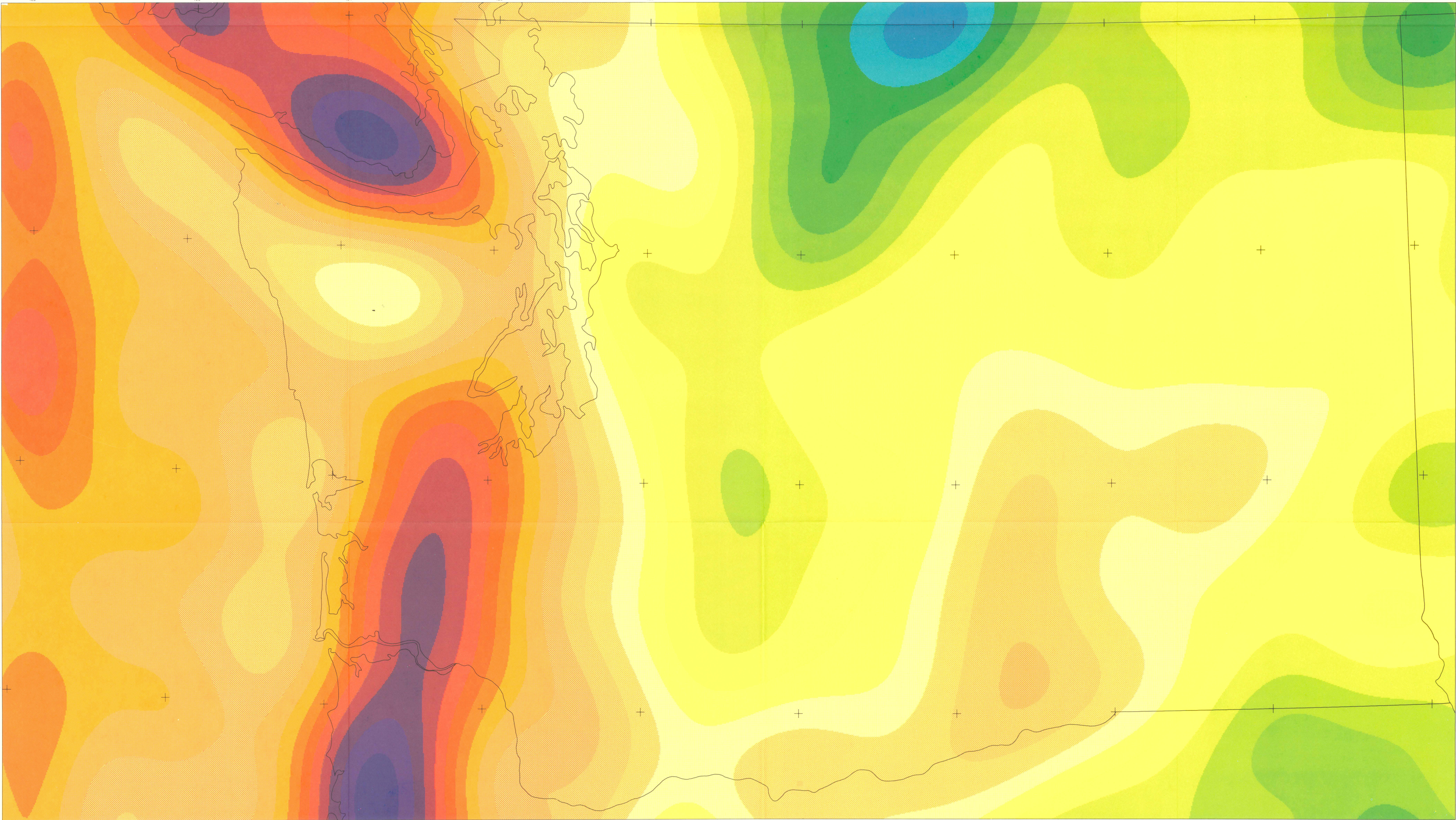
MAP E. REGIONAL WAVELENGTH-FILTERED GRAVITY ANOMALY
