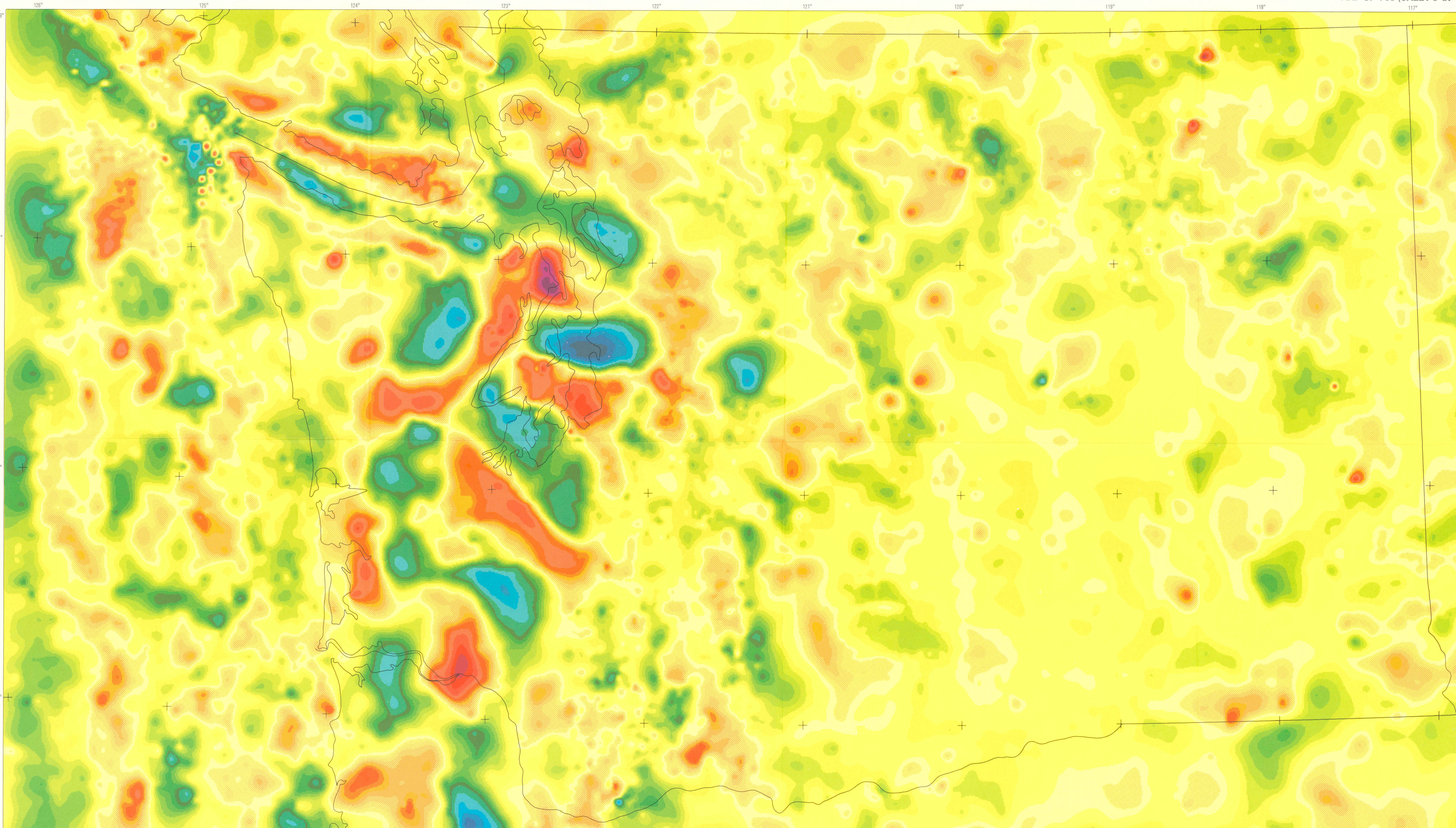
MAP F. RESIDUAL WAVELENGTH-FILTERED GRAVITY ANOMALY
