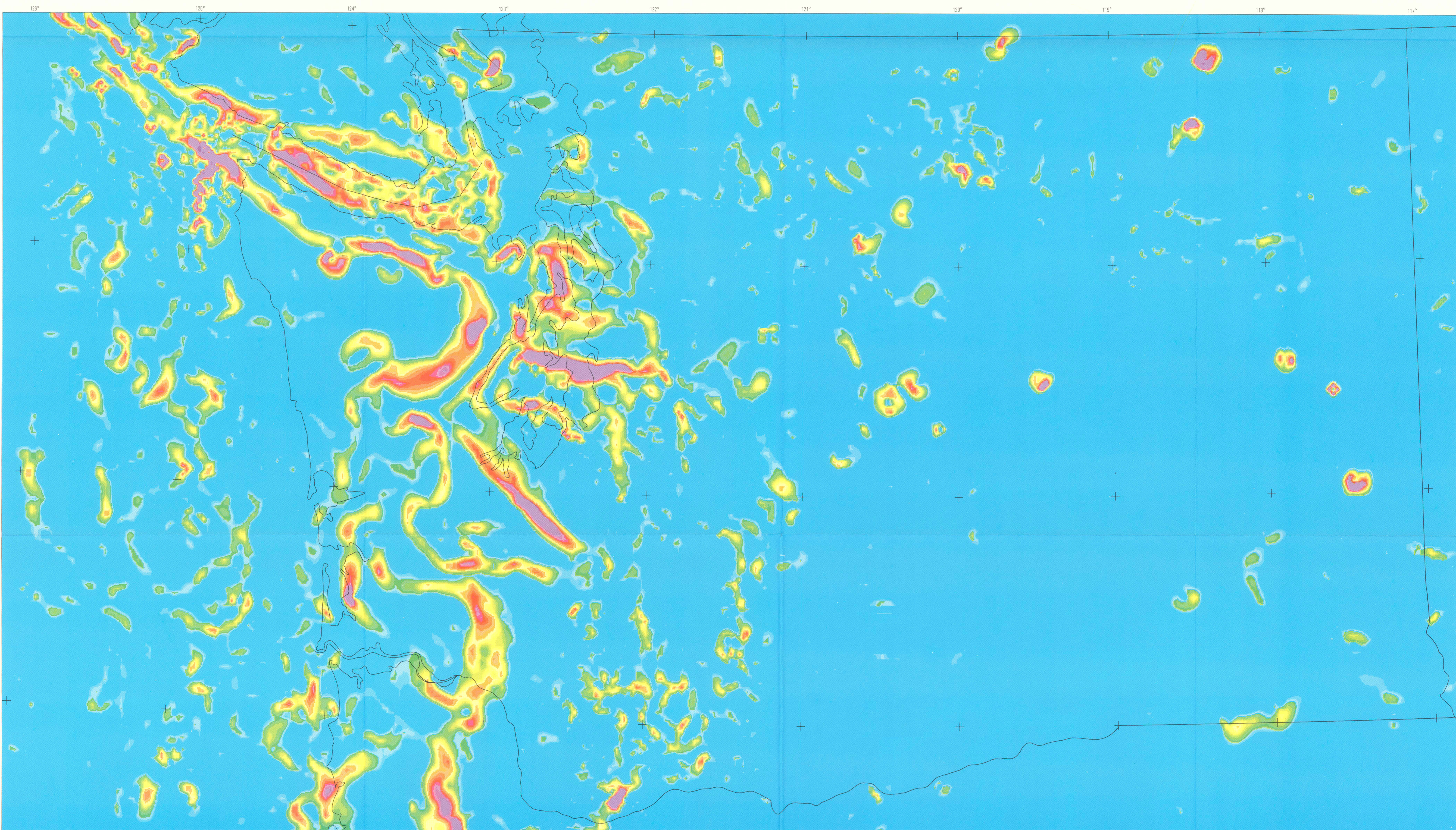
MAP G. HORIZONTAL GRAVITY GRADIENT
