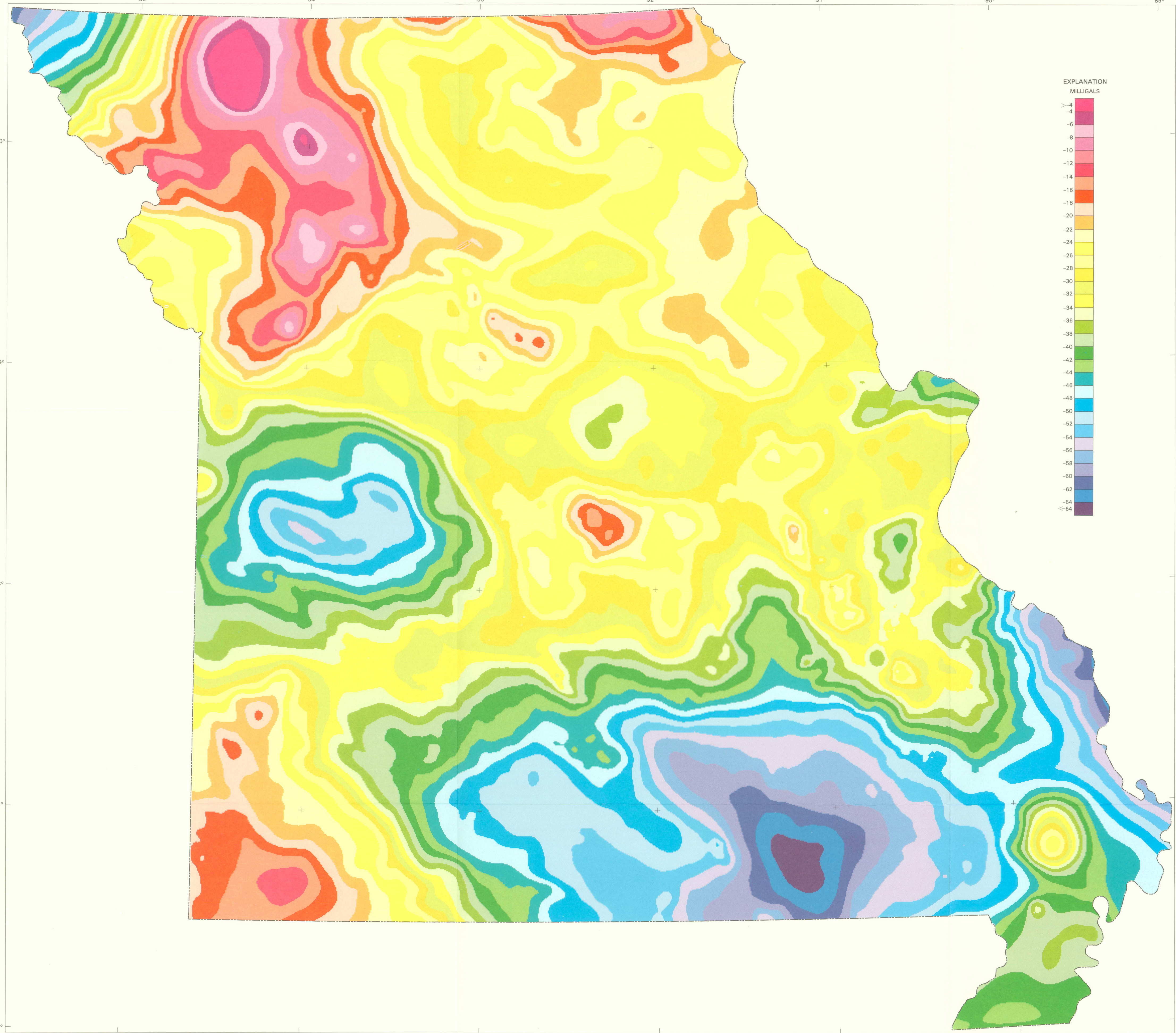
MAP C—PSEUDOGRAVITY FIELD
