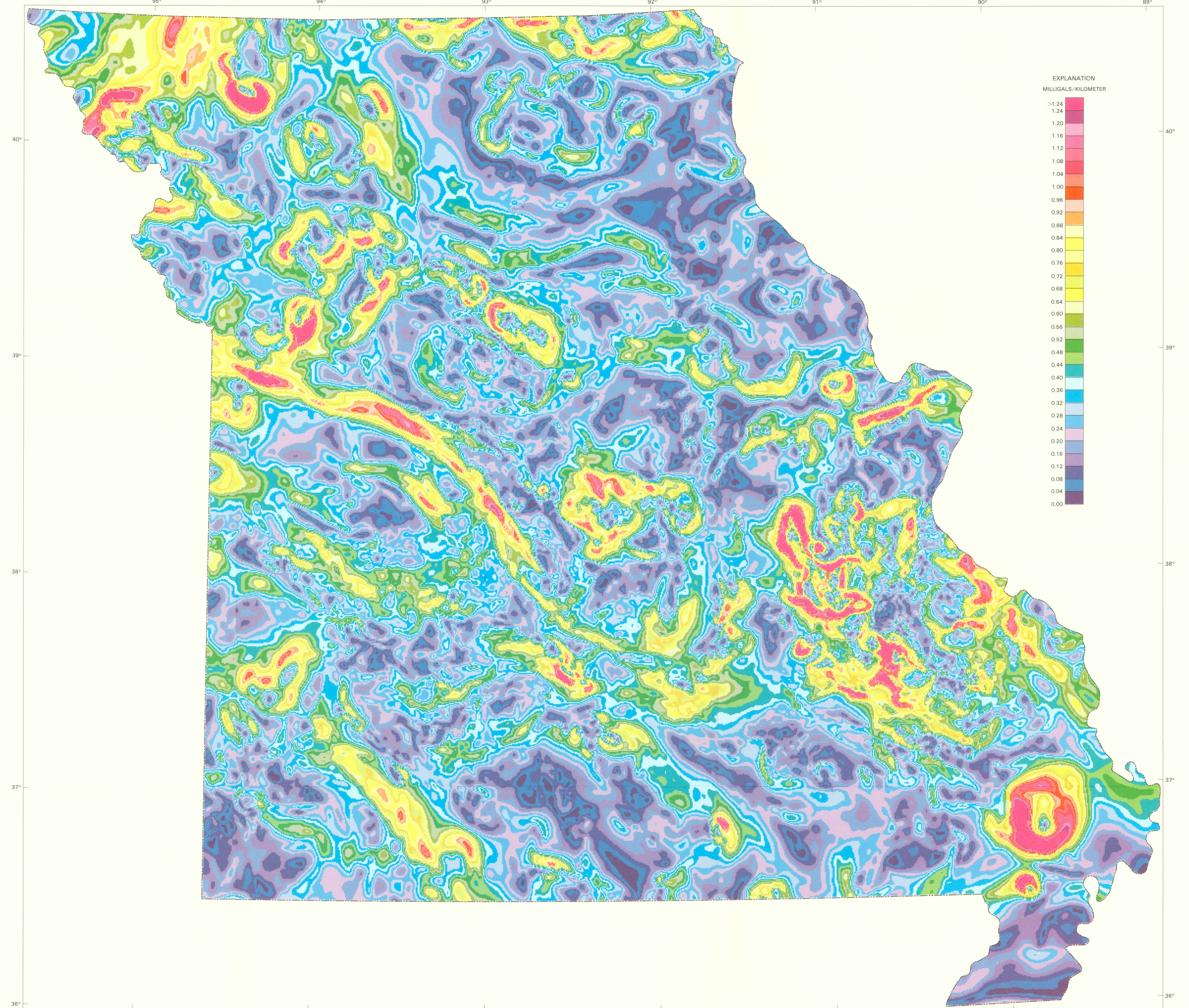
MAP D—MAGNITUDE OF THE HORIZONTAL GRADIENT OF THE PSEUDOGRAVITY FIELD
