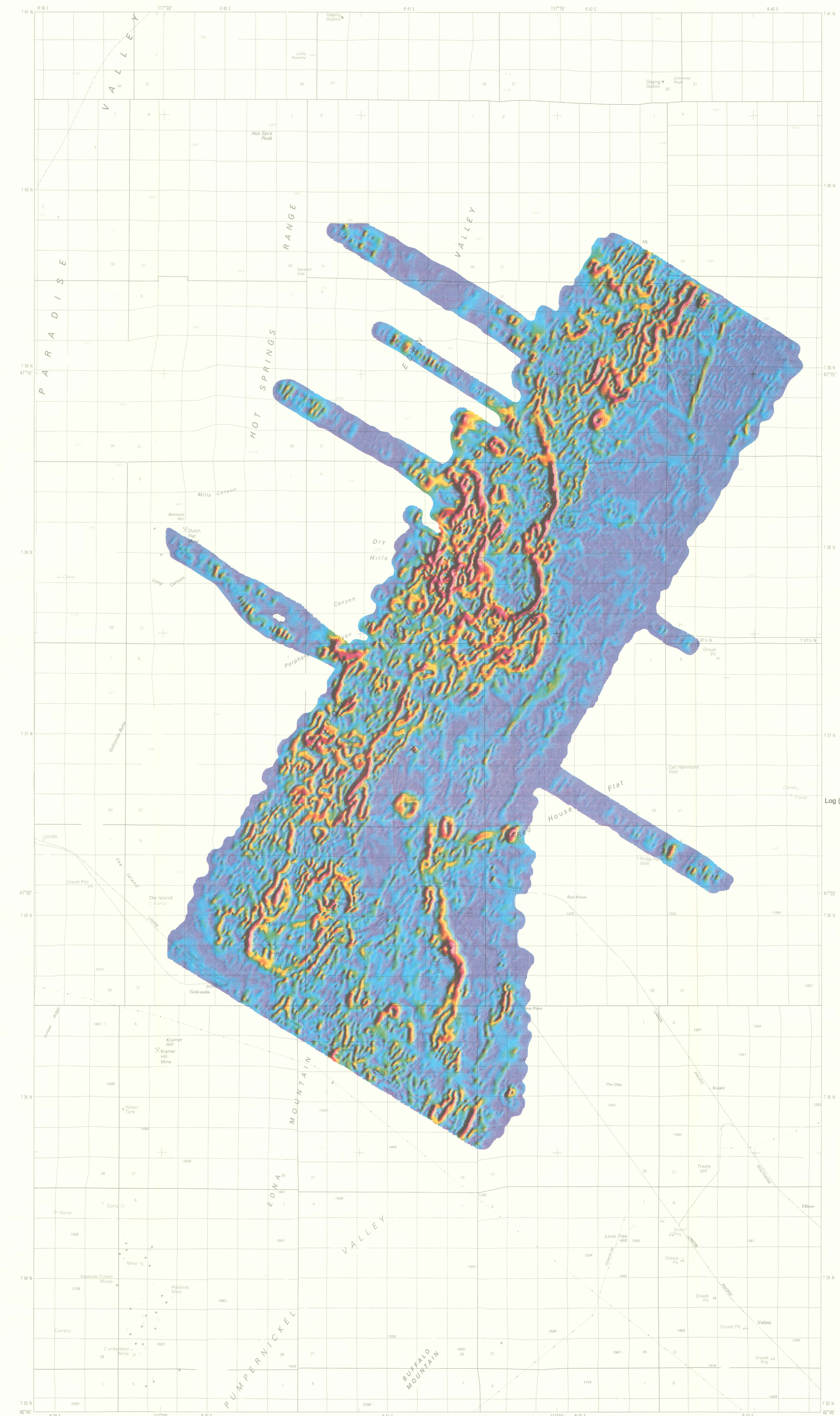
MAP E. HORIZONTAL GRADIENT MAGNITUDE OF 7,200-HERTZ APPARENT RESISTIVITY
