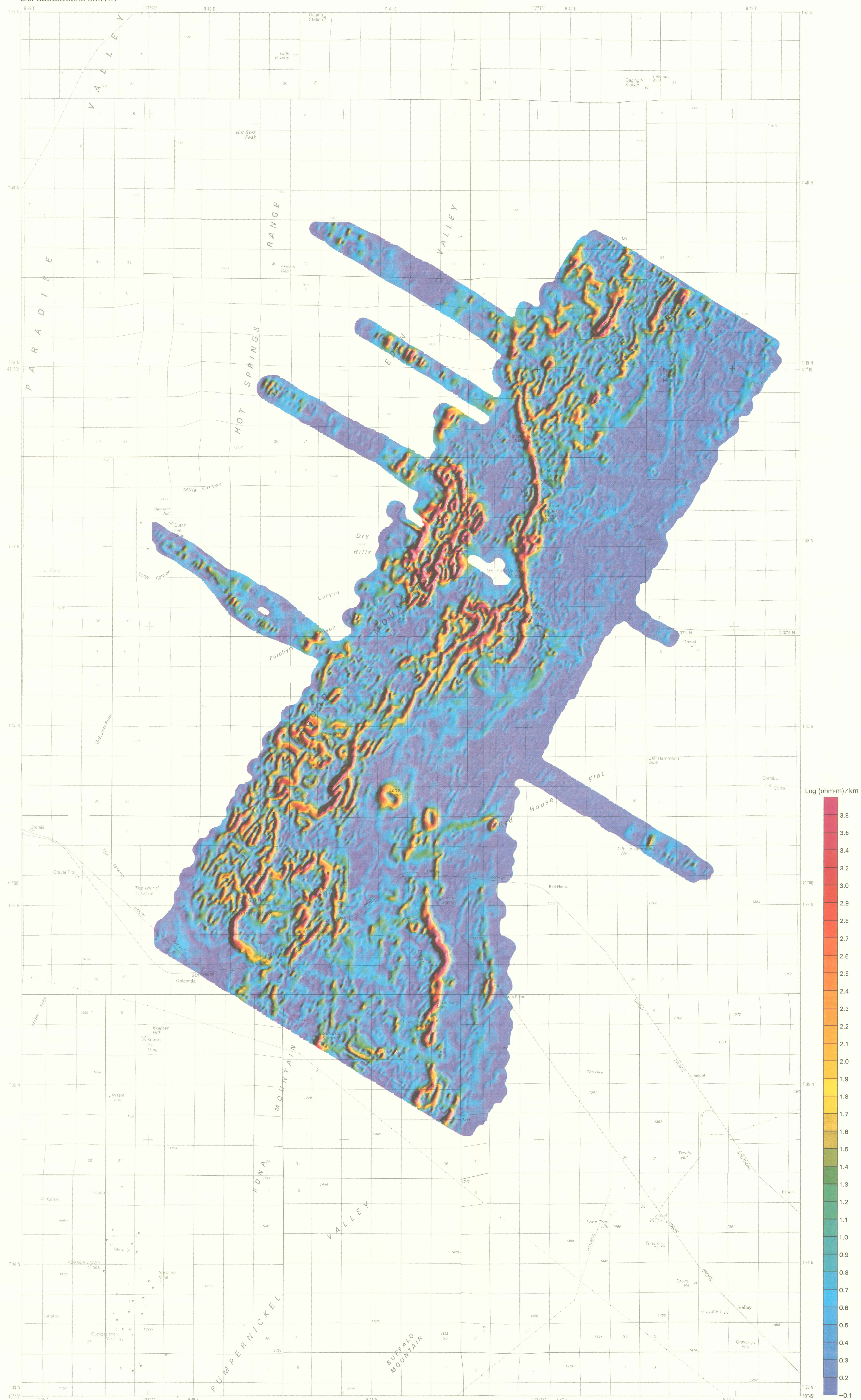
MAP D. HORIZONTAL GRADIENT MAGNITUDE OF 900-HERTZ APPARENT RESISTIVITY
