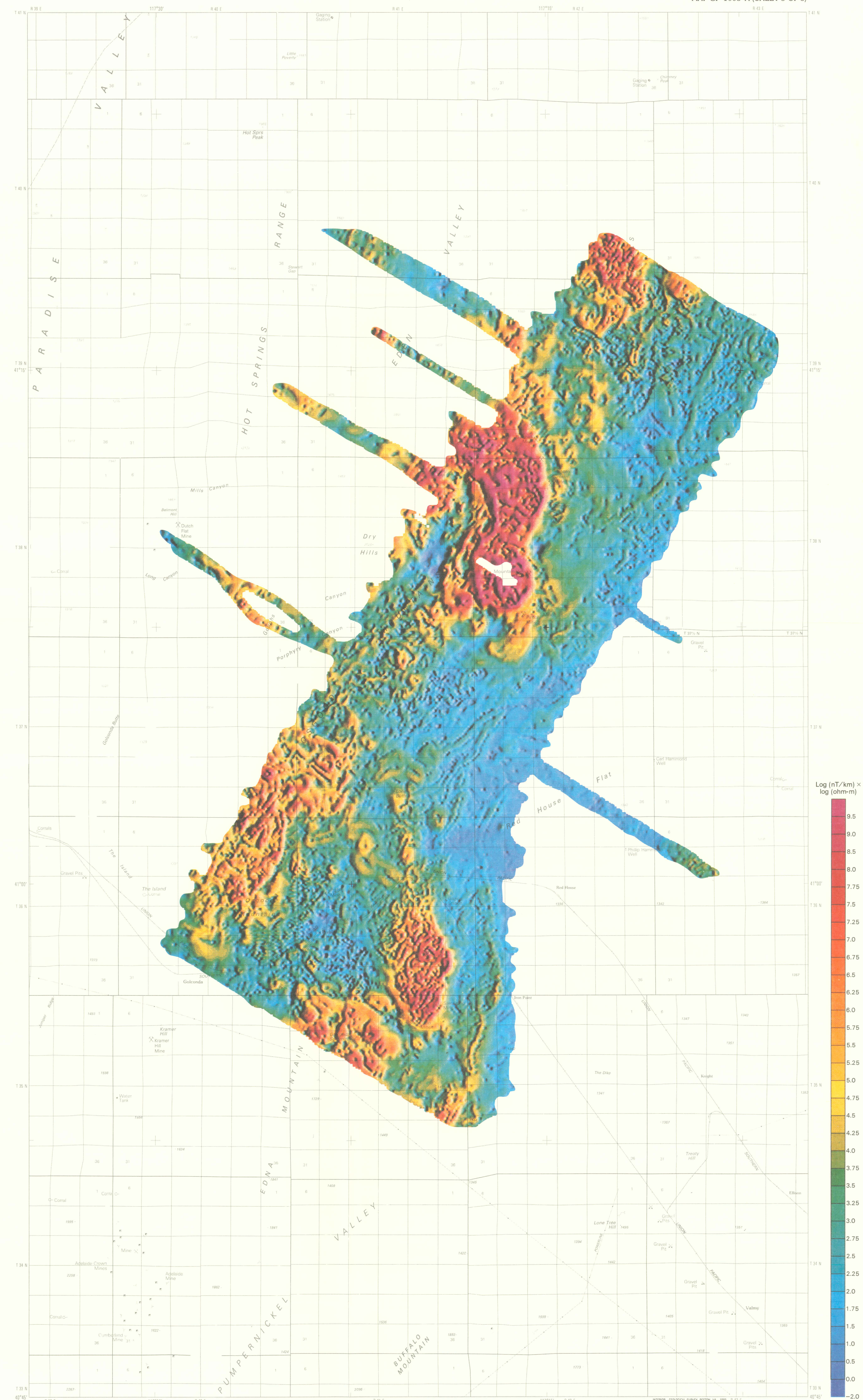
MAP I. LOG HORIZONTAL GRADIENT MAGNITUDE OF REDUCED-TO-THE-POLE MAGNETICS MULTIPLIED BY LOG 900-HERTZ APPARENT RESISTIVITY
