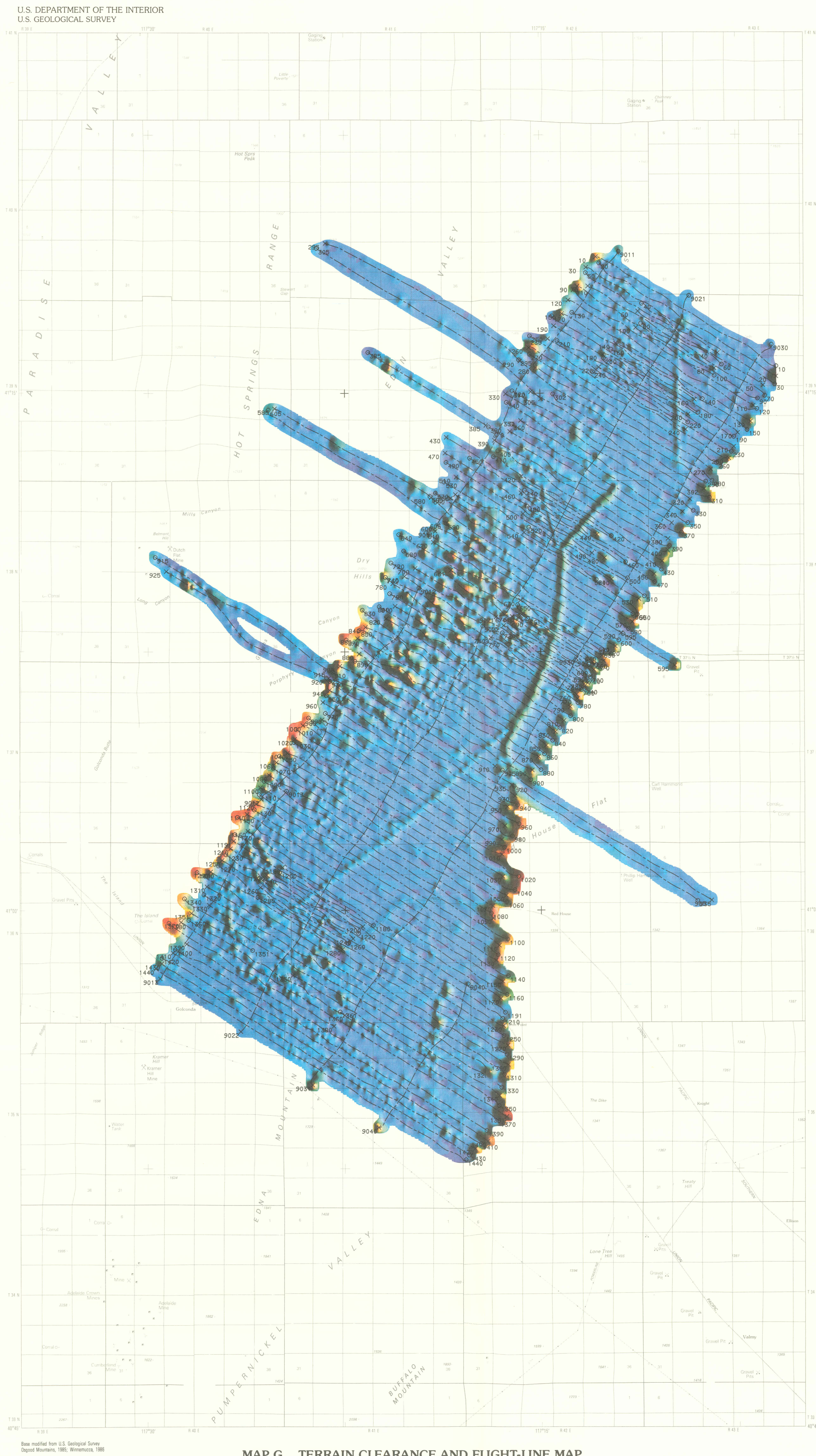
MAP G. TERRAIN CLEARANCE AND FLIGHT-LINE MAP
