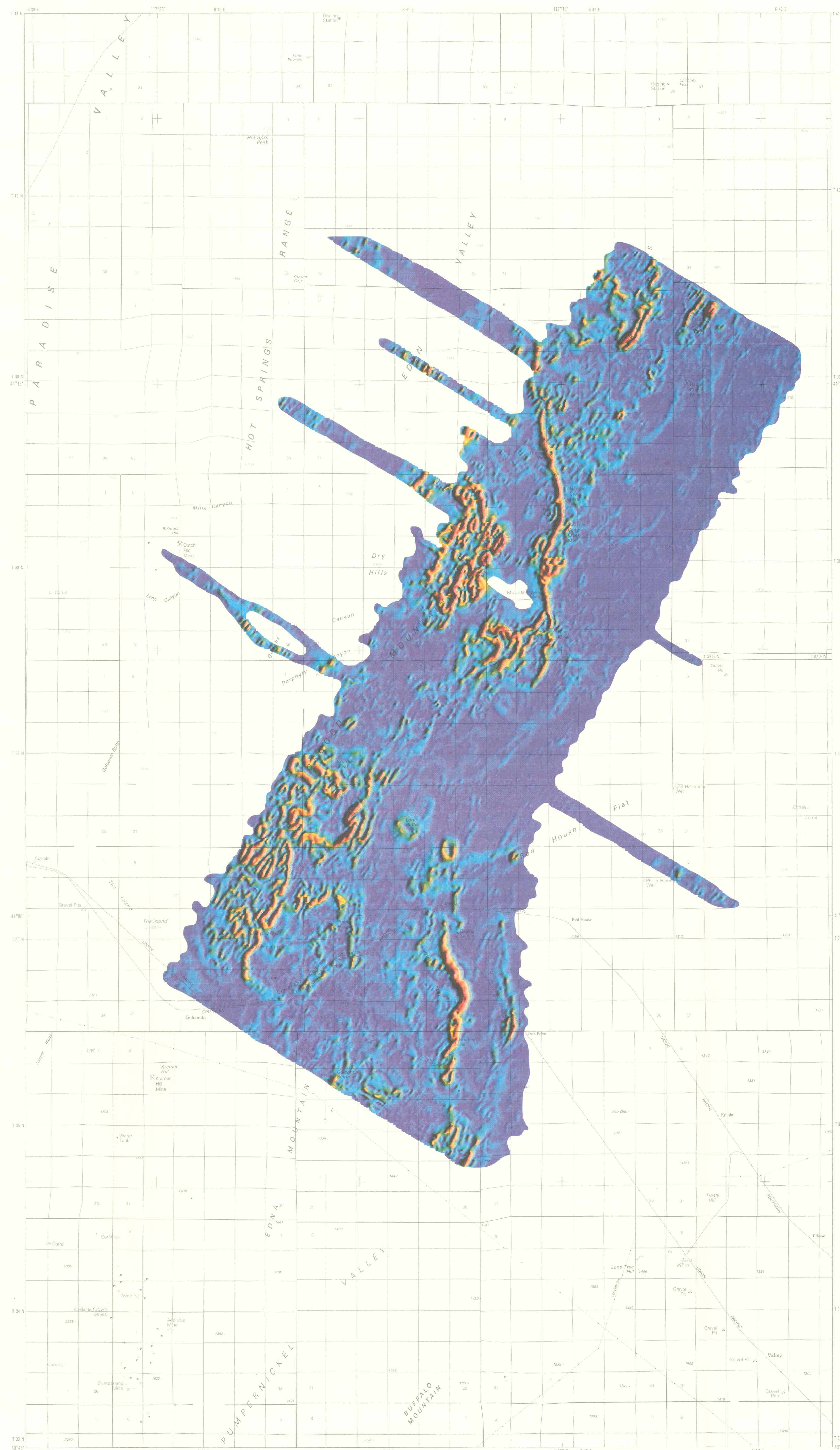
MAP H. LOG HORIZONTAL GRADIENT MAGNITUDE OF REDUCED-TO-THE-POLE MAGNETICS MULTIPLIED BY HORIZONTAL GRADIENT MAGNITUDE OF LOG 900-HERTZ APPARENT RESISTIVITY
