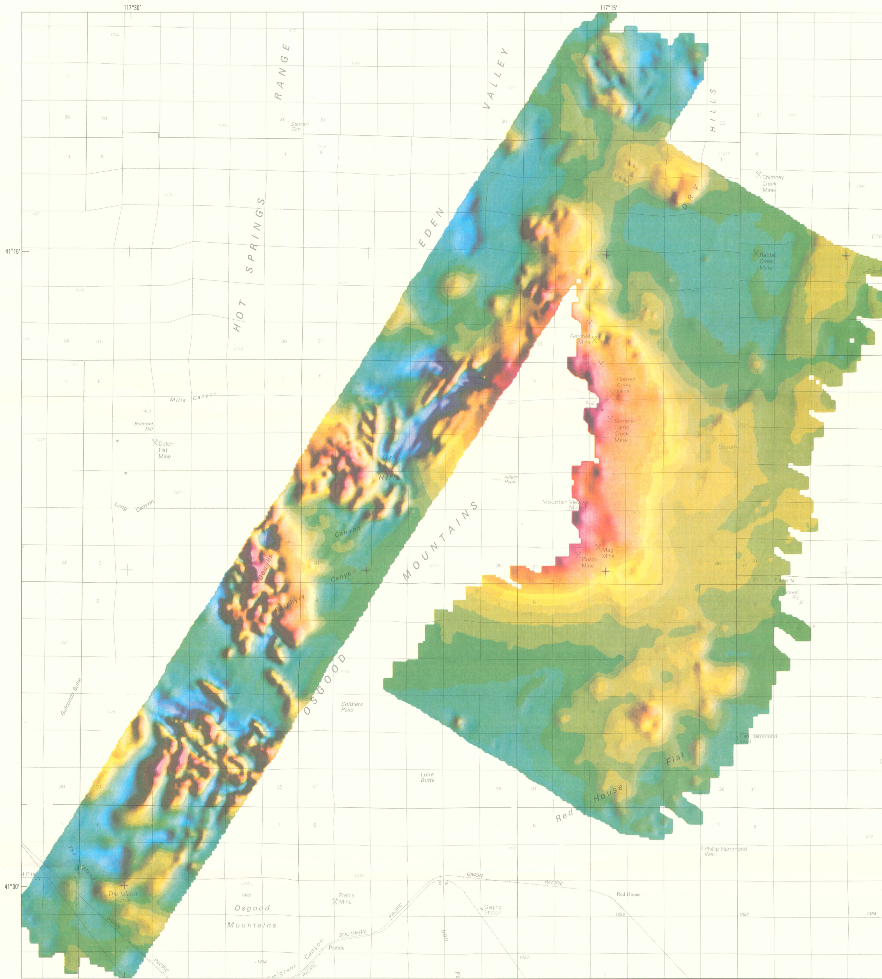
MAP K. REDUCED-TO-POLE MAGNETIC MAP, IN-HOUSE SURVEY
