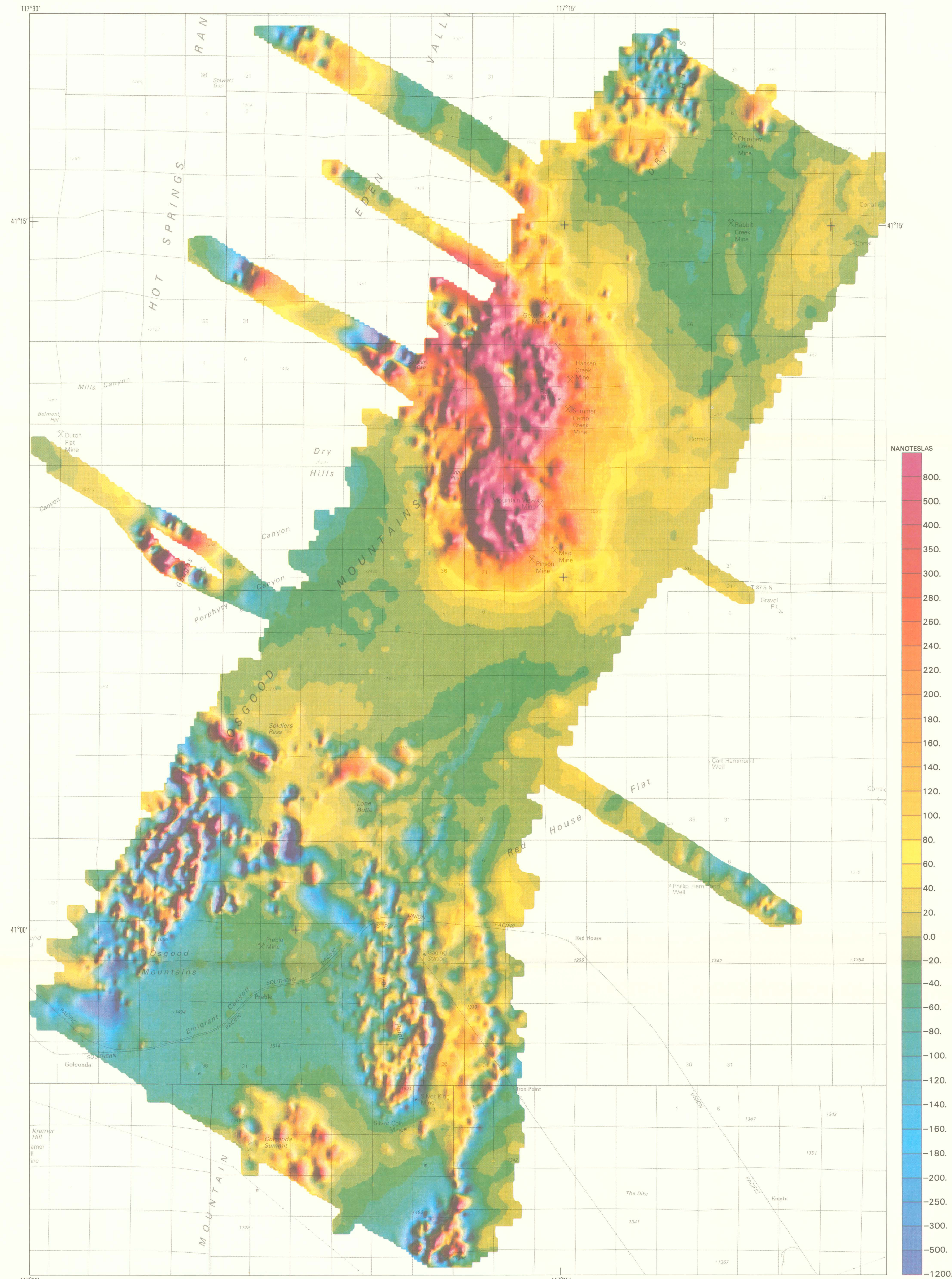
MAP J. REDUCED-TO-POLE MAGNETIC MAP, CONTRACT SURVEY
