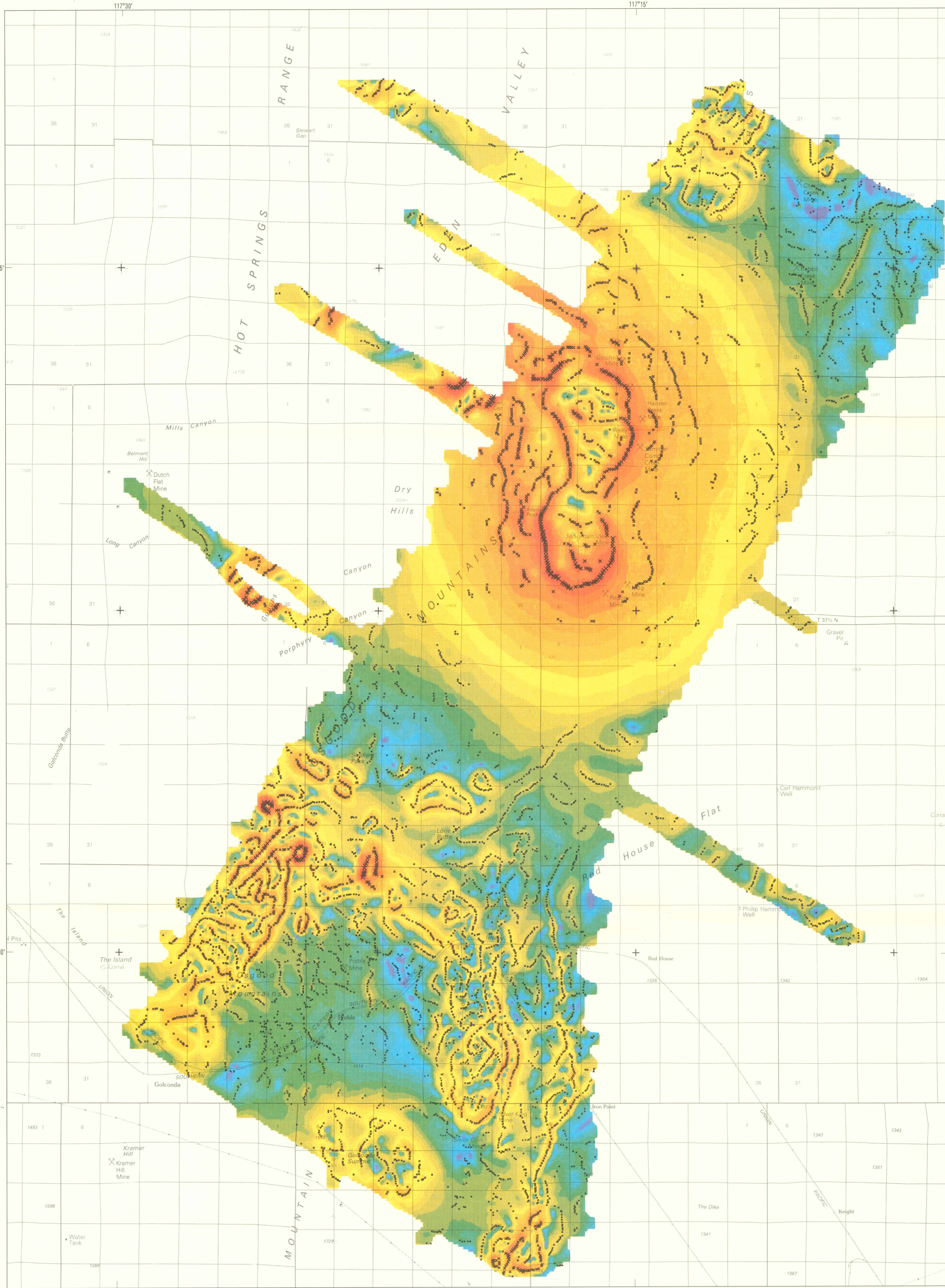
MAP M. MAP SHOWING LOG OF HORIZONTAL-GRADIENT MAGNITUDE OF PSEUDOGRAVITY (COLOR) AND LOCATIONS OF LOCAL MAXIMA (X'S), CONTRACT SURVEY
