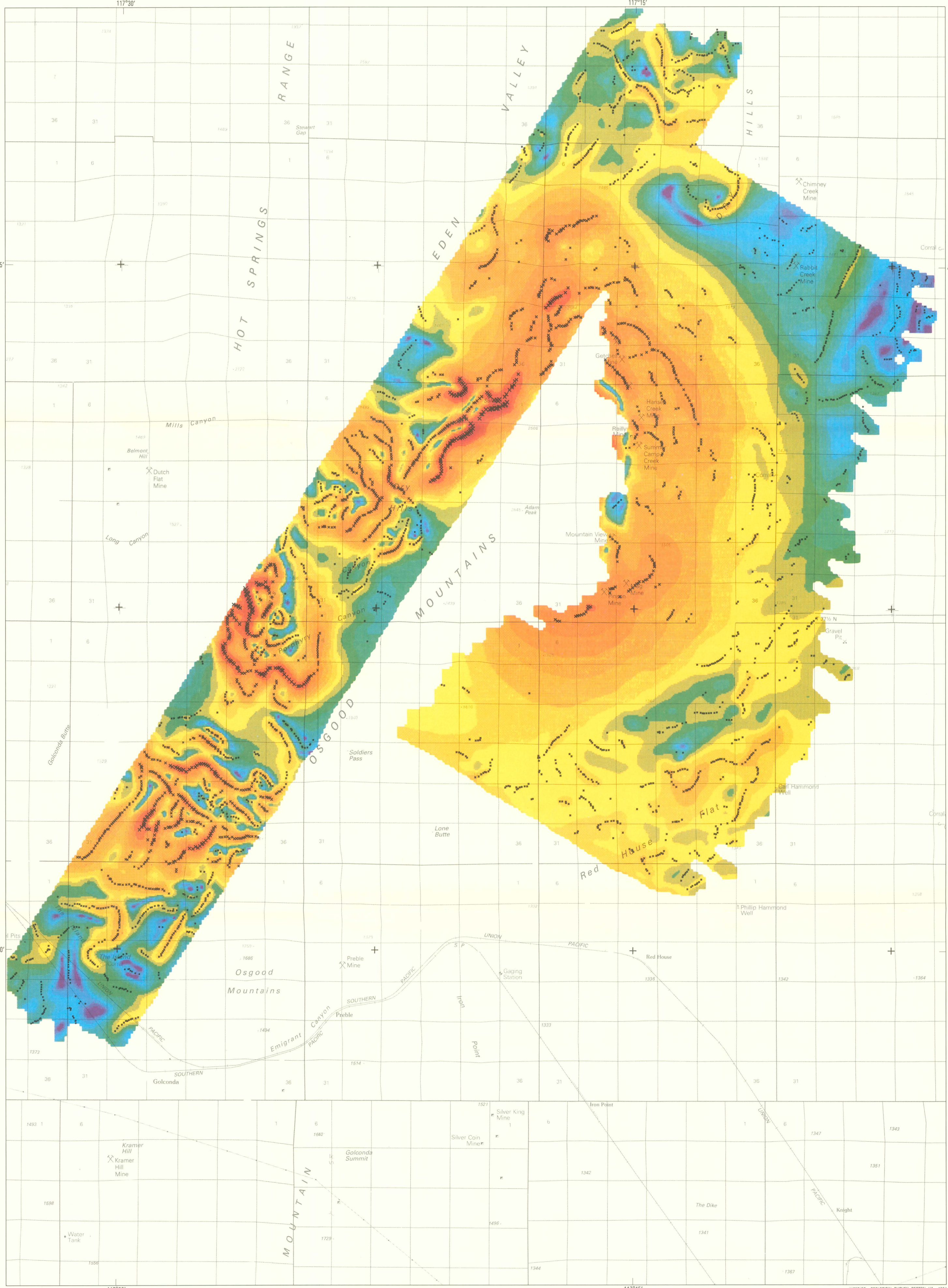
MAP N. MAP SHOWING LOG OF HORIZONTAL-GRADIENT MAGNITUDE OF PSEUDOGRAVITY (COLOR) AND LOCATIONS OF LOCAL MAXIMA (X'S), IN-HOUSE SURVEY
