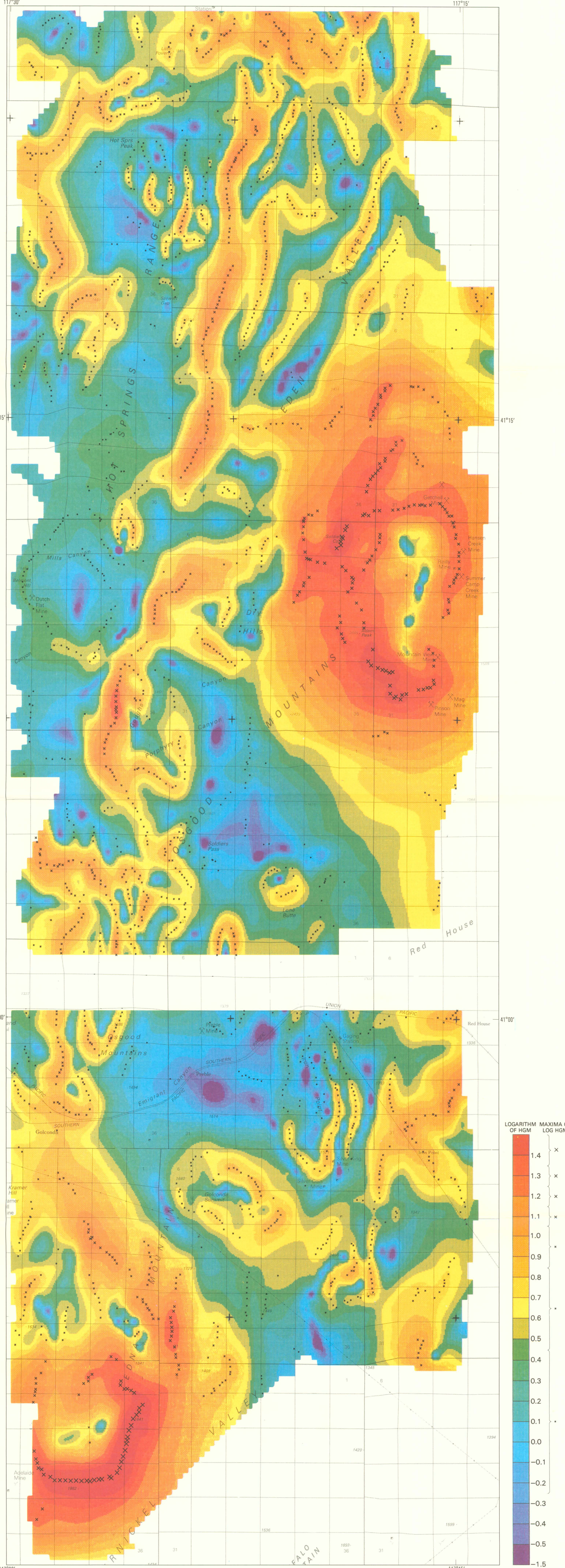
MAP O. MAP SHOWING LOG OF HORIZONTAL-GRADIENT MAGNITUDE OF PSEUDOGRAVITY (COLOR) AND LOCATIONS OF LOCAL MAXIMA (X'S), IRON POINT SURVEY
