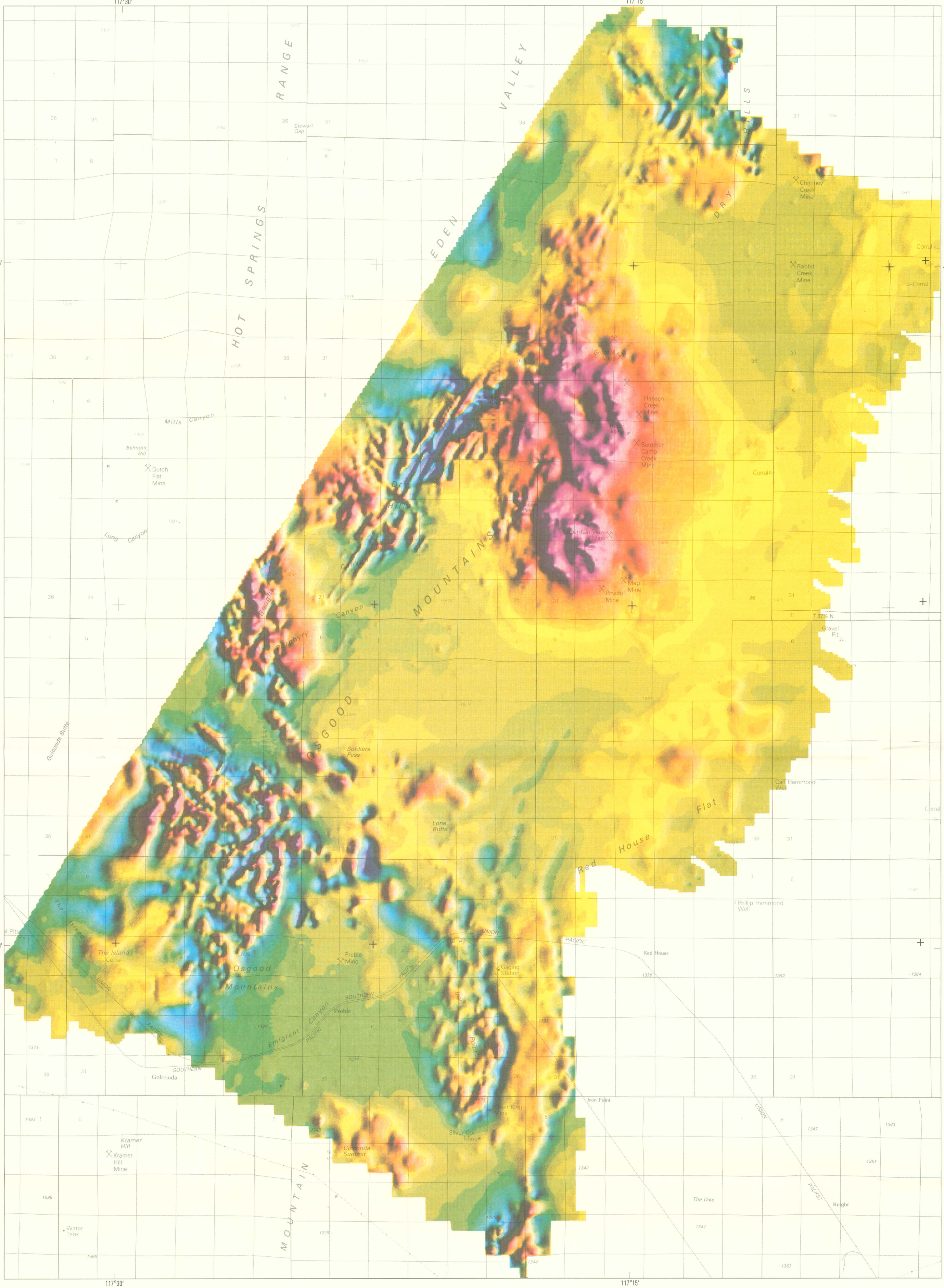
MAP Q. MAP SHOWING REDUCED-TO-POLE MERGED MAGNETIC DATA
