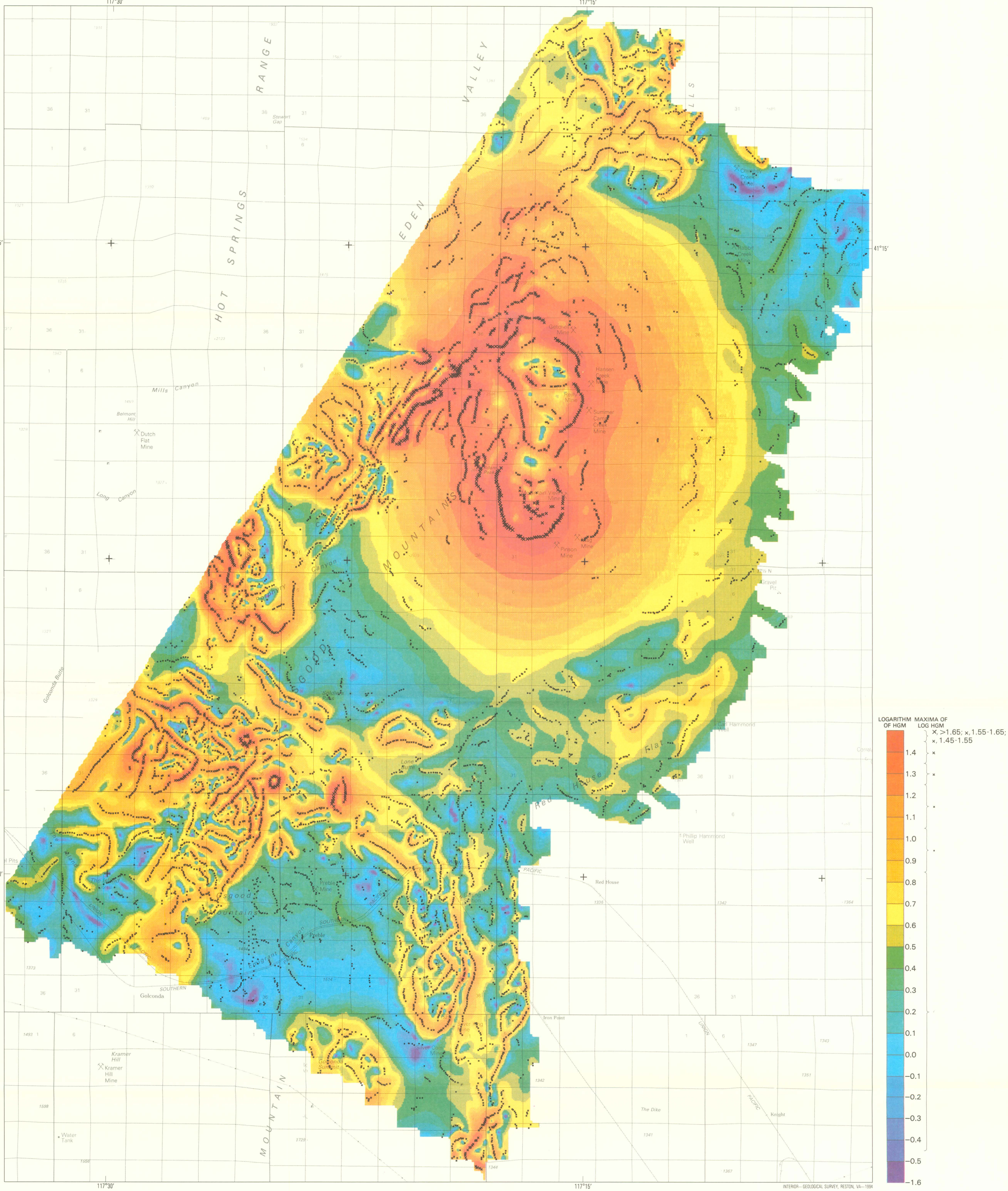
MAP R. MAP SHOWING LOG OF HORIZONTAL-GRADIENT MAGNITUDE OF PSEUDOGRAVITY (COLOR) AND LOCATIONS OF LOCAL MAXIMA (X'S), MERGED DATA
