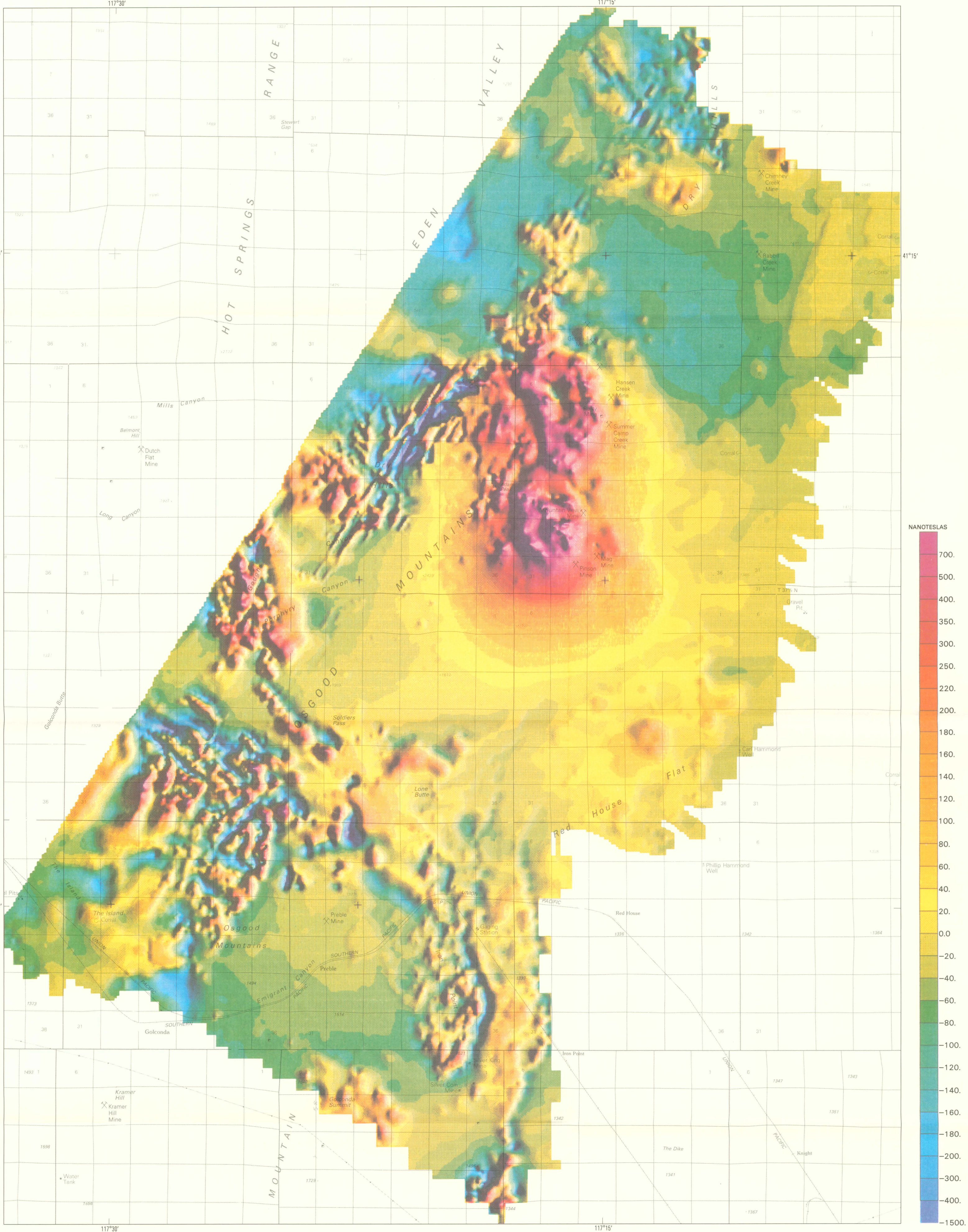
MAP P. MAP SHOWING MERGED CONTRACT AND IN-HOUSE SURVEY MAGNETIC DATA
