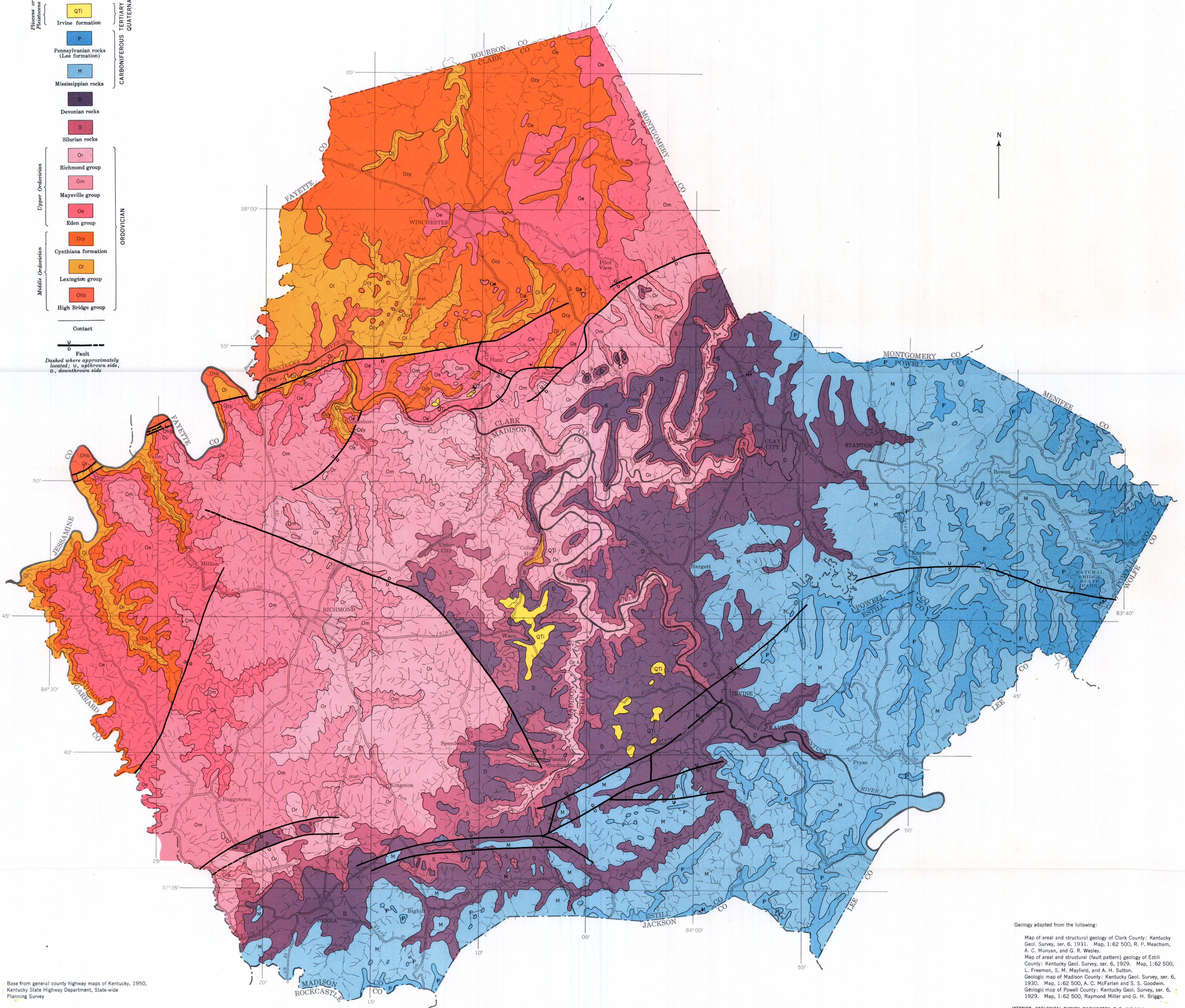
GEOLOGIC MAP OF CLARK, ESTILL, MADISON, AND POWELL COUNTIES, KENTUCKY (COUNTY GROUP 19)
