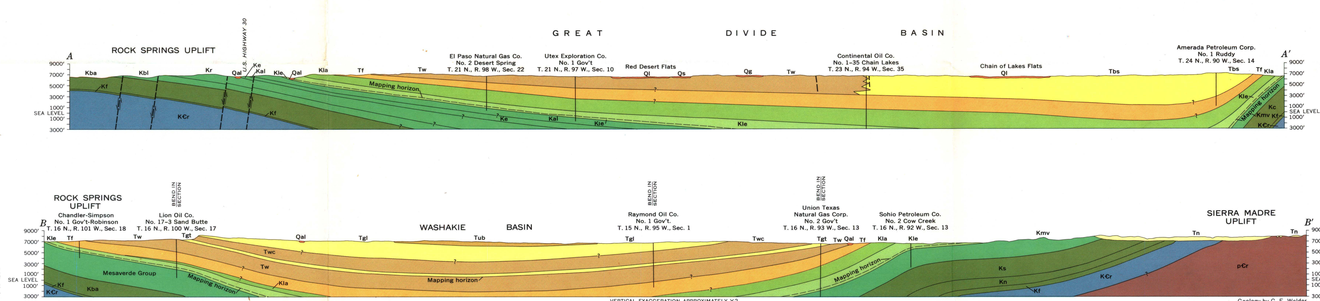
GEOLOGIC MAP SHOWING GENERALIZED STRUCTURE CONTOURS AND GEOLOGIC SECTIONS GROUND-WATER RECONNAISSANCE OF THE GREAT DIVIDE AND WASHAKIE BASINS AND SOME ADJACENT AREAS, SOUTHWESTERN WYOMING By George E. Welder and Laurence J. McGreevy 1966
