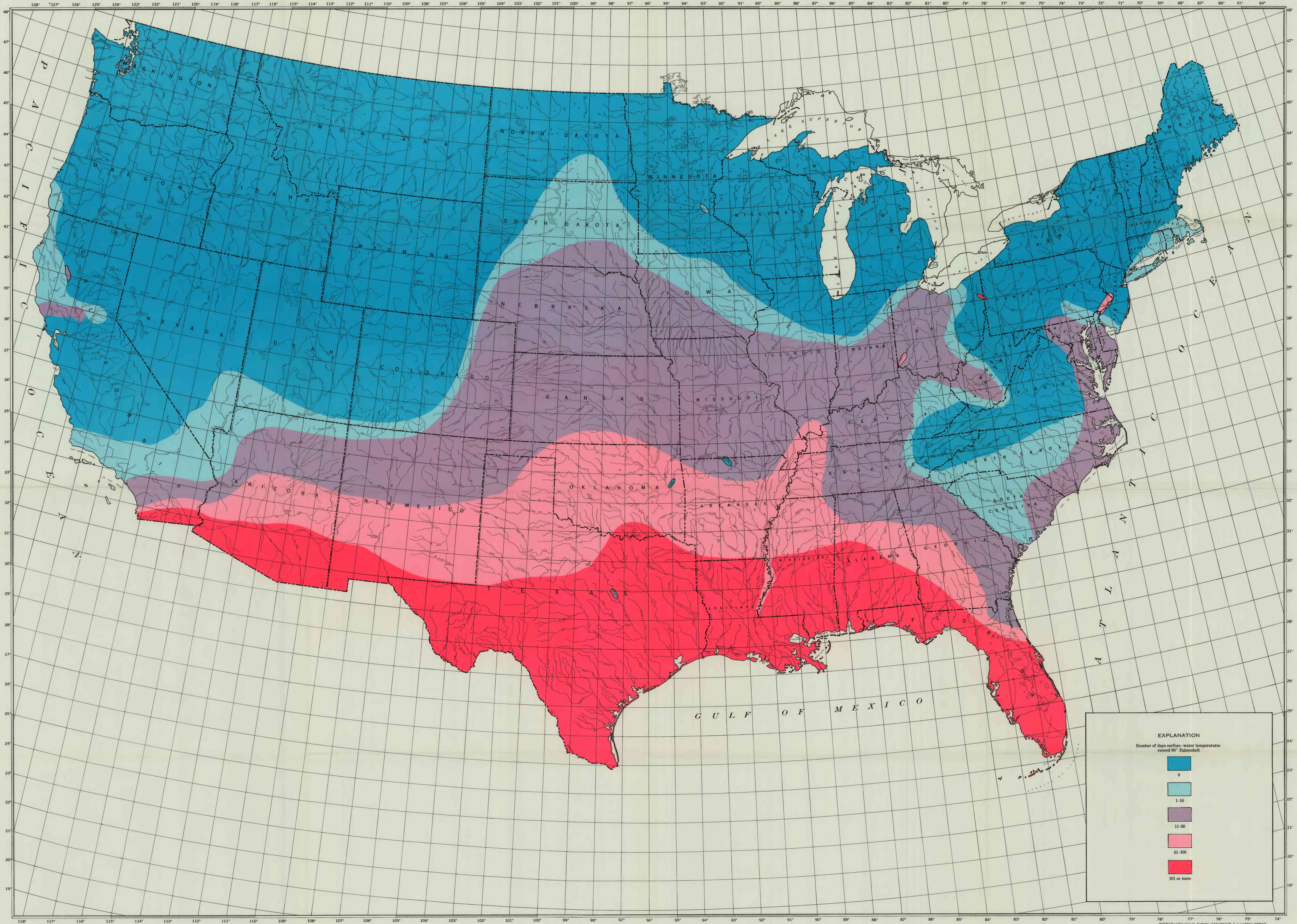
AVERAGE NUMBER OF DAYS PER YEAR WHEN SURFACE-WATER TEMPERATURES ARE 80° F OR HIGHER TEMPERATURE OF SURFACE WATERS IN THE CONTERMINOUS UNITED STATES
