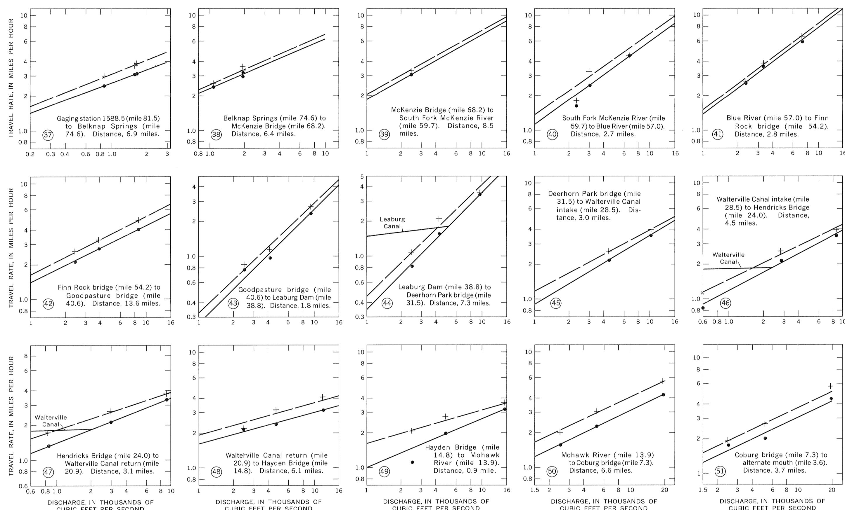
FIGURE 5.—Rate of travel for subreach discharge for McKenzie River.
