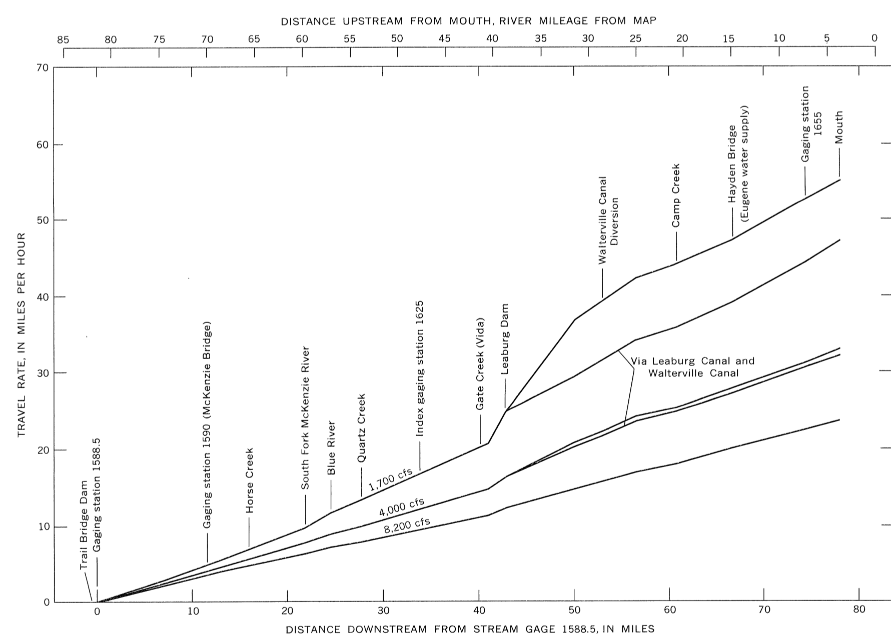
FIGURE 6.—Time of travel of McKenzie River for selected discharges at index gaging station 1825 (near Vida).
