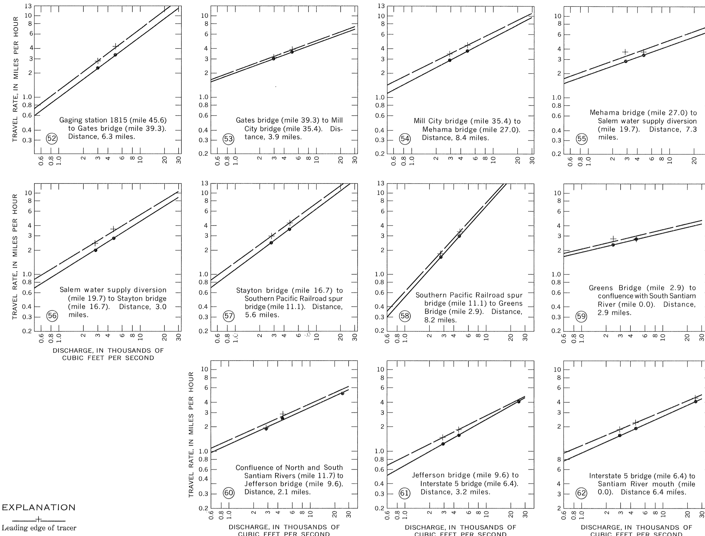
FIGURE 7.—Rate of travel for subreach discharge for North Santiam River (subreaches 52-59) and Santiam River (subreaches 60-62).
