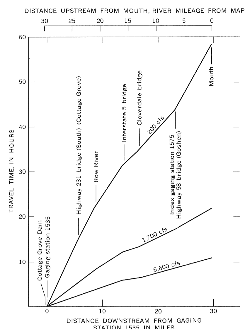
FIGURE 4.—Time of travel of Coast Fork Willamette River for selected discharges at index gaging station 1575 (near Goshen).
