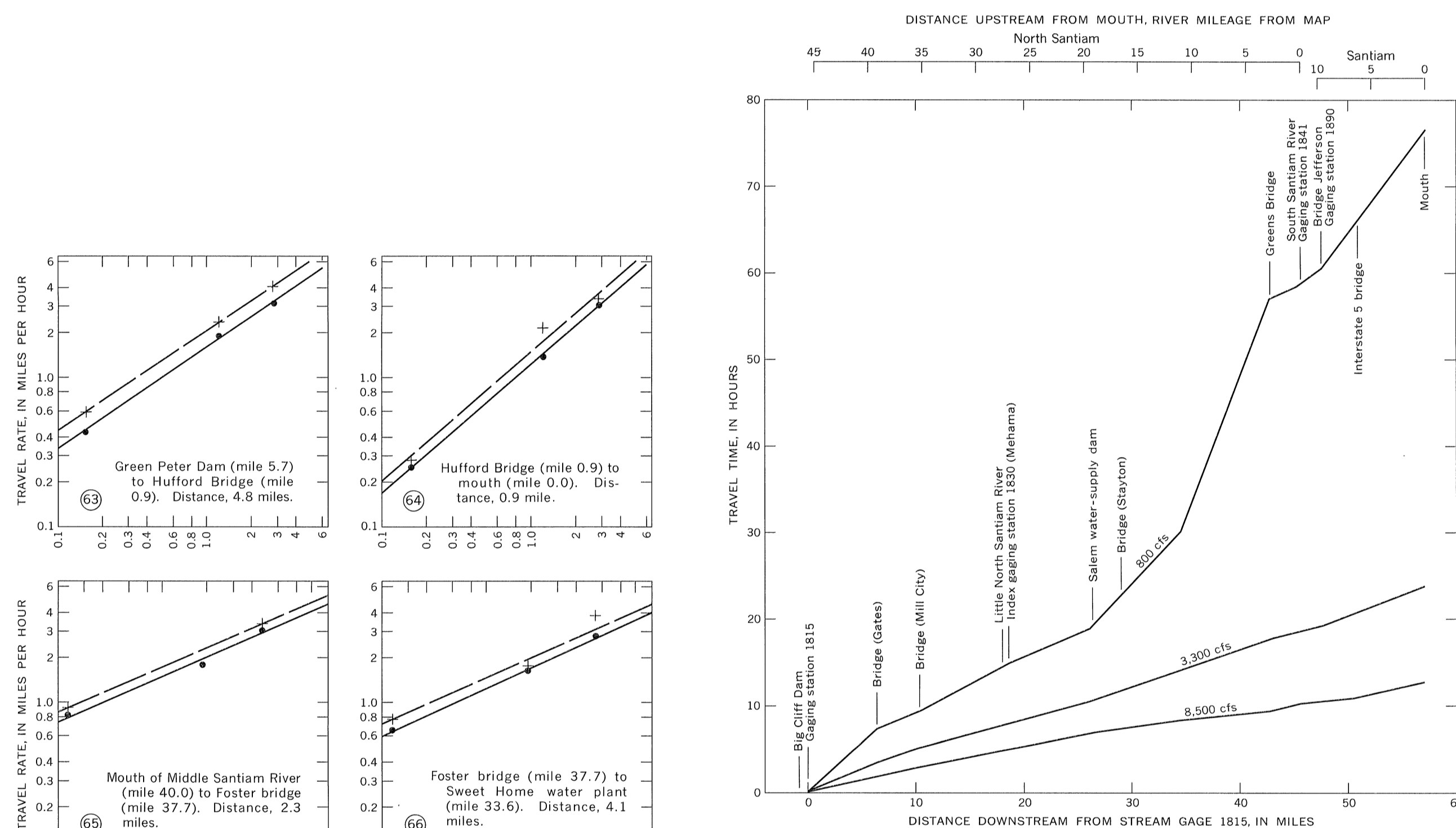
FIGURE 8.—Time of travel of North Santiam and Santiam Rivers for selected discharges at index gaging station 1830 (Mehama).
