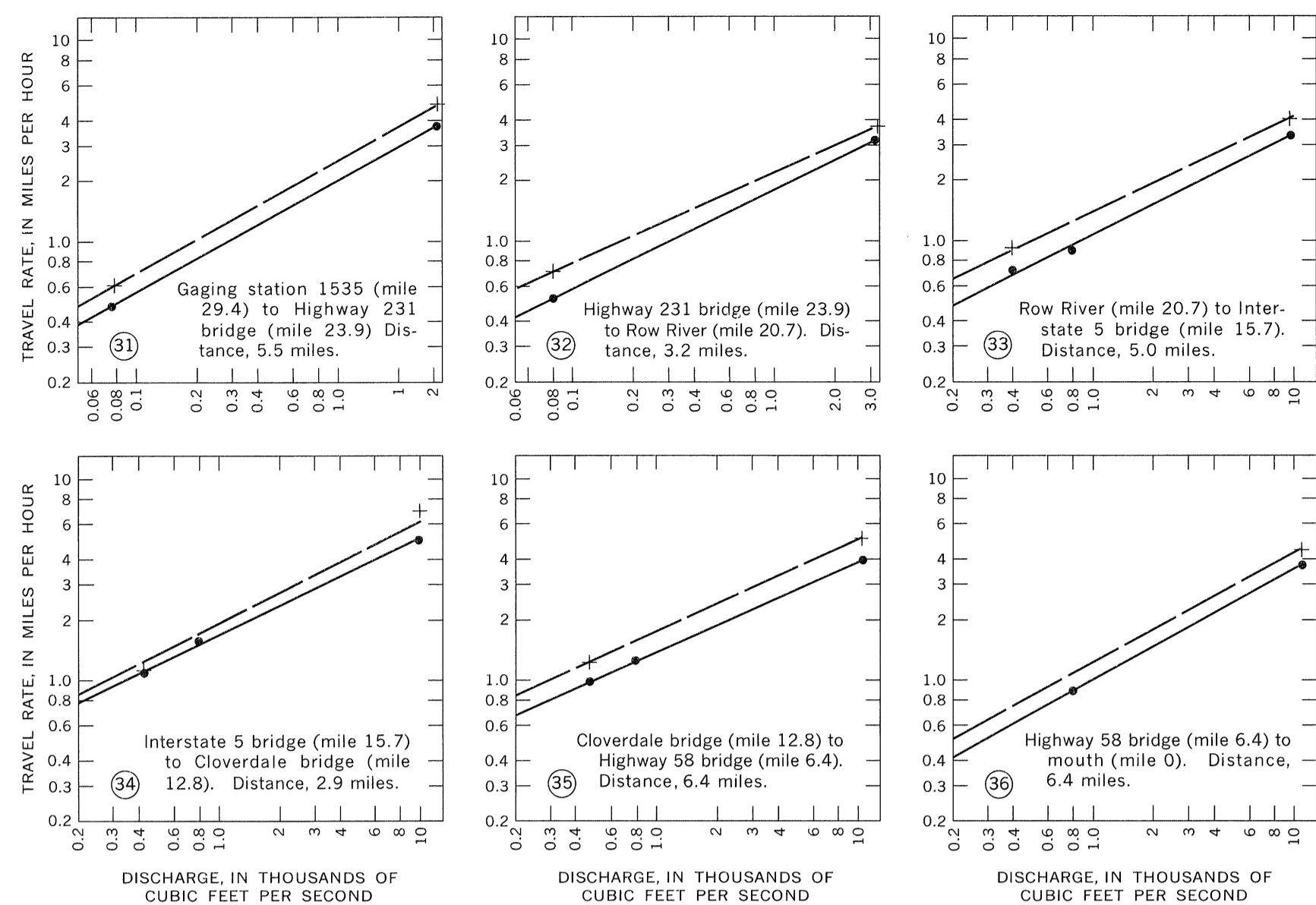
FIGURE 3.—Rate of travel for subreach discharge for Coast Fork Willamette River.
