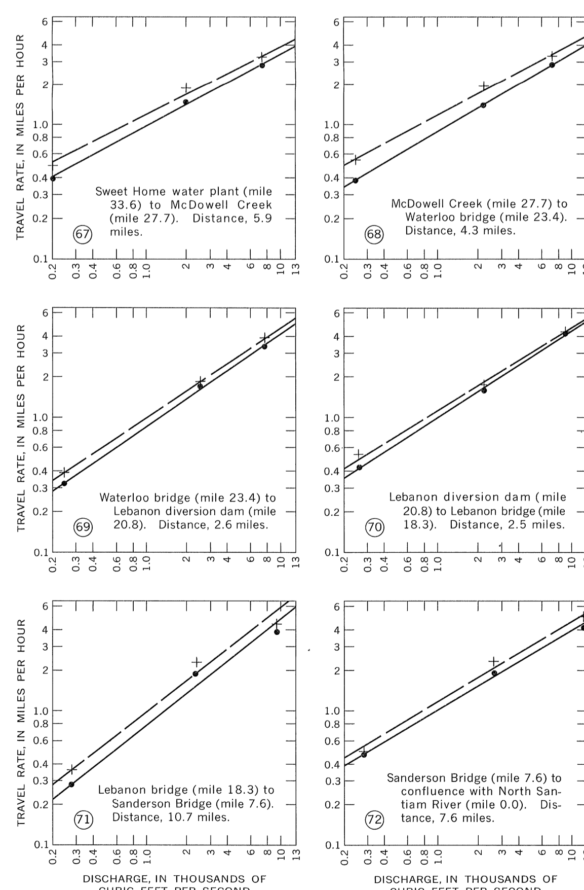
FIGURE 9.—Rate of travel for subreach discharge for Middle Santiam River (subreaches 63 and 64) and South Santiam River (subreaches 65-72).
