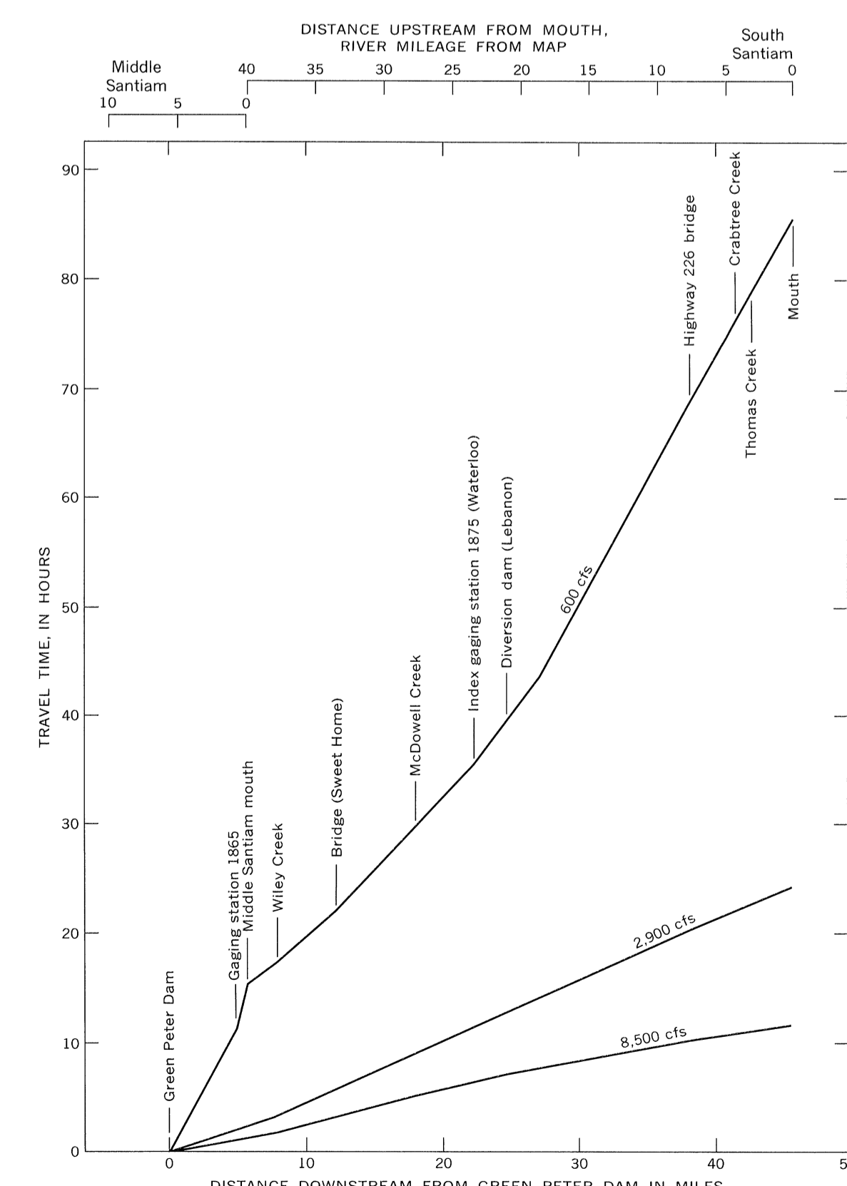
FIGURE 10.—Time of travel of Middle Santiam and South Santiam Rivers for selected discharges at index gaging station 1875 (Waterloo).
