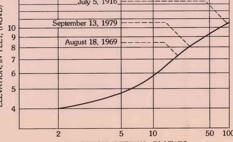
FIGURE 4—Frequency of high tides at Mobile gage (Mobile River at Alabama State Docks)
