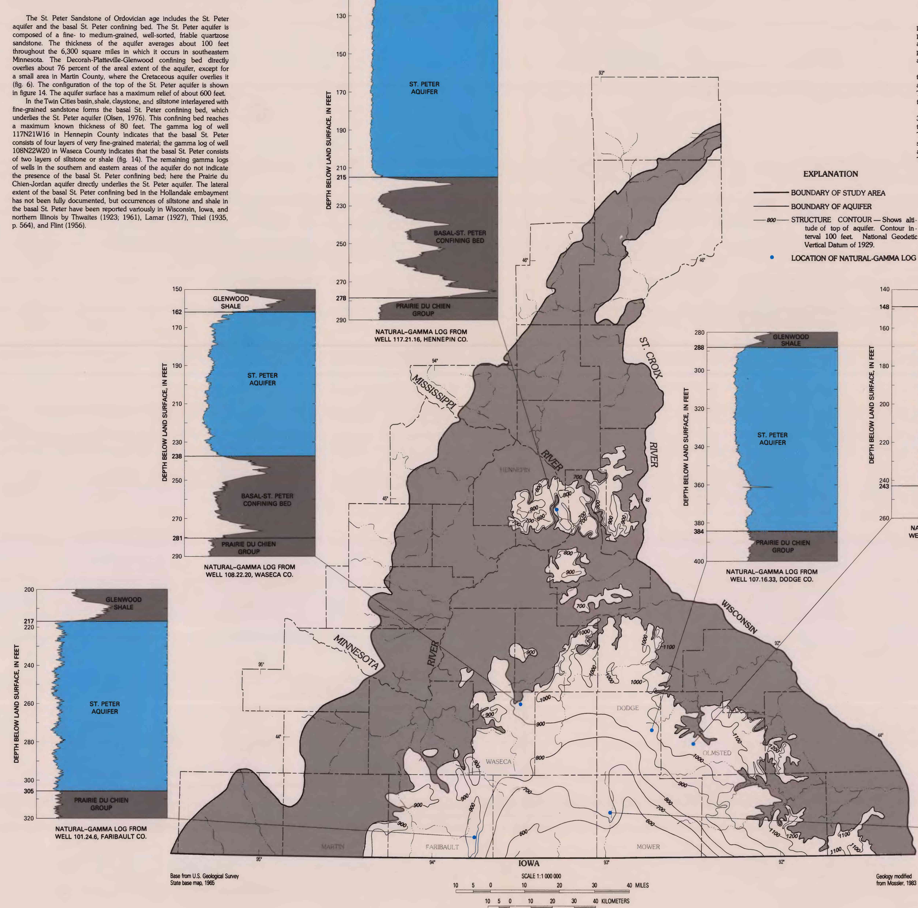
FIGURE 14.—CONFIGURATION OF TOP OF ST. PETER AQUIFER
