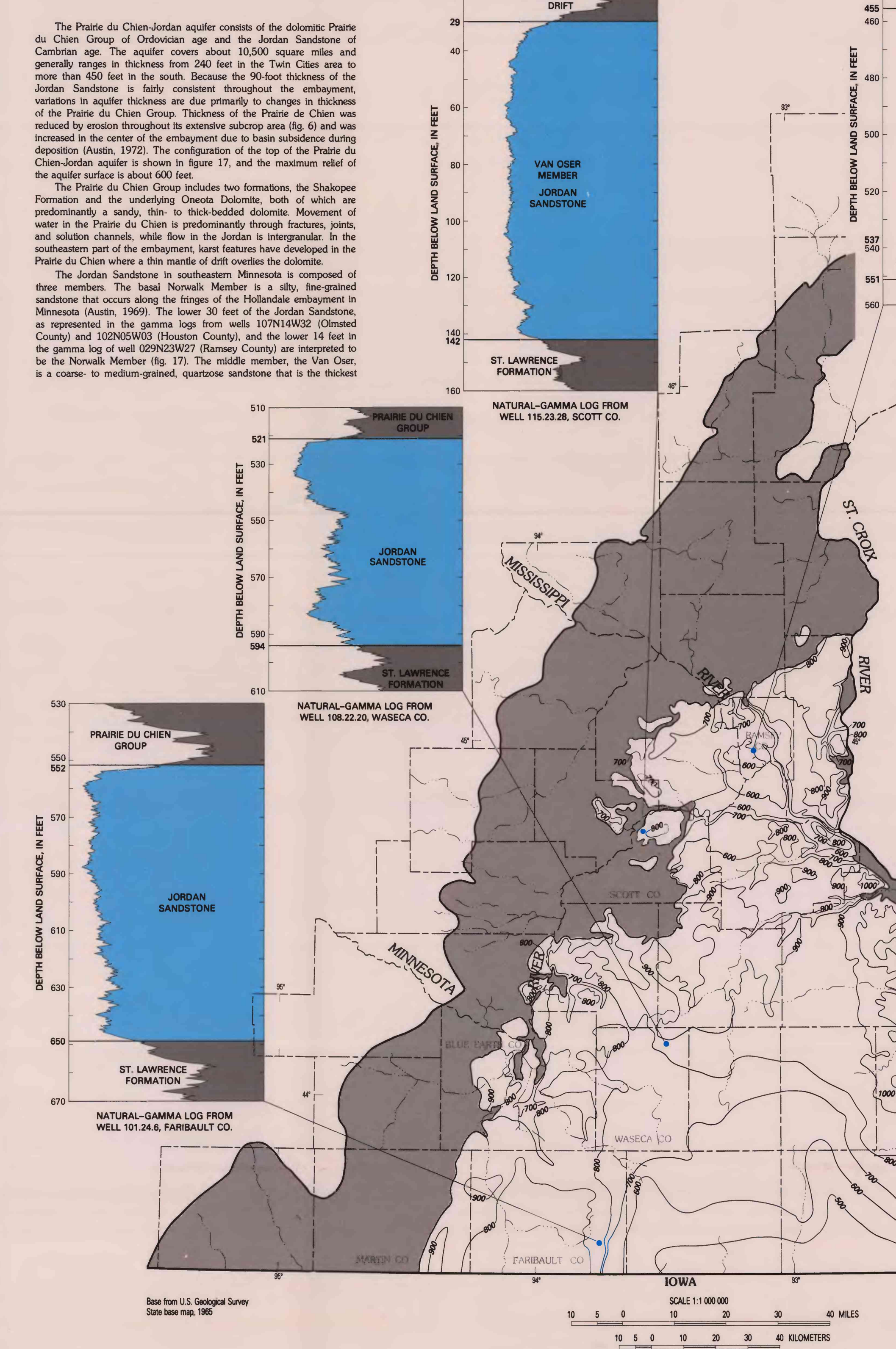
FIGURE 17.—CONFIGURATION OF TOP OF PRAIRIE DU CHIEN-JORDAN AQUIFER
