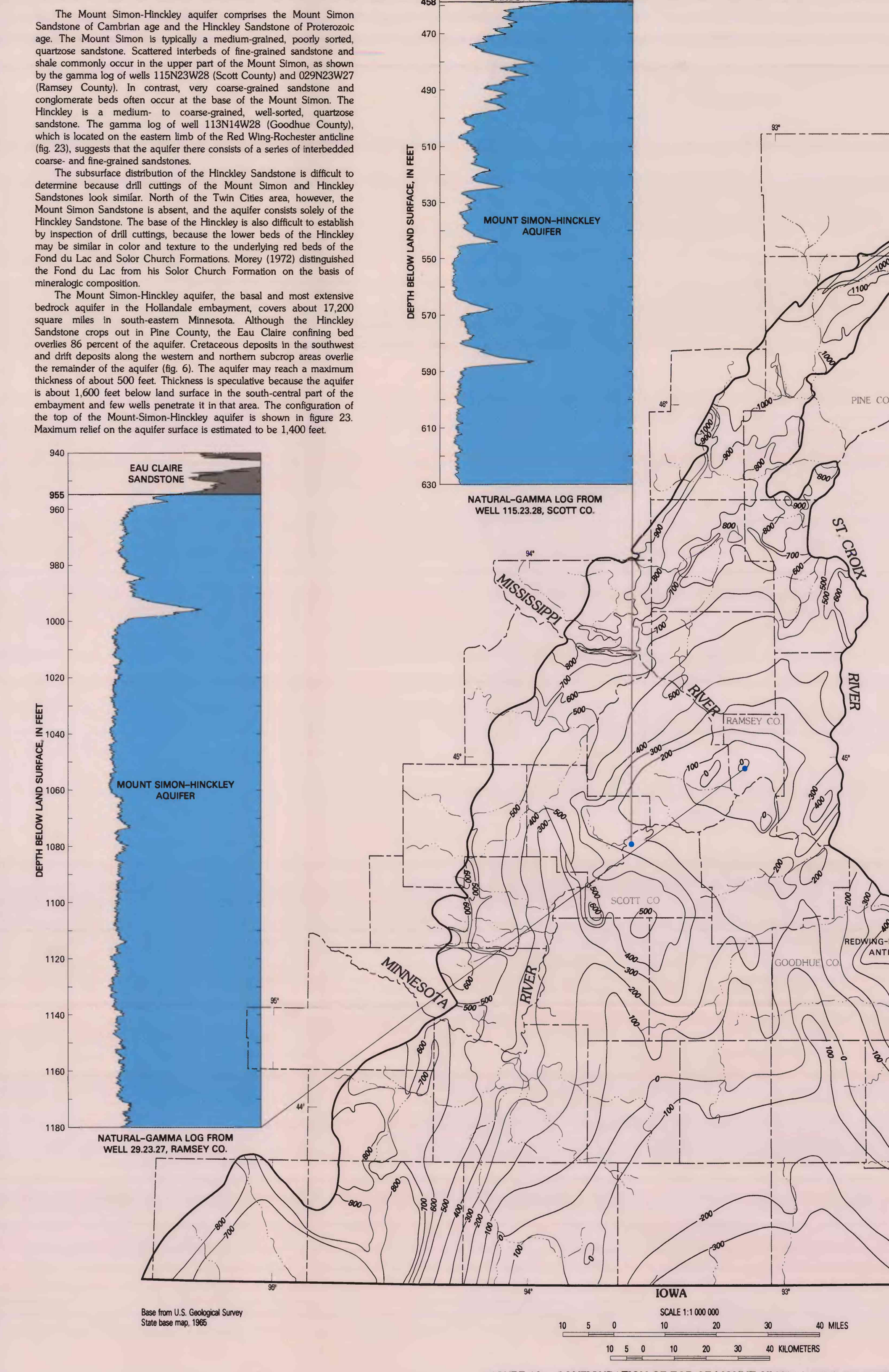
FIGURE 23.—CONFIGURATION OF TOP OF MOUNT SIMON-HINCKLEY AQUIFER
