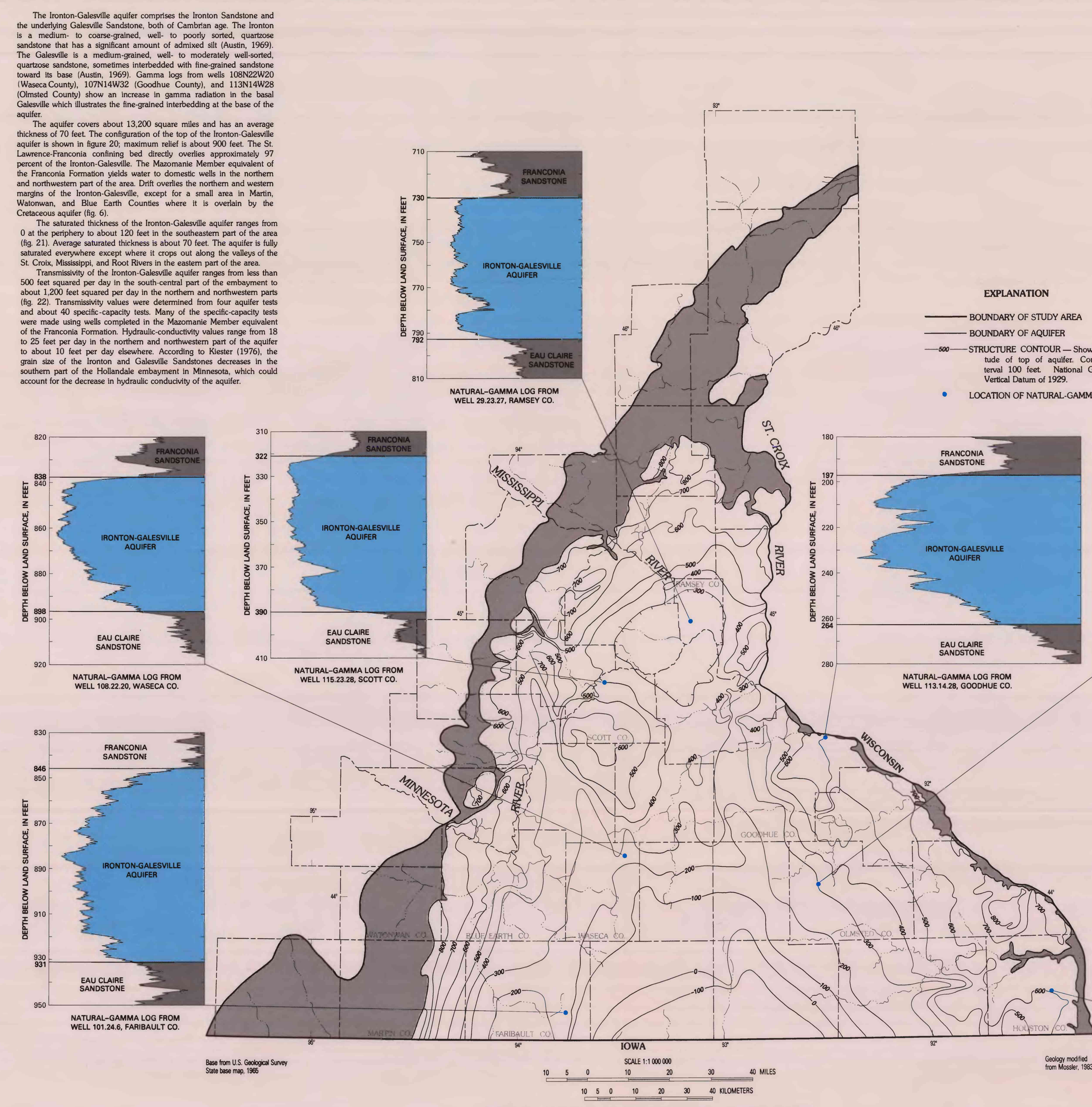
FIGURE 20.—CONFIGURATION OF TOP OF IRONTON-GALESVILLE AQUIFER
