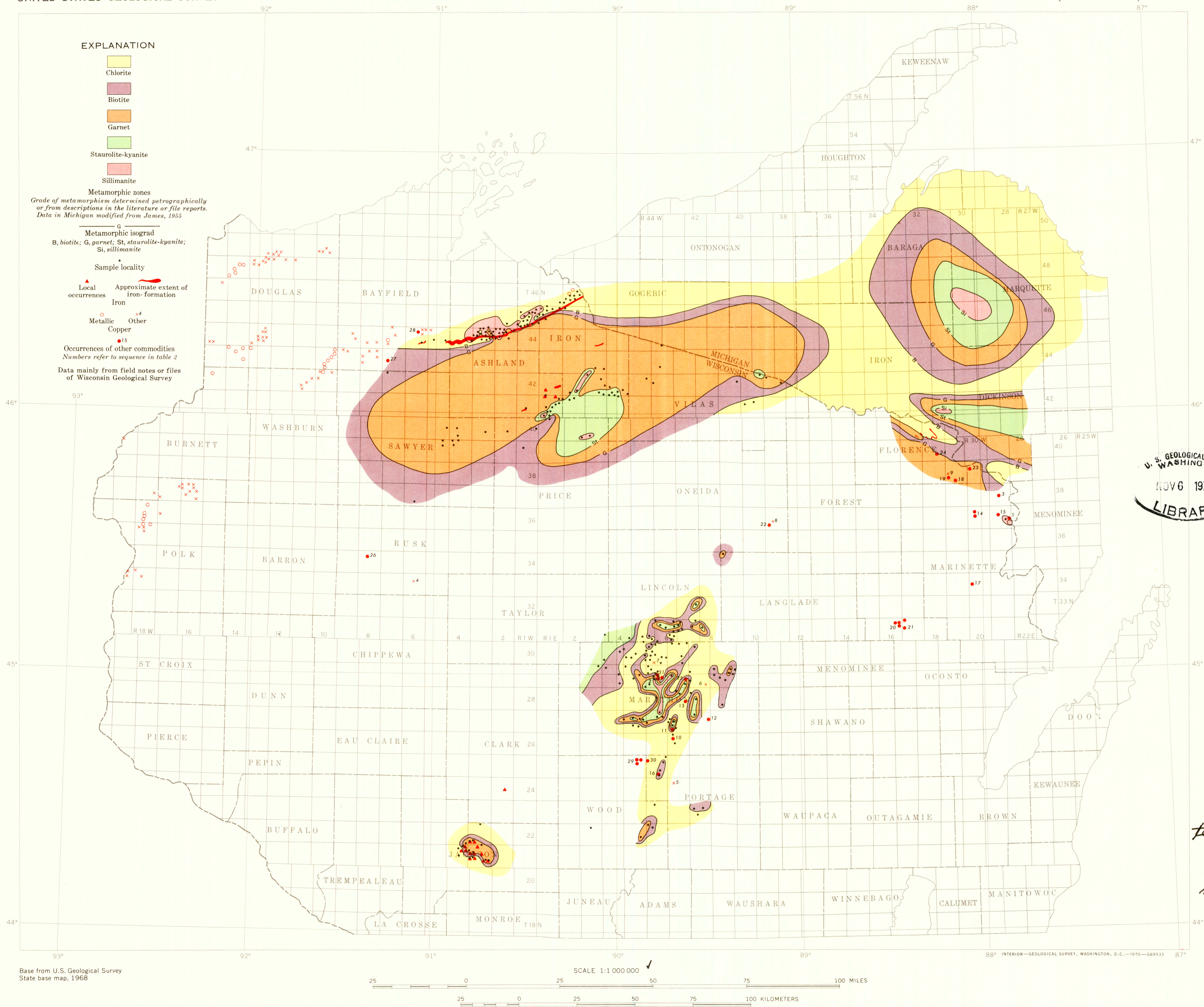
Map of northern Wisconsin and part of Michigan showing mineral commodity localities (Wisconsin only) and metamorphic zones
