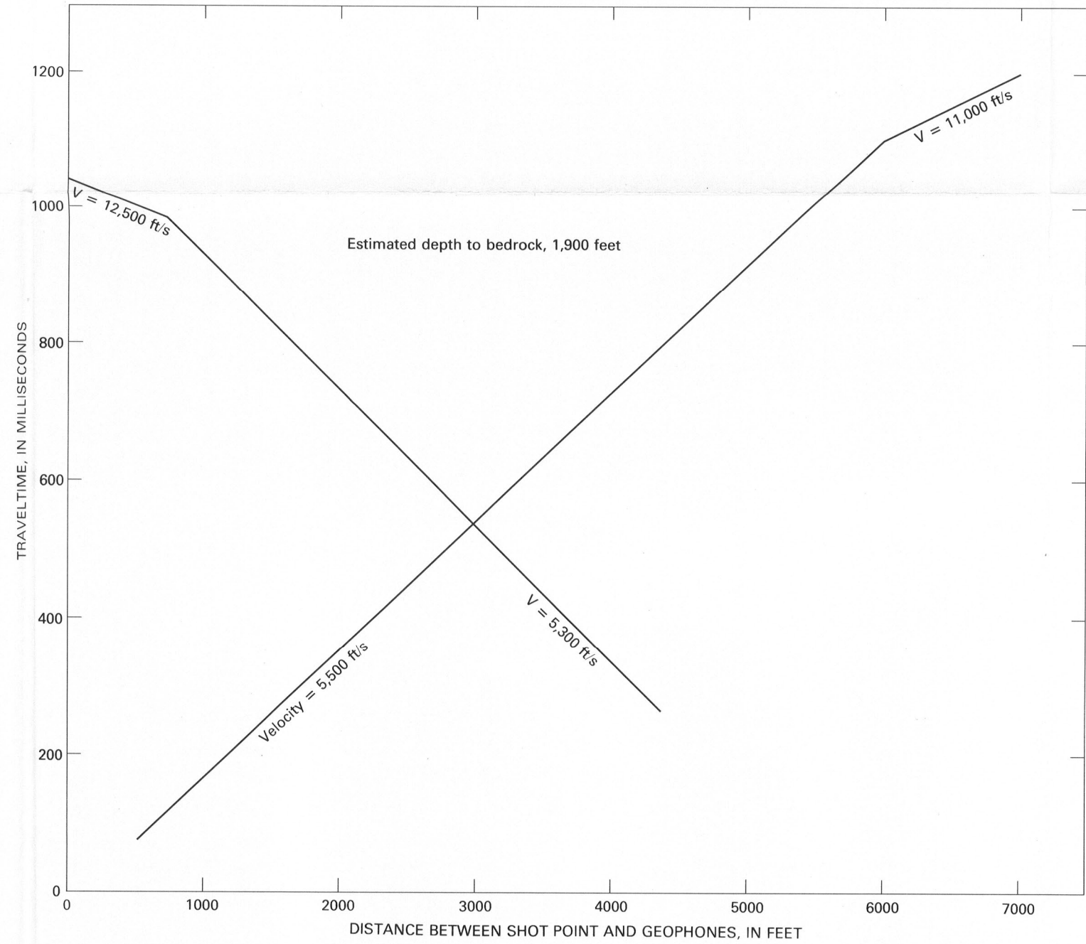
FIGURE 4—Relation between traveltime of seismic wave and distance between shot point and geophones at site S4.
