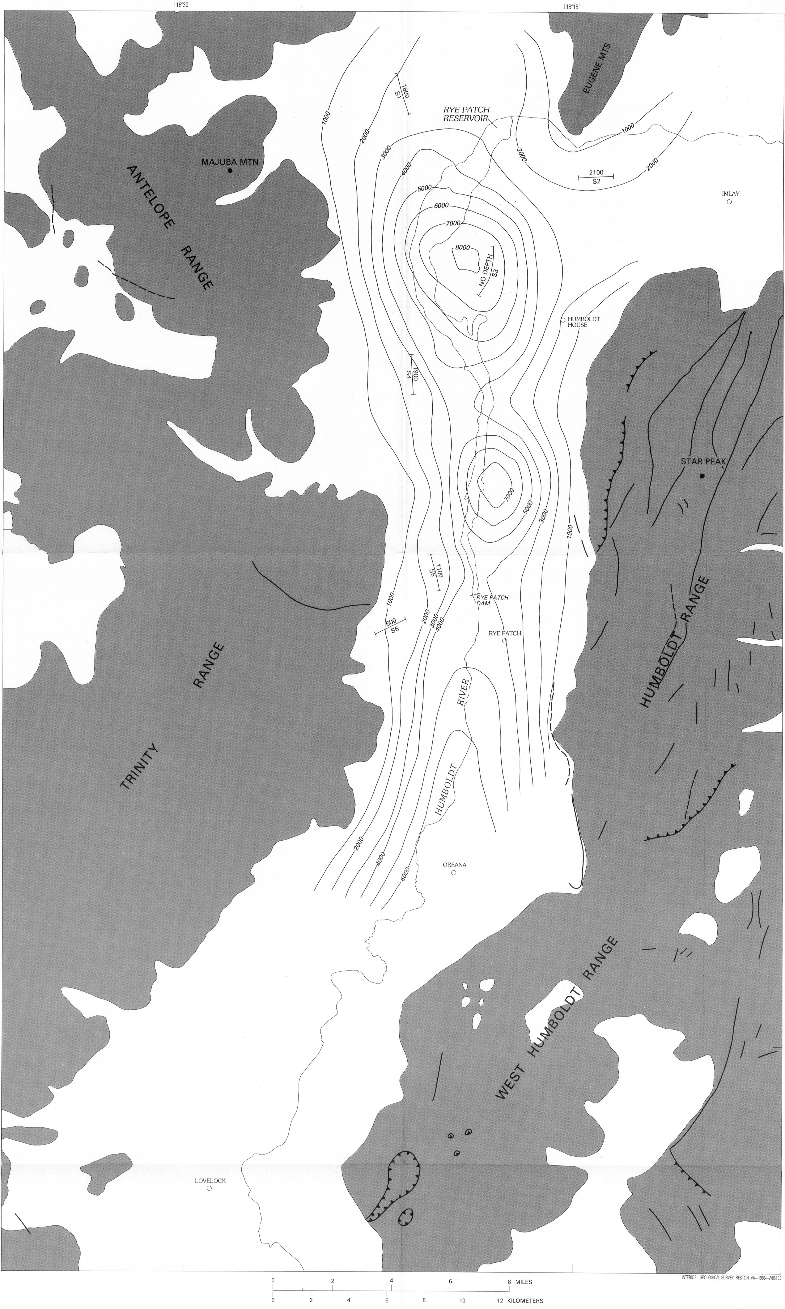
FIGURE 3—Depth to bedrock and location of seismic refraction lines.
