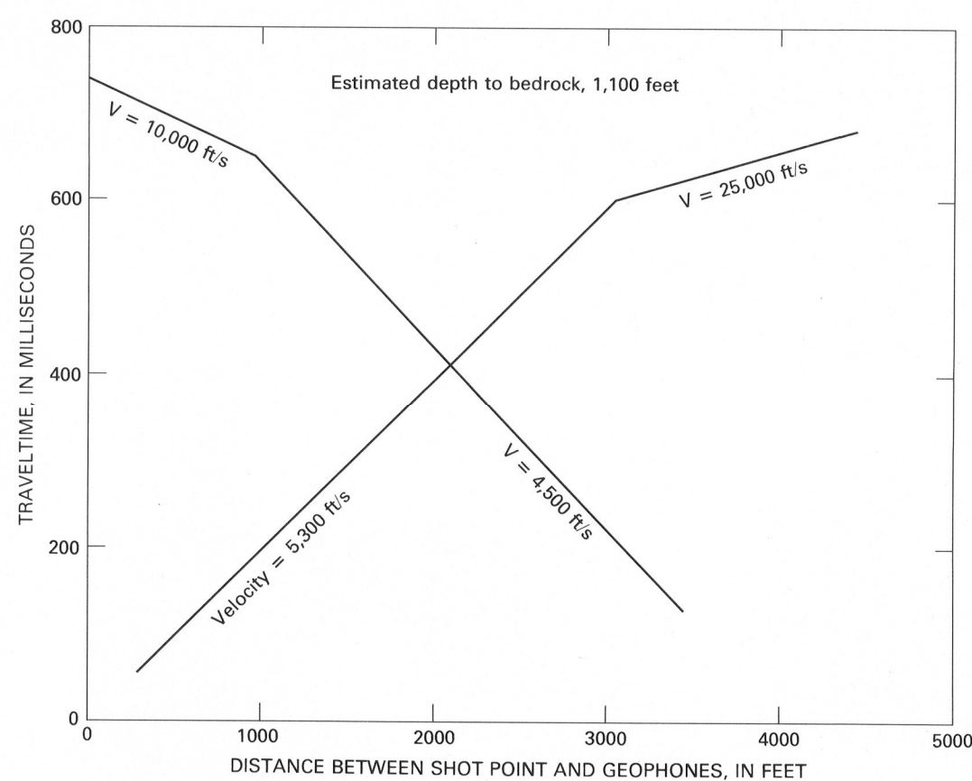
FIGURE 5—Relation between traveltime of seismic wave and distance between shot point and geophones at site S5.
