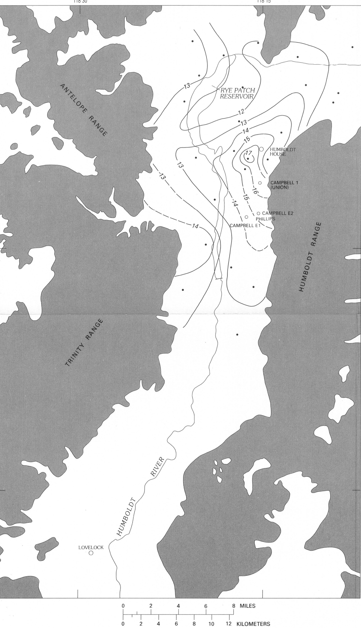
FIGURE 6—Temperature at a depth of 6.6 feet (2 meters).
