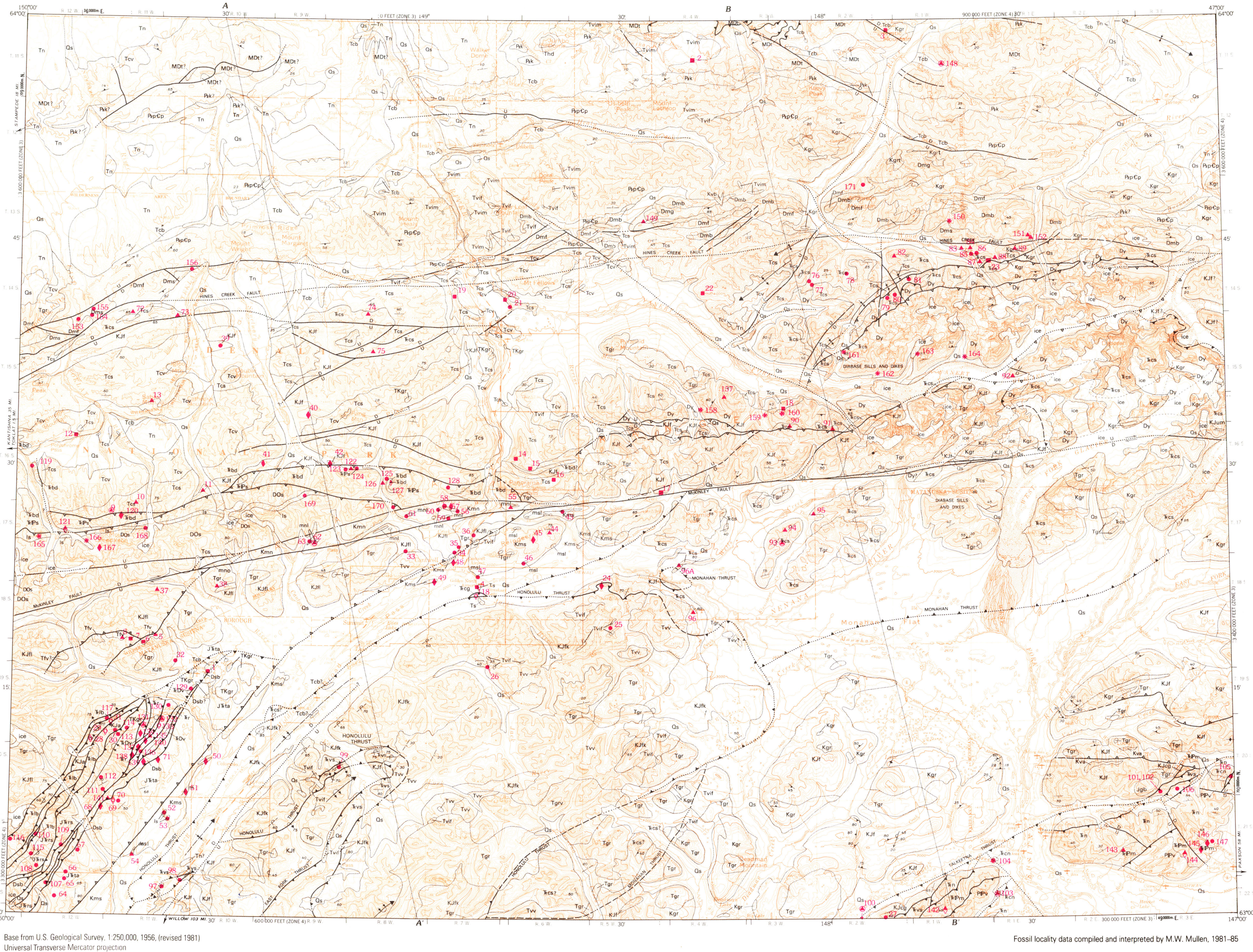
MAP B. FOSSIL LOCALITIES
