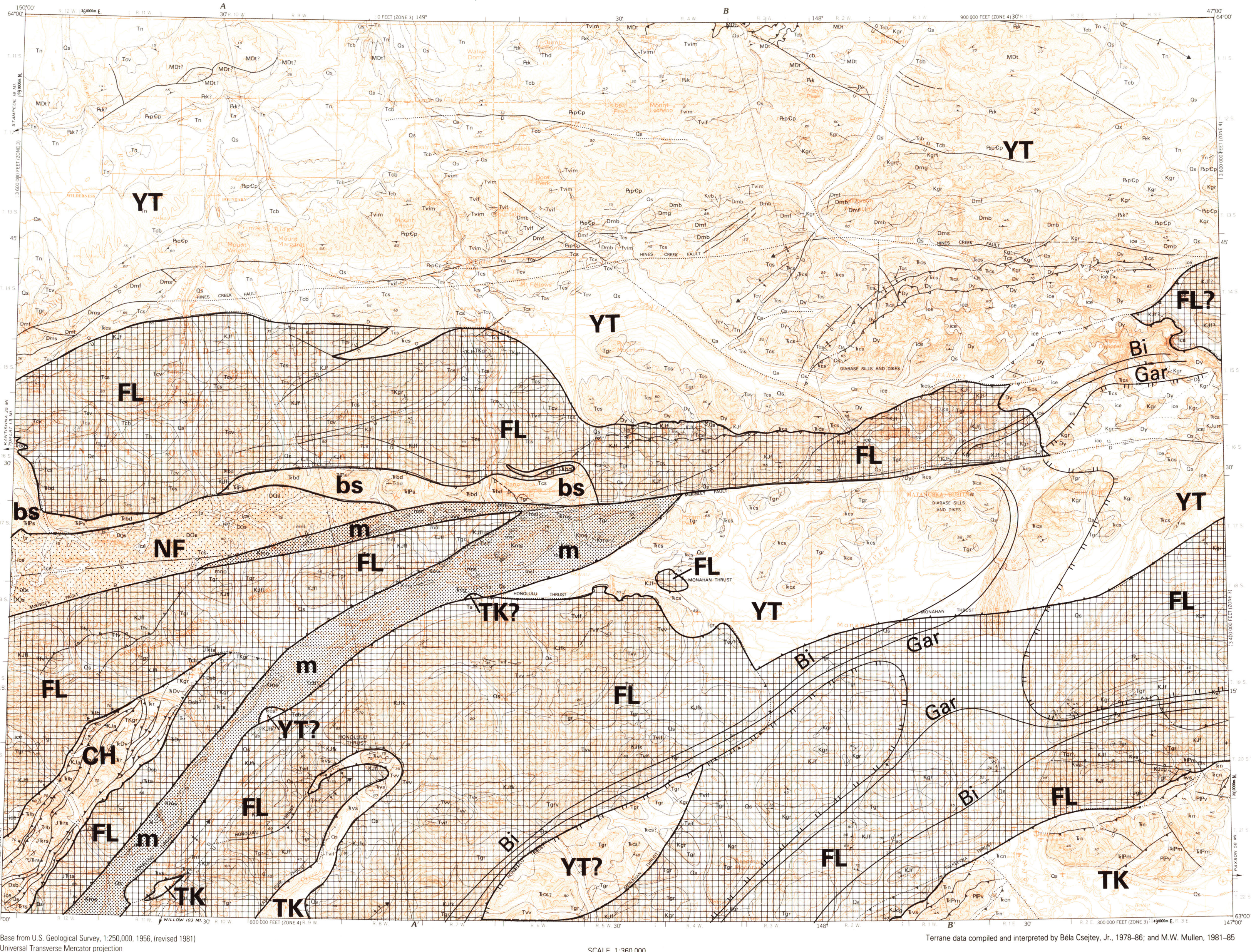
MAP C. TECTONOSTRATIGRAPHIC TERRANE MAP AND THE APPROXIMATE EXTENT OF THE MID-CRETACEOUS MACLAREN METAMORPHIC BELT
