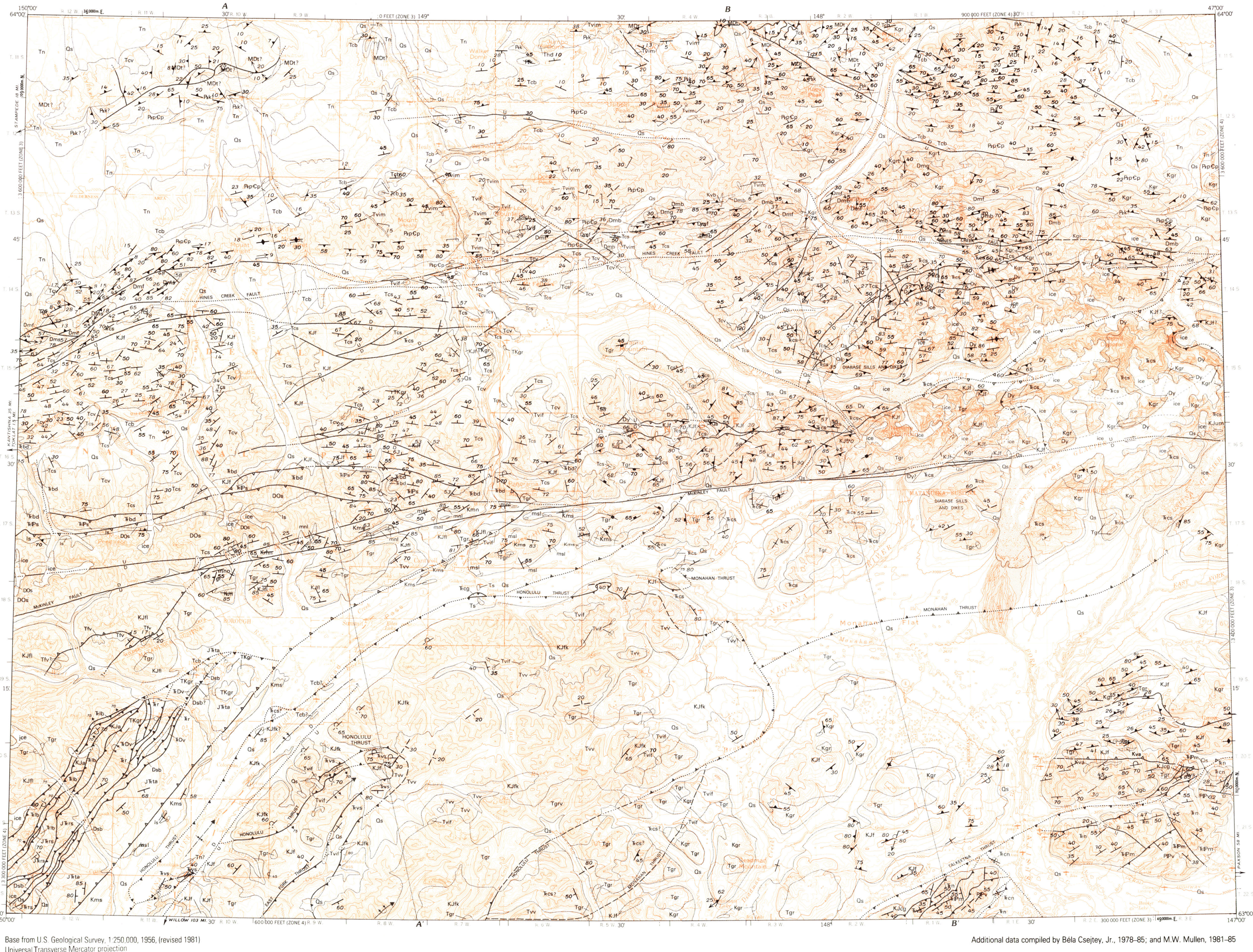
MAP A. ADDITIONAL BEDDING AND STRUCTURAL DATA
