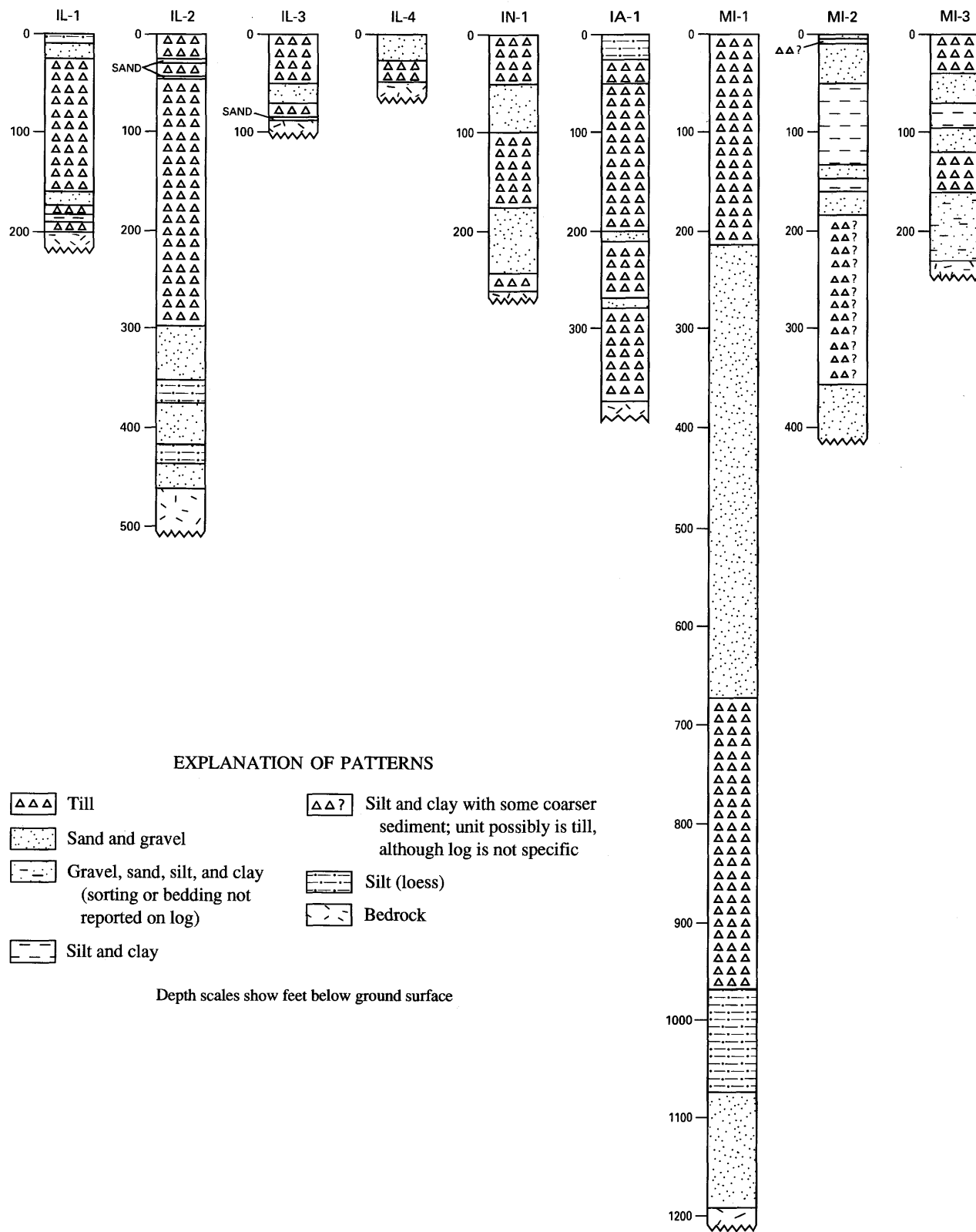
Figure 2. —Selected lithologic logs illustrating subsurface lithologic variations in different geologic settings, including buried valleys, moraines, interlobate areas, river valleys, and upland areas. Locations are shown on map. Logs were selected to alert the map user to the potential vertical lithologic variations in different settings, and to show the subsurface in certain areas where stack units are mapped. Similar lithologic variations in similar geologic settings are not implied; therefore, extrapolation of log data should be avoided. Depth scales show feet below ground surface.
