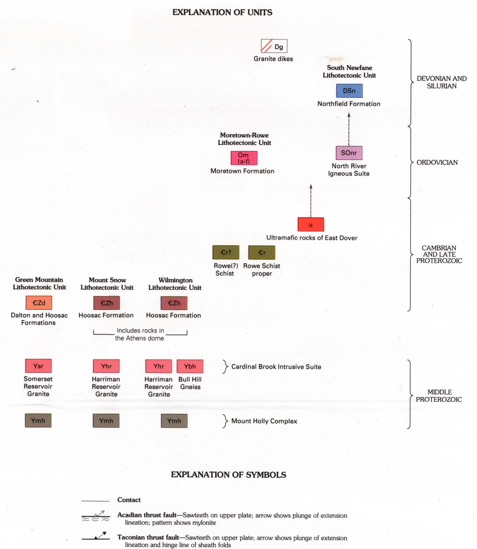
Figure 1. —Geologic map of the Sadawga, Raponda, and southern Athens dome areas, southern Vermont, from Ratcliffe and others (1992), Ratcliffe (1993a, 1997), and this report. West Dover–Jacksonville map area outlined.
