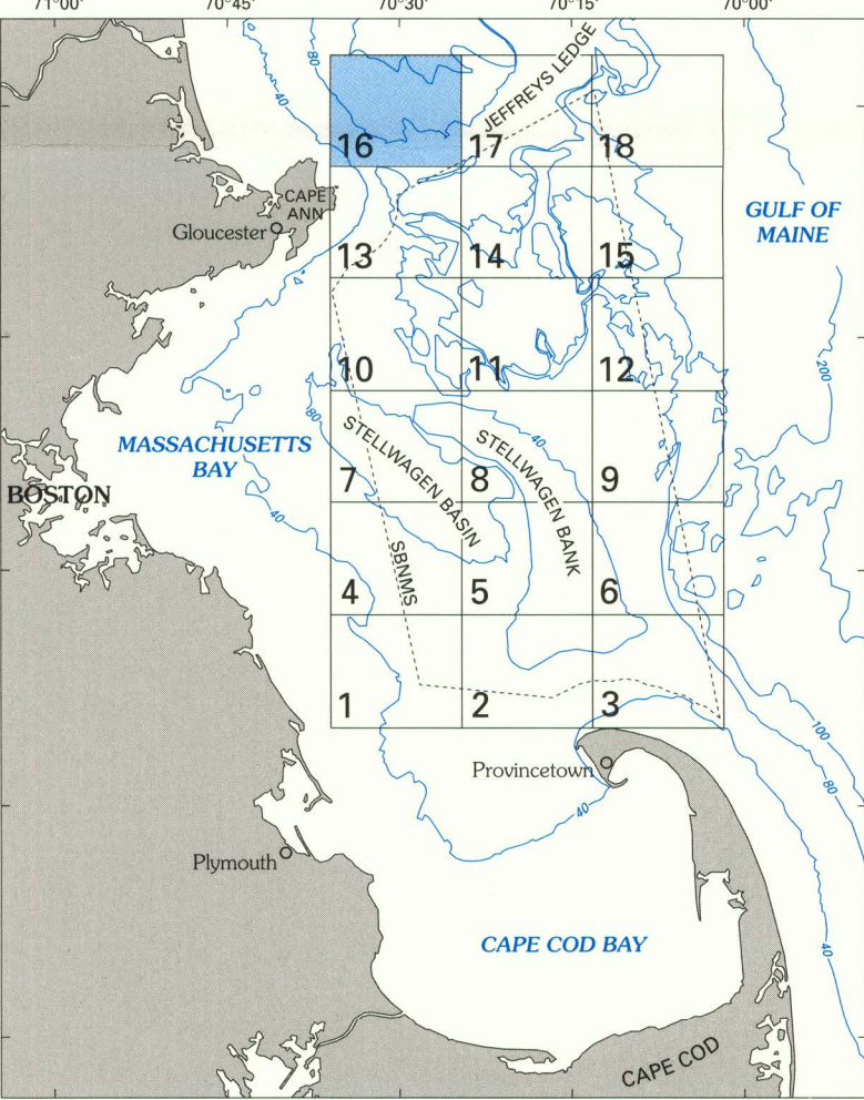
Location map outlining the 18 quadrangles in this series. Quadrangle 16 shown in blue. Boundary of Stellwagen Bank National Marine Sanctuary (SBNMS) indicated by dashed line. Bathymetric contours in meters.
