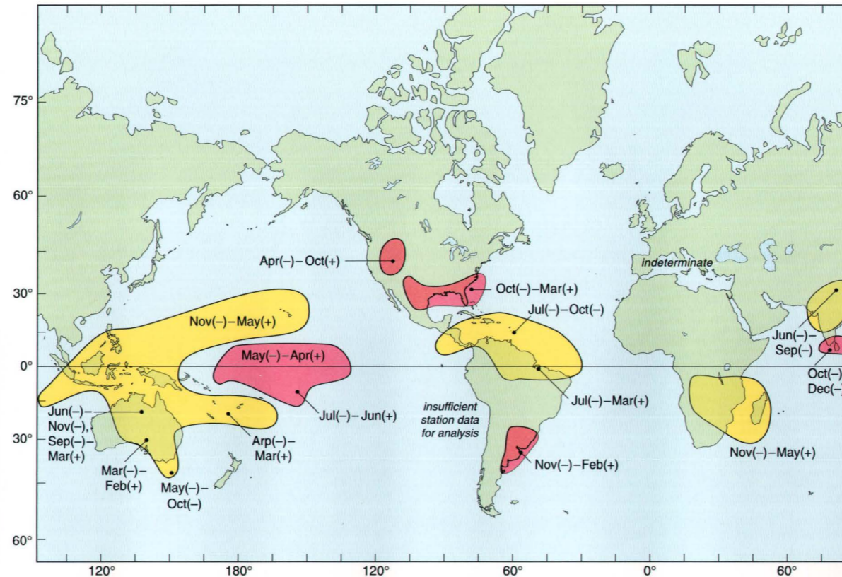
During El Niño, precipitation is enhanced in some (pink) areas and diminished in other (yellow) regions. The months indicate when these regions are affected, typically coinciding with local rainy seasons. The year that unusually high sea-surface temperatures first appear is indicated by (-); (+) refers to the following year. (Source: Philander, 1992).
