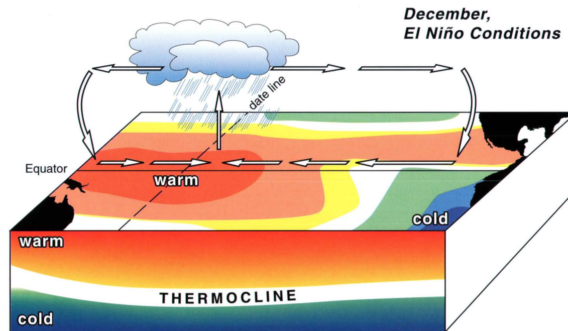
In an El Niño year, the trade winds relax, allowing a surge of warm water eastward across the Pacific and changing the characteristics of waters in the eastern part of the ocean basin. (Source: Philander, 1992)
