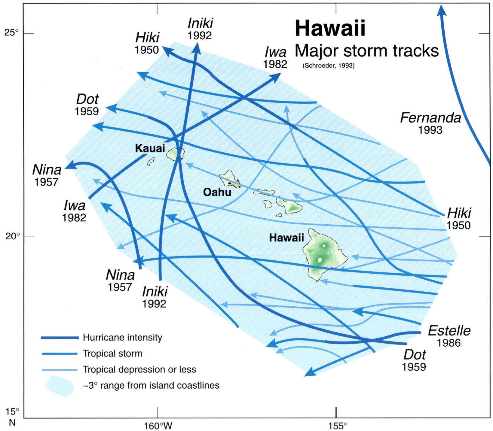
Tracks of the major storms that have affected the main Hawaiian Islands.
