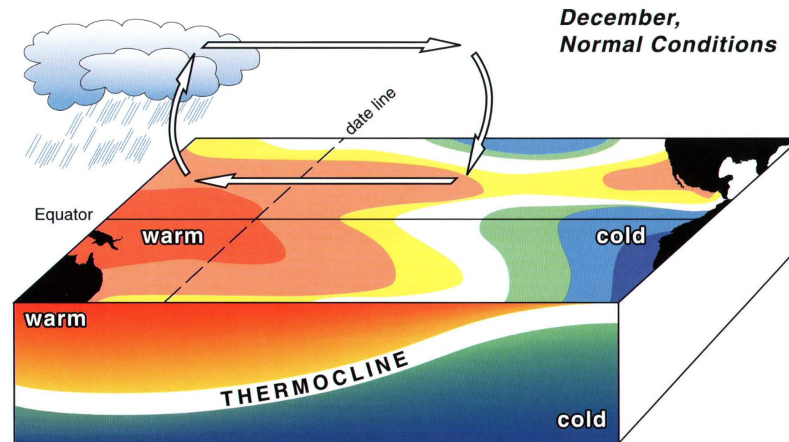
In a normal year, intense westward winds (white arrows) drive equatorial currents that push warm Pacific surface waters steadily to the west and expose colder waters from the deeper water column, to the surface in the east. (Source: Philander, 1992)
