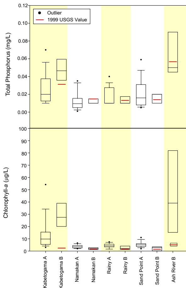
Figure 14. Comparison of total phosphorus and chlorophyll- a data collected by the the U.S. Geological Survey (Payne 1991) and the Minnesota Department of Natural Resources (Eibler 2001b,c and unpublished data) from selected lakes in Voyageurs National Park. A represents data collected by MNDNR (July and September 1983-2000; n=14-16 ). B represents data collected from USGS (August 1977-1983; n=4-7 ).
