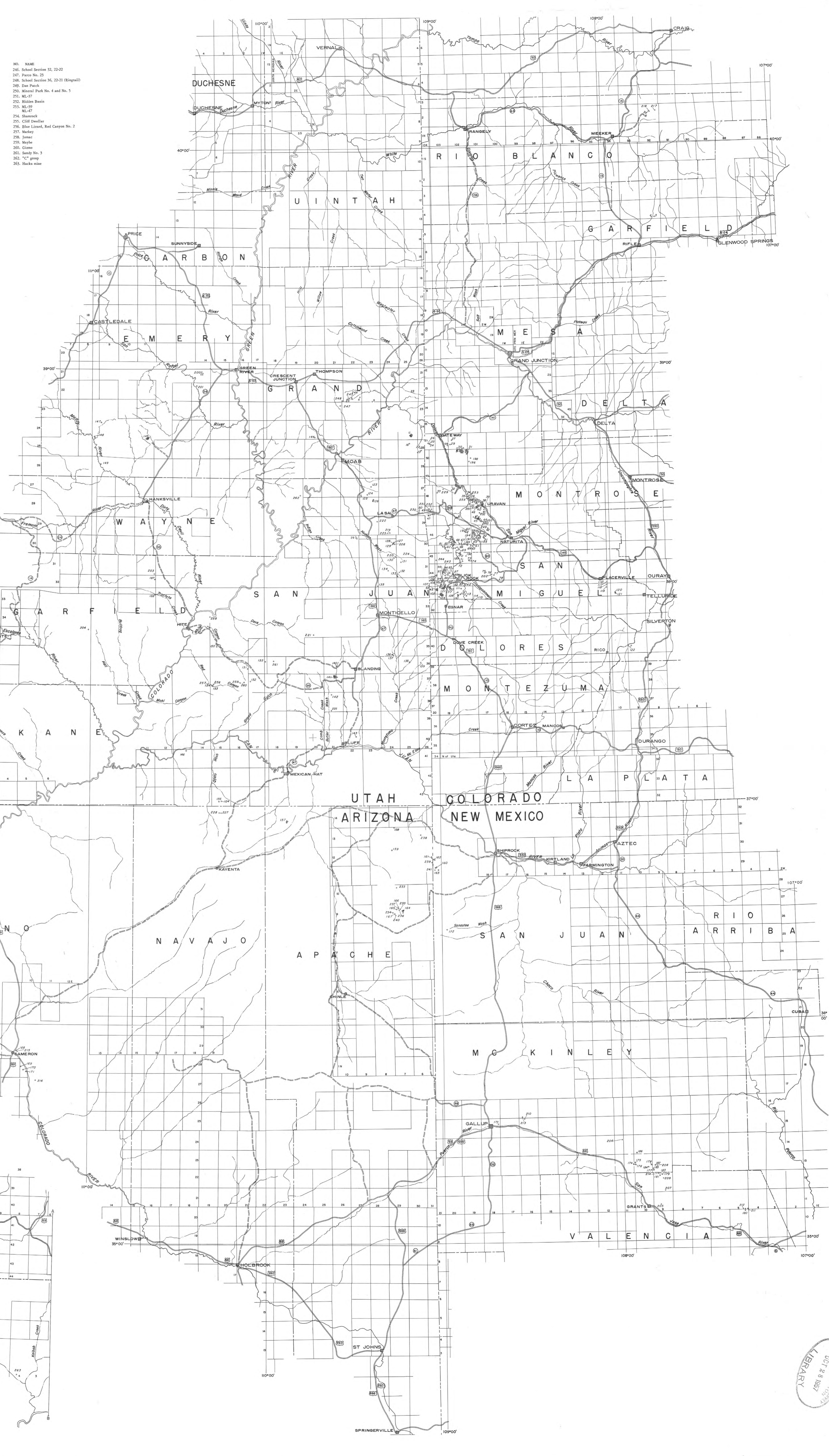
URANIUM AND VANADIUM DEPOSITS OF THE COLORADO PLATEAU THAT PRODUCED MORE THAN 1,000 TONS OF ORE THROUGH JUNE 30, 1955
