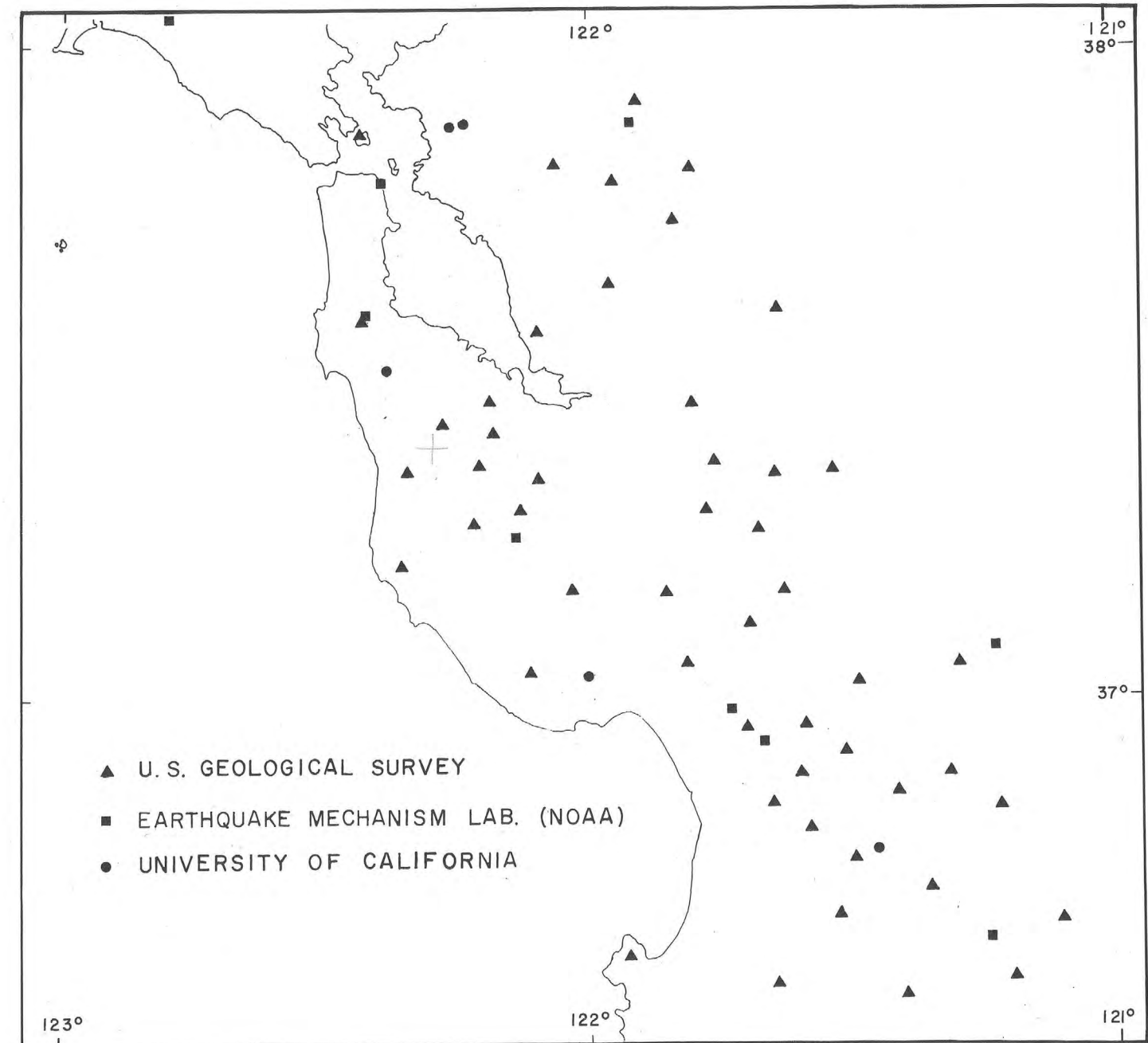
MAP SHOWING DISTRIBUTION OF SEISMOGRAPH STATIONS, SOUTHERN SAN FRANCISCO BAY REGION, 1969-1970
