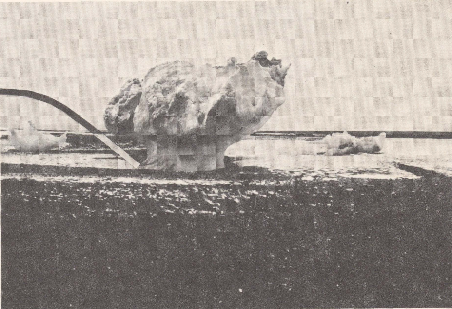
D. Current scour occurs around grounded ice on the inner shelf, where flow velocities of 2 to 3 knots are common. Under such conditions, turbid-water wakes and flow patterns in the surficial drift ice are pronounced. If the ice and its scour depression continue to move, a sequence of cut-and-fill structures will develop in the sediment. The photograph shows such current scour on a barrier island, following a 3-meter drop in sea level after a storm surge (Reimnitz and others, 1972).
