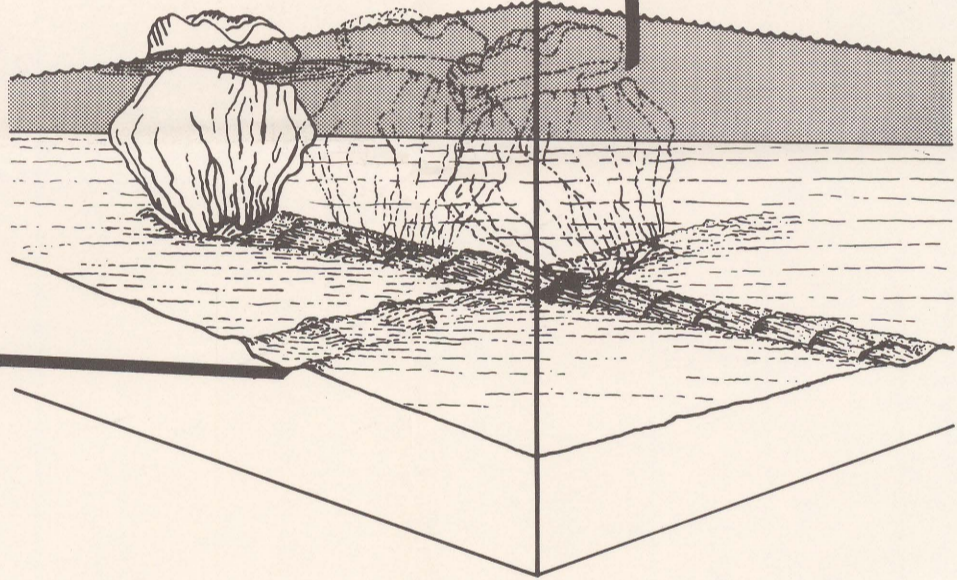
B. Metastable chunks of ice touching the bottom sometimes wobble, creating regularly spaced bottom features. Also illustrated are notches formed at sea level by wave action during the summer. Grounded ice often is marked by elevated swash notches, which may indicate the depth range traversed by the ice after grounding.
