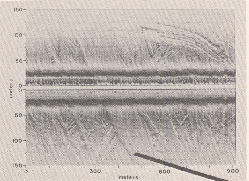
B. Metastable chunks of ice touching the bottom sometimes wobble, creating regularly spaced bottom features. Also illustrated are notches formed at sea level by wave action during the summer. Grounded ice often is marked by elevated swash notches, which may indicate the depth range traversed by the ice after grounding.
