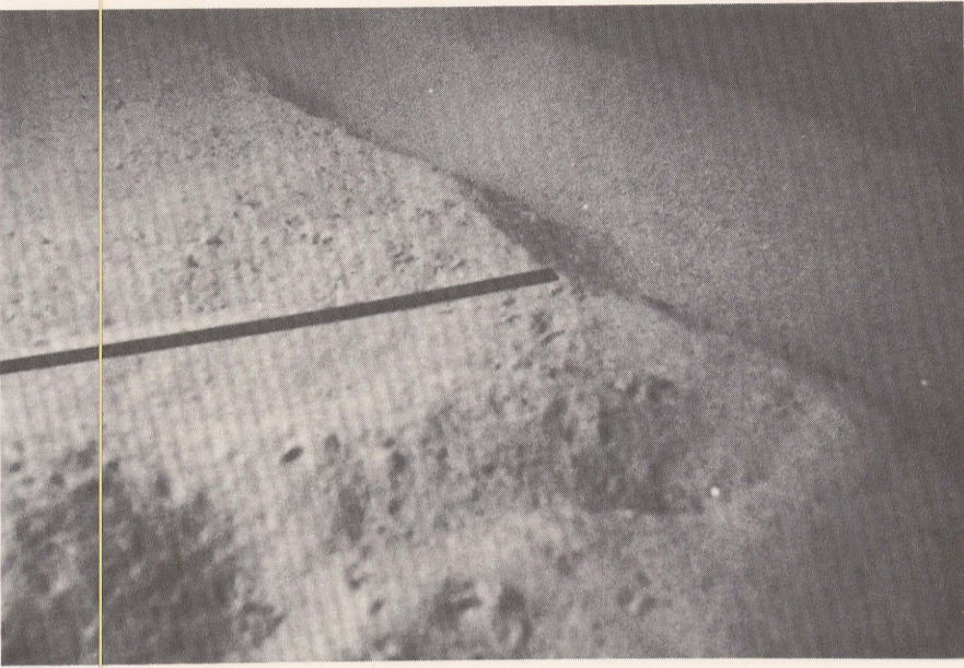
A. The most common bottom features are grooves that single pieces of ice cut in unconsolidated sediments, ranging from mud to coarse gravel. The sonograph demonstrates how a gouge may change shape due to rotation of the cutting tool. The underwater photo shows an 80-cm-wide gouge in medium-grained sand.
