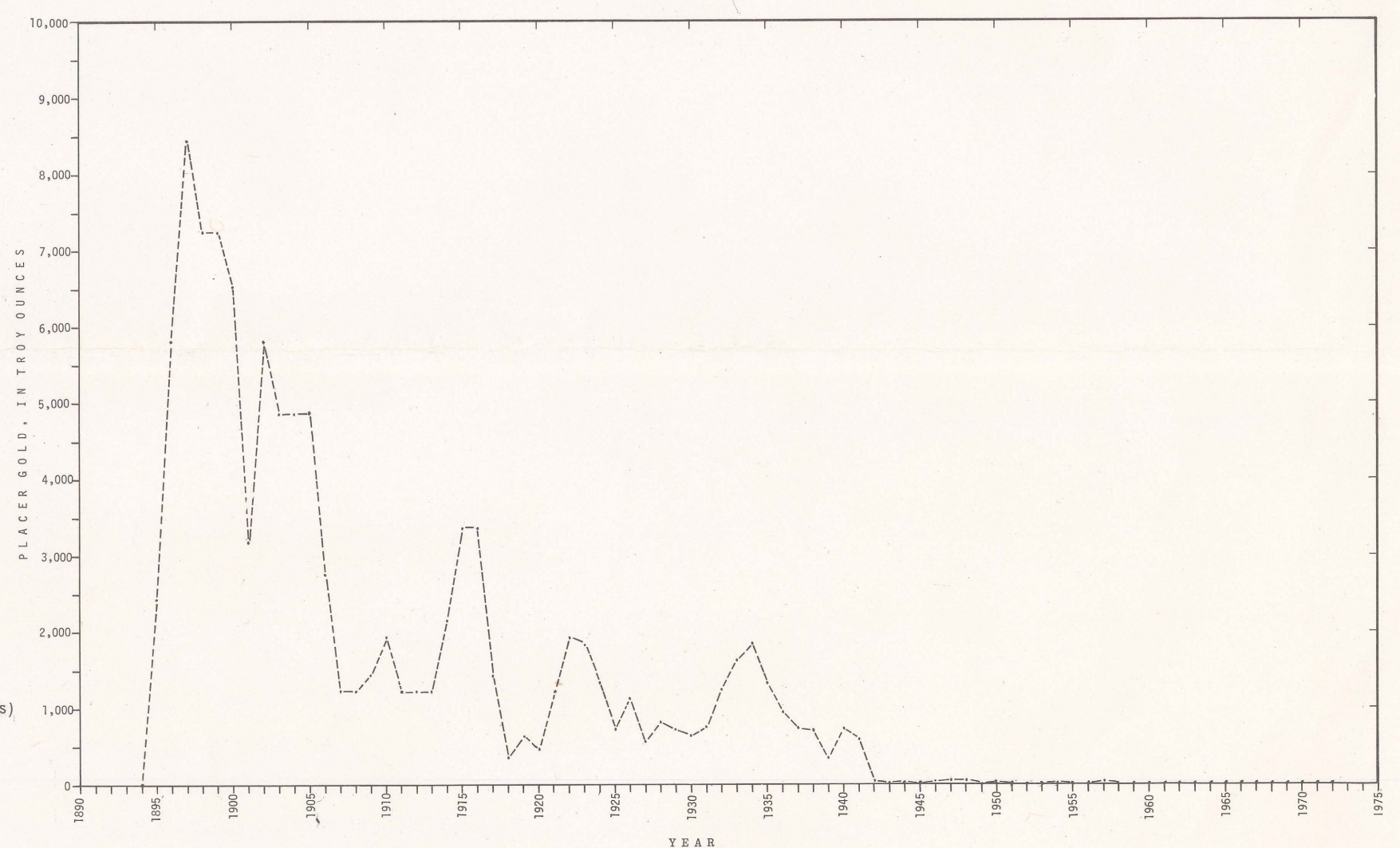
Figure 1.—Placer gold production of Seward and Blying Sound quadrangles. Data compiled from Smith (1934) for 1893-1930; unpublished records of U.S. Geological Survey for 1931-46; and Minerals Yearbooks of U.S. Bureau of Mines for 1947-72.
