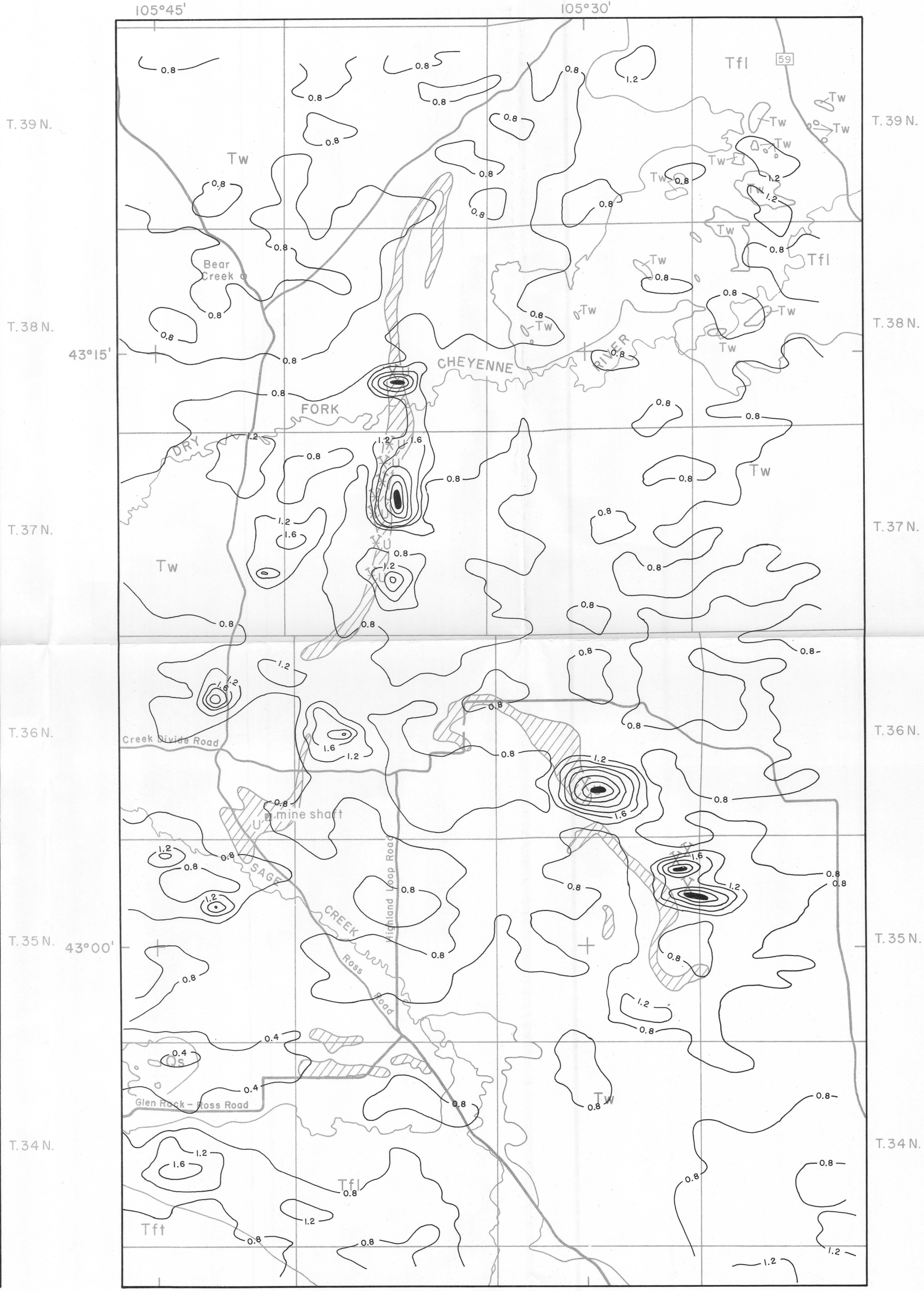
FIGURE 5.--MAP SHOWING RATIO OF PPM EU/PERCENT K. CONTOUR INTERVAL 0.4 PPM/PERCENT.
