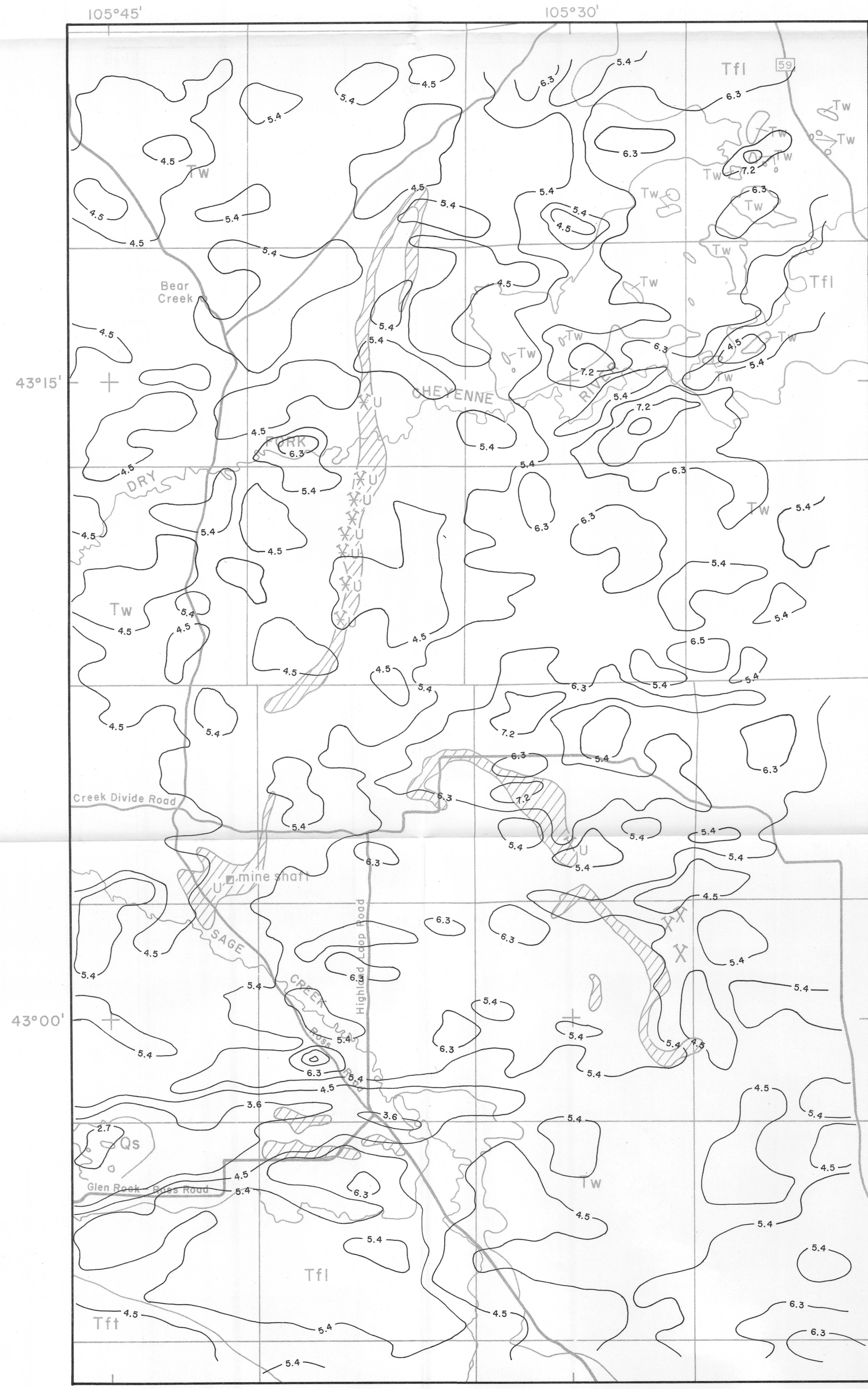
FIGURE 6.--MAP SHOWING RATIO OF PPM ETH/PERCENT K. CONTOUR INTERVAL 0.9 PPM/PERCENT.
