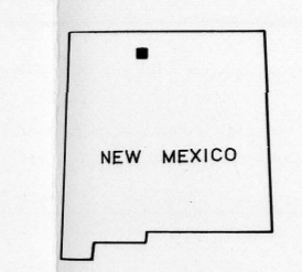
STRUCTURE CONTOUR MAP ISOPACH AND STRUCTURE CONTOUR MAPS OF THE BURRO CANYON(?) FORMATION IN THE MESA GOLONDRINA AND MESA DE LOS VIEJOS AREAS, CHAMA BASIN, NEW MEXICO
