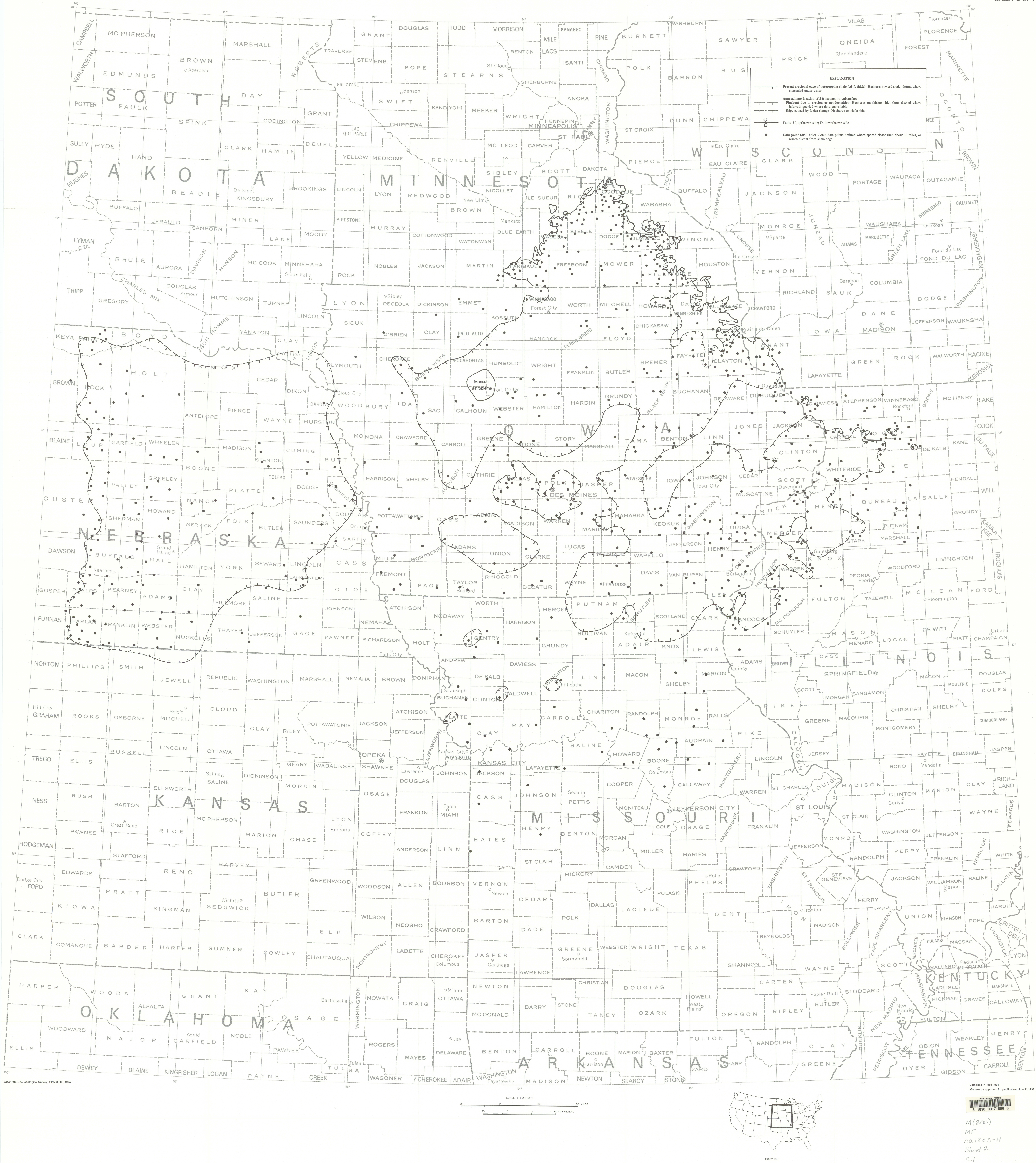
MAP B. AREAL EXTENT OF GLENWOOD SHALE AND EQUIVALENTS
