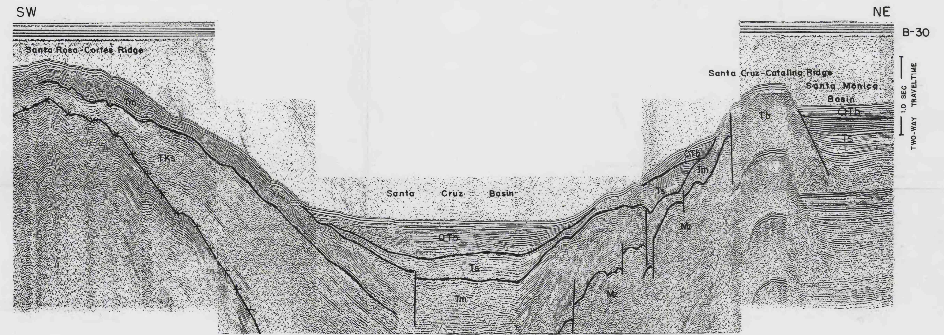
SEISMIC REFLECTION PROFILES OF SANTA CRUZ BASIN
