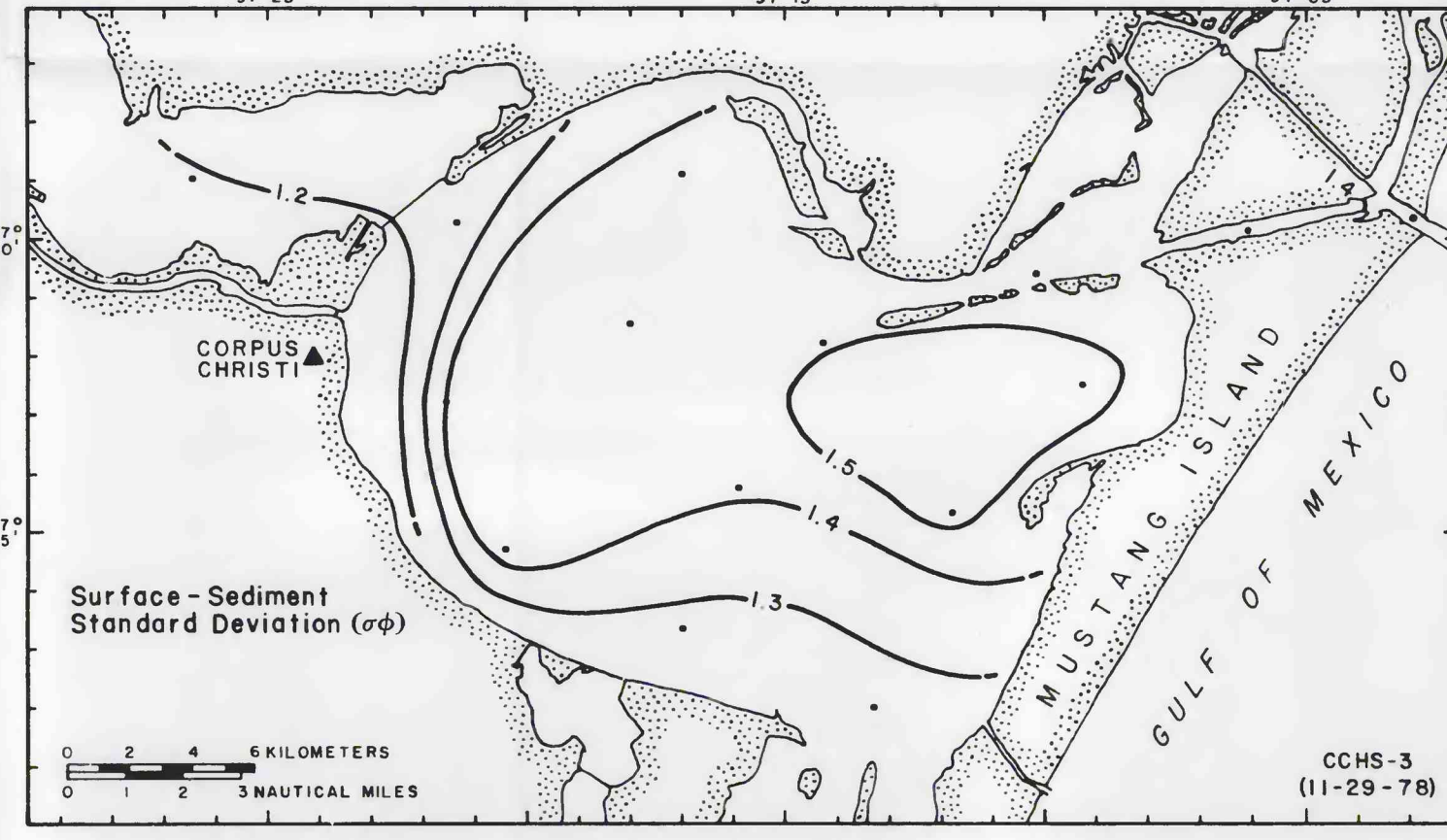
MAPS SHOWING TIME-SEQUENCE SURFACE PATTERNS OF ESTUARINE HYDROGRAPHY AND SUSPENDED SEDIMENTS IN CORPUS CHRISTI BAY, TEXAS GULF COAST
