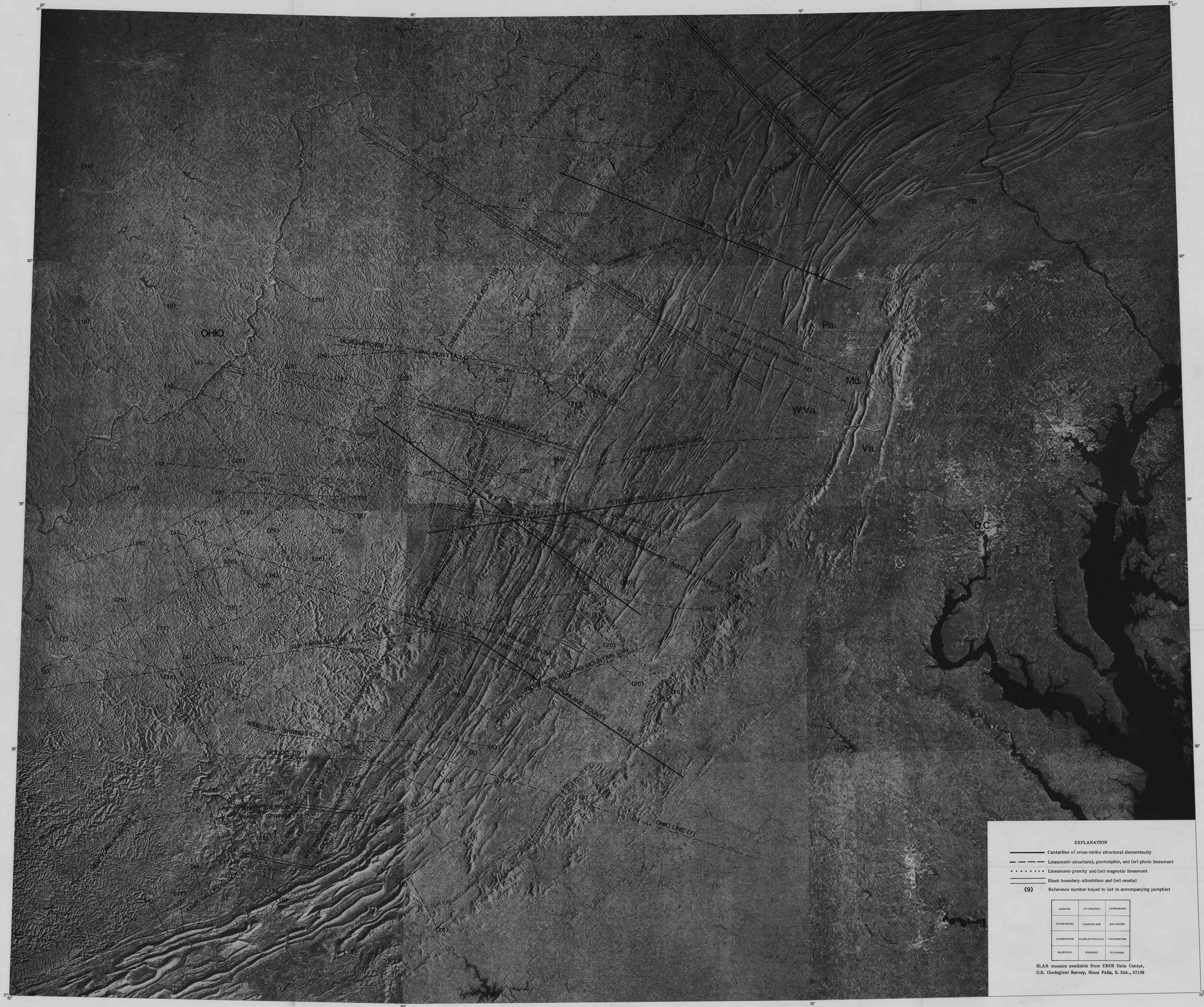
SIDE-LOOKING AIRBORNE RADAR IMAGE MAP SHOWING CROSS-STRIKE STRUCTURAL DISCONTINUITIES AND LINEAMENTS OF THE CENTRAL APPALACHIANS
