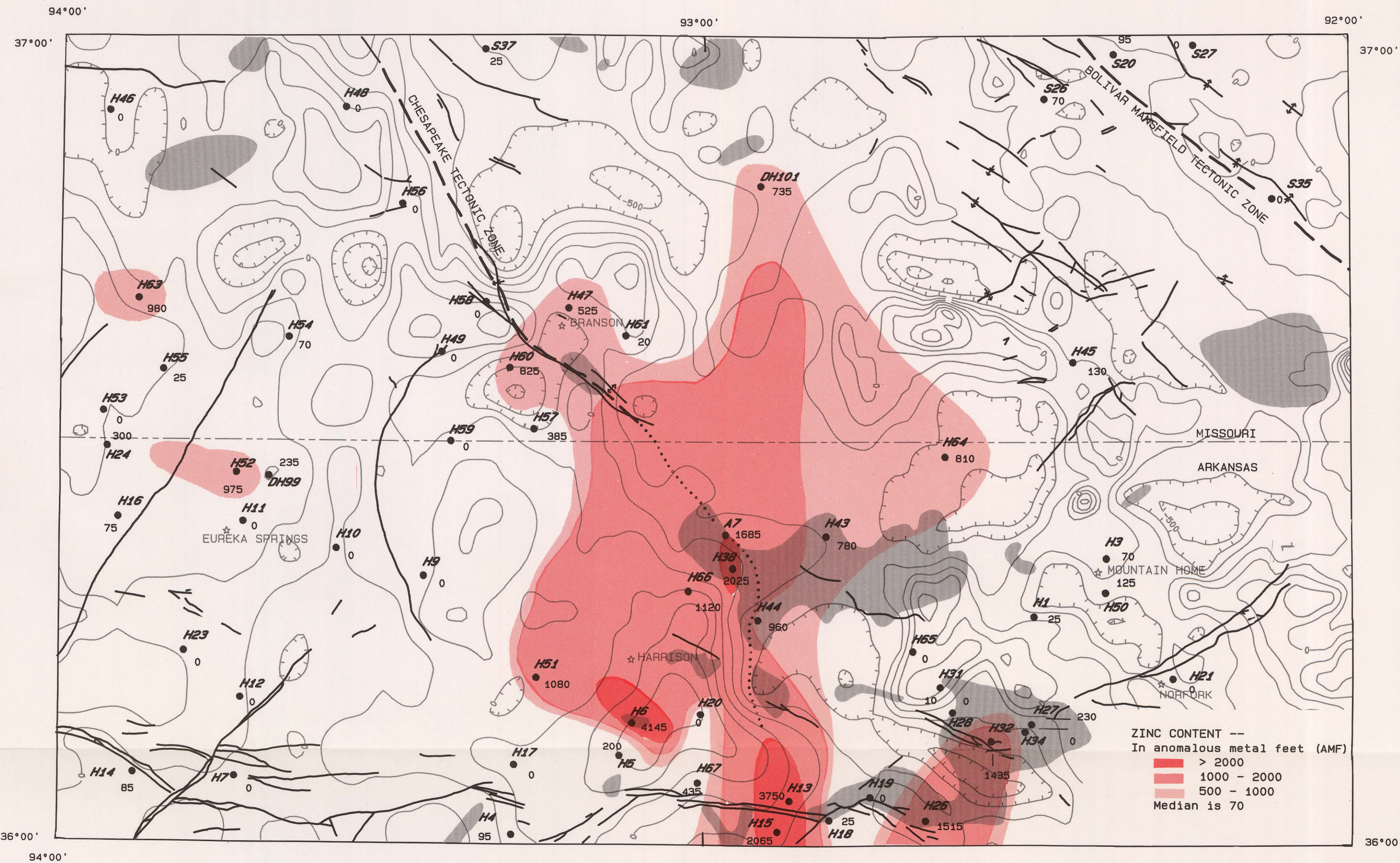
MAP G. DISTRIBUTION AND ABUNDANCE OF ZINC IN INSOLUBLE RESIDUES OF ORDOVICIAN ROCKS
