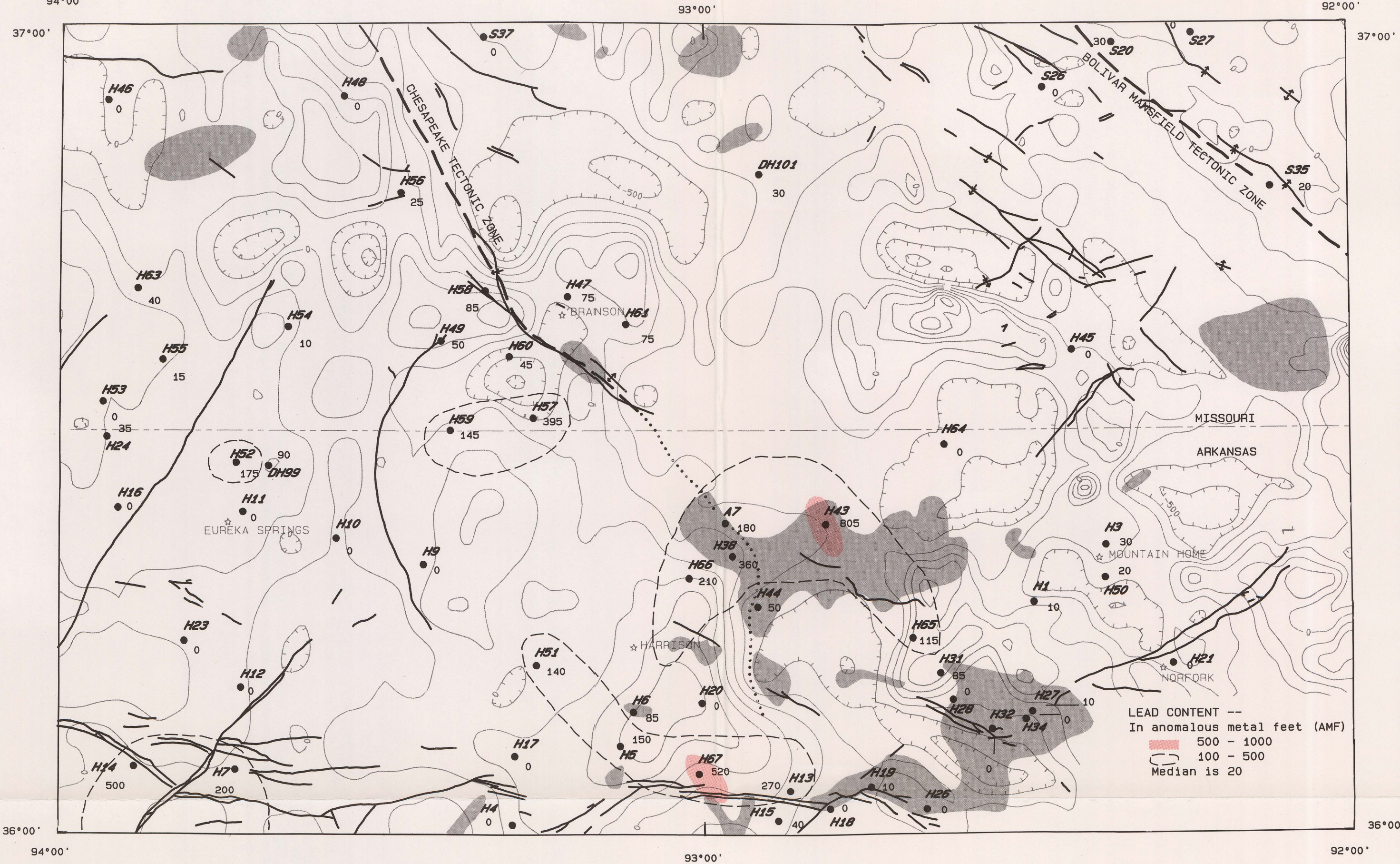
MAP E. DISTRIBUTION AND ABUNDANCE OF LEAD IN INSOLUBLE RESIDUES OF ORDOVICIAN ROCKS
