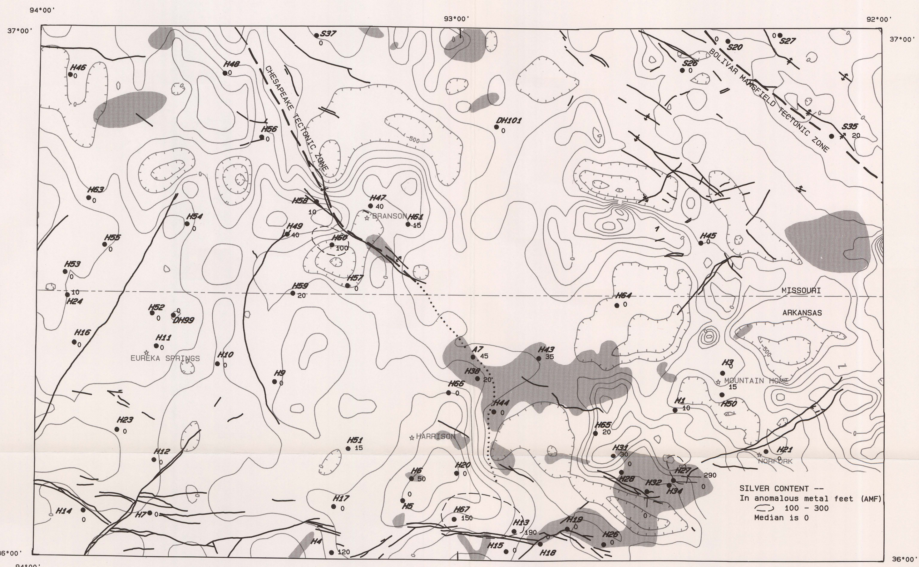
MAP I. DISTRIBUTION AND ABUNDANCE OF SILVER IN INSOLUBLE RESIDUES OF ORDOVICIAN ROCKS
