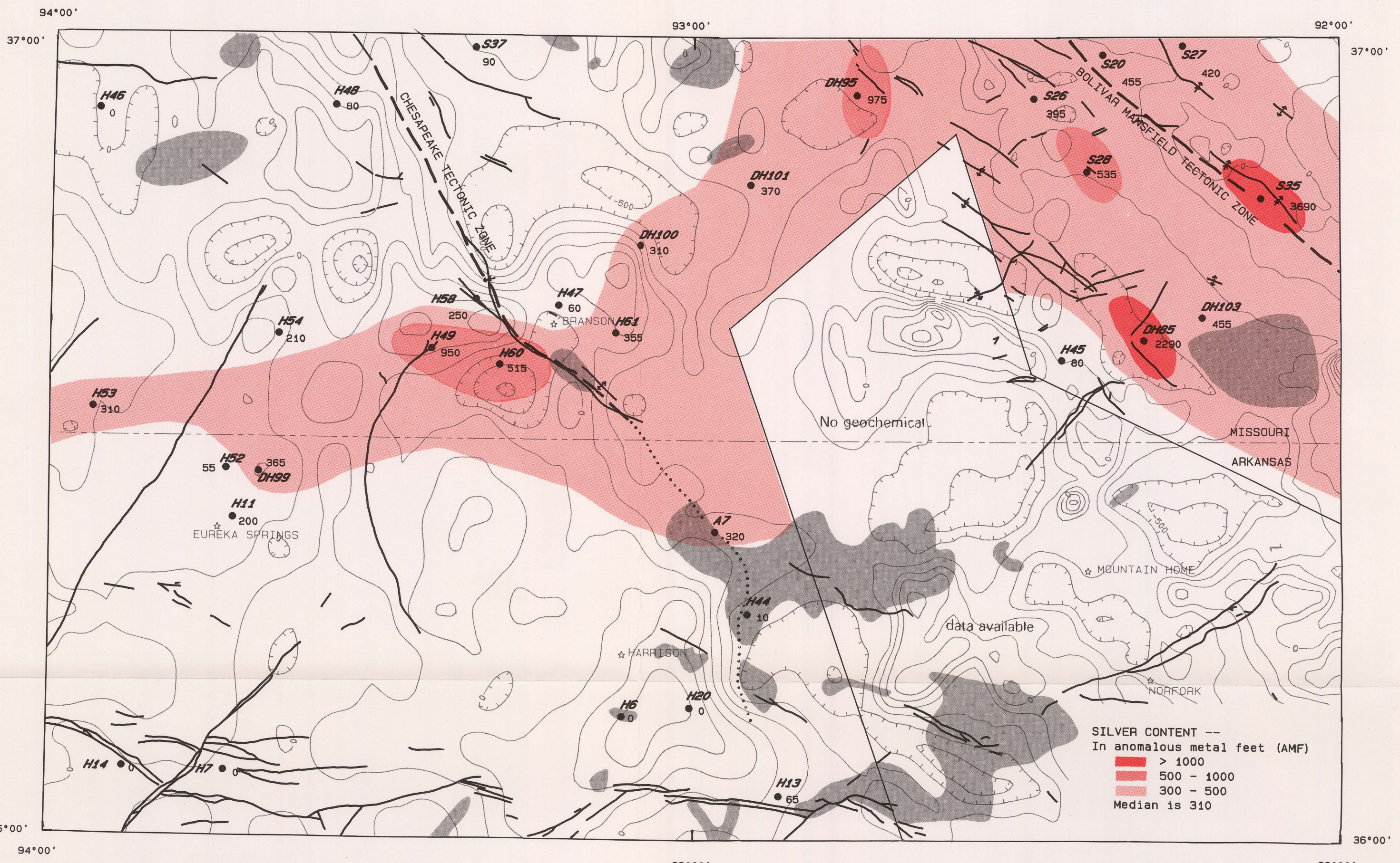
MAP H. DISTRIBUTION AND ABUNDANCE OF SILVER IN INSOLUBLE RESIDUES OF CAMBRIAN ROCKS
