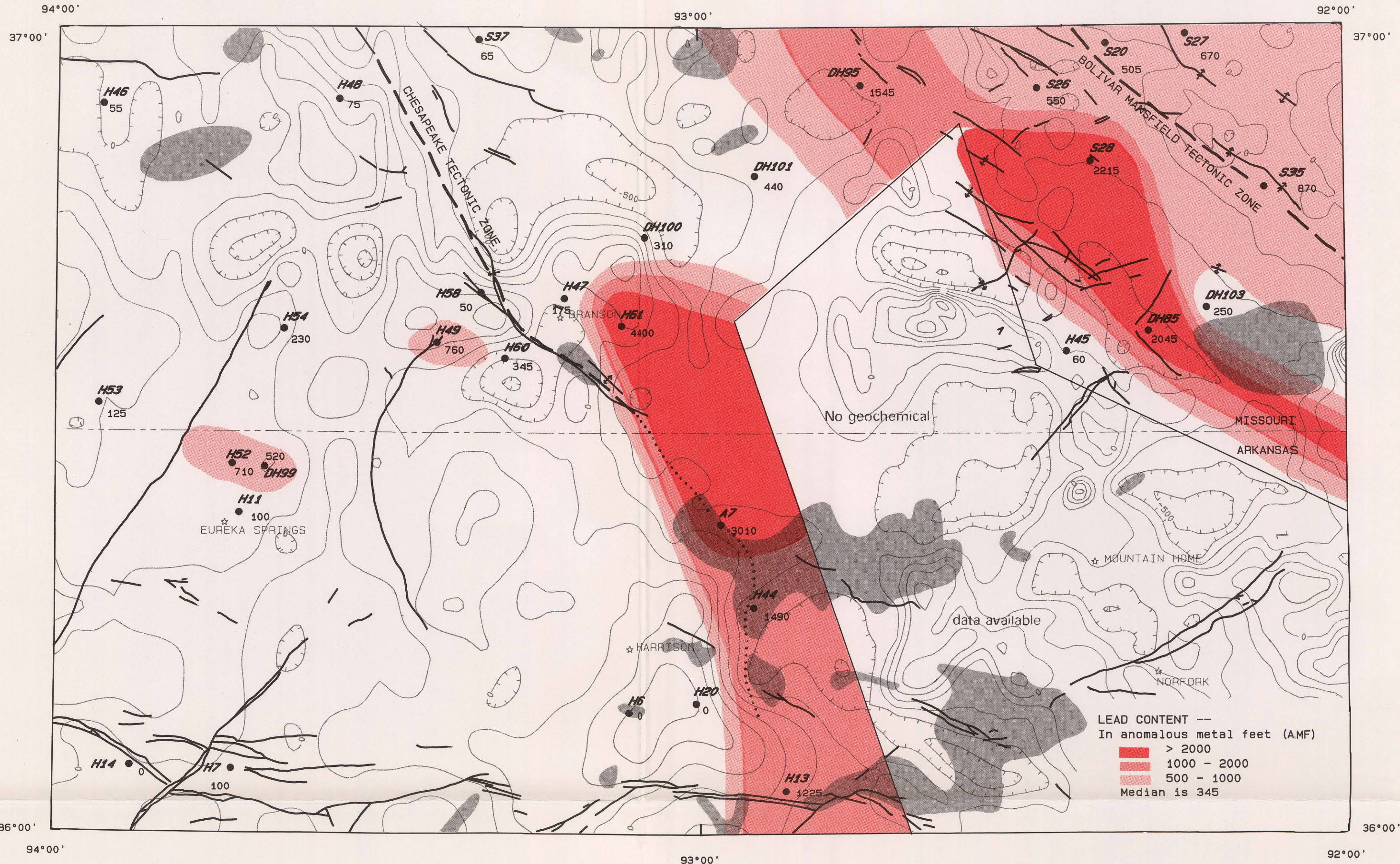
MAP D. DISTRIBUTION AND ABUNDANCE OF LEAD IN INSOLUBLE RESIDUES OF CAMBRIAN ROCKS
