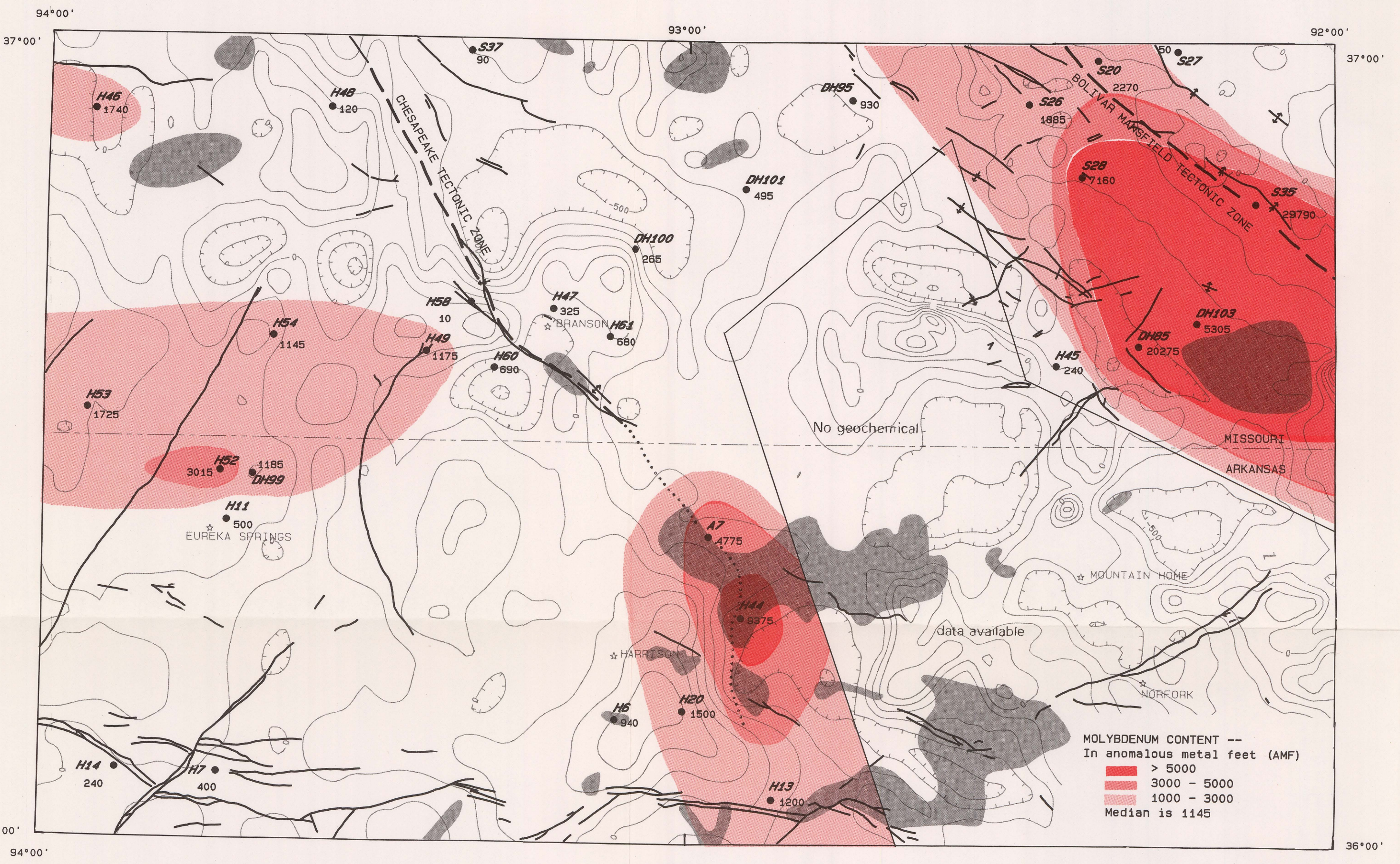
MAP J. DISTRIBUTION AND ABUNDANCE OF MOLYBDENUM IN INSOLUBLE RESIDUES OF CAMBRIAN ROCKS
