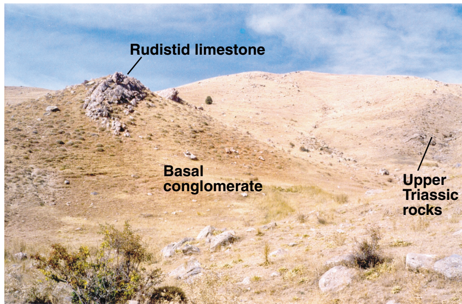
Figure 6. Upper Cretaceous basal conglomerate and rudistid limestone unconformably overlying Upper Triassic rocks in the Jermanis coal field, central Armenia. Upper Cretaceous basal conglomerate is about 20 m thick.
