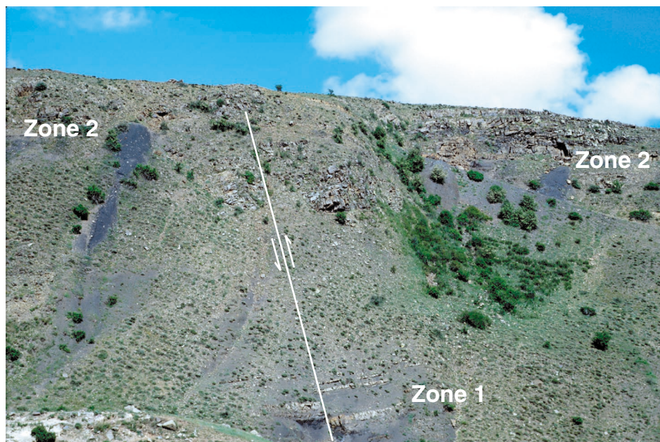
Figure 9. Minor fault and coal zones 1 and 2 in Upper Triassic coal-bearing rocks, northwestern block, Jermanis coal field, central Armenia.
