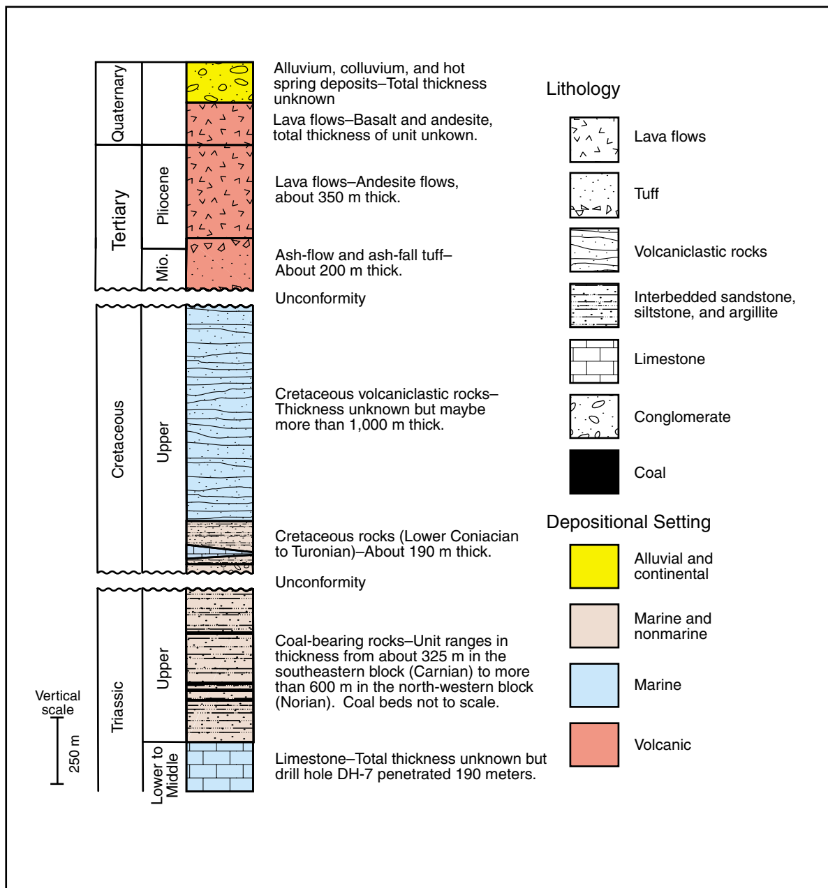
Figure 3. Generalized stratigraphic column of the lithostratigraphic units exposed in the Jermanis coal field, central Armenia. Mio.=Miocene. Thicknesses of rock units from Atabekian and others (1996).
