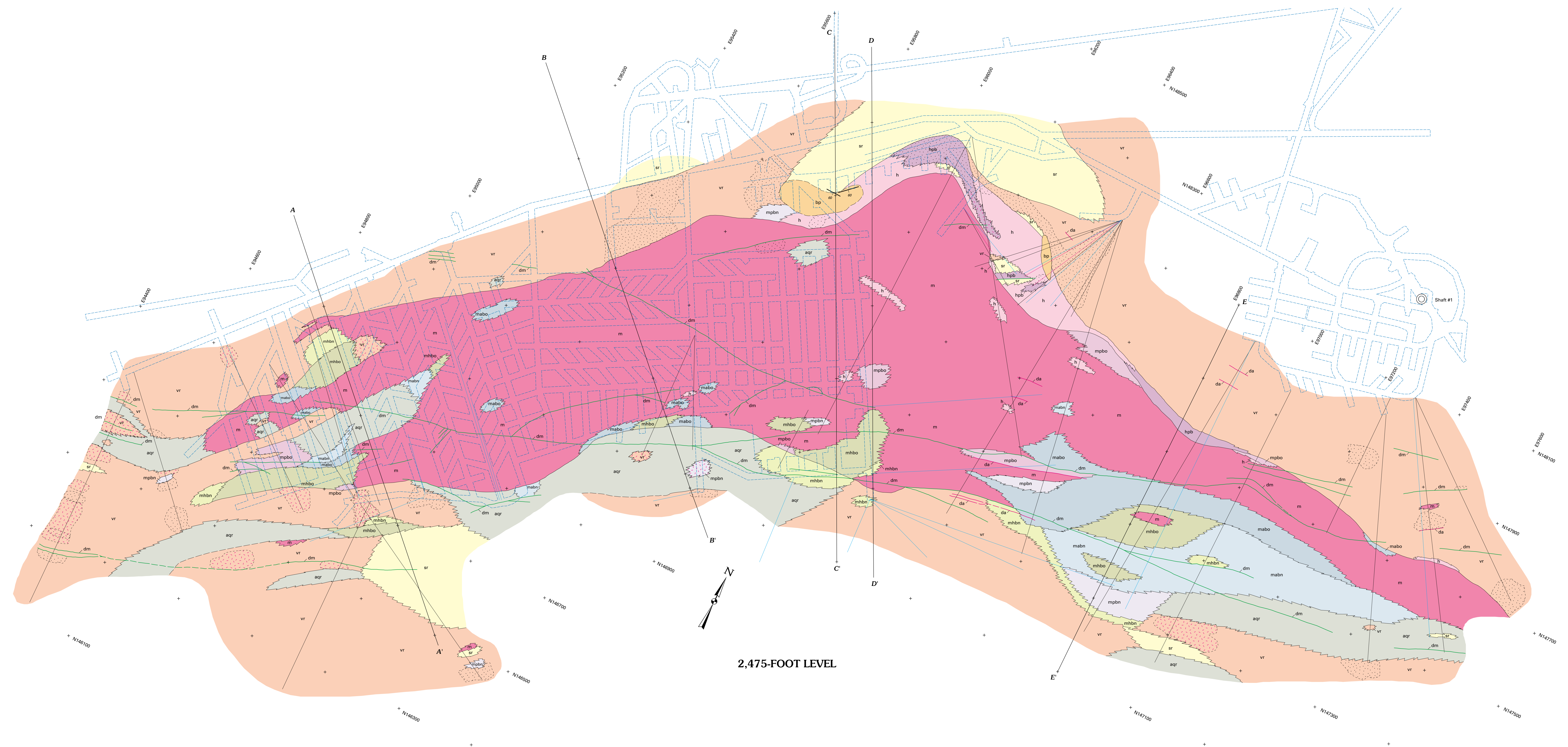
GEOLOGIC MAPS AND CROSS SECTIONS OF MINE LEVELS AT THE PEA RIDGE IRON MINE, WASHINGTON COUNTY, MISSOURI By C.M. Seeger, 1 L.M. Nuelle, 2 W.C. Day, 3 G.B. Sidder, 4 M.A. Marikos, 5 and D.C. Smith 1
