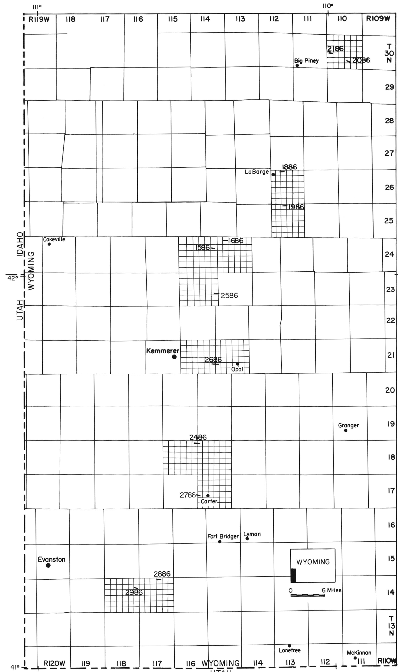
INDEX MAP SHOWING LOCATIONS OF MEASURED SECTIONS
