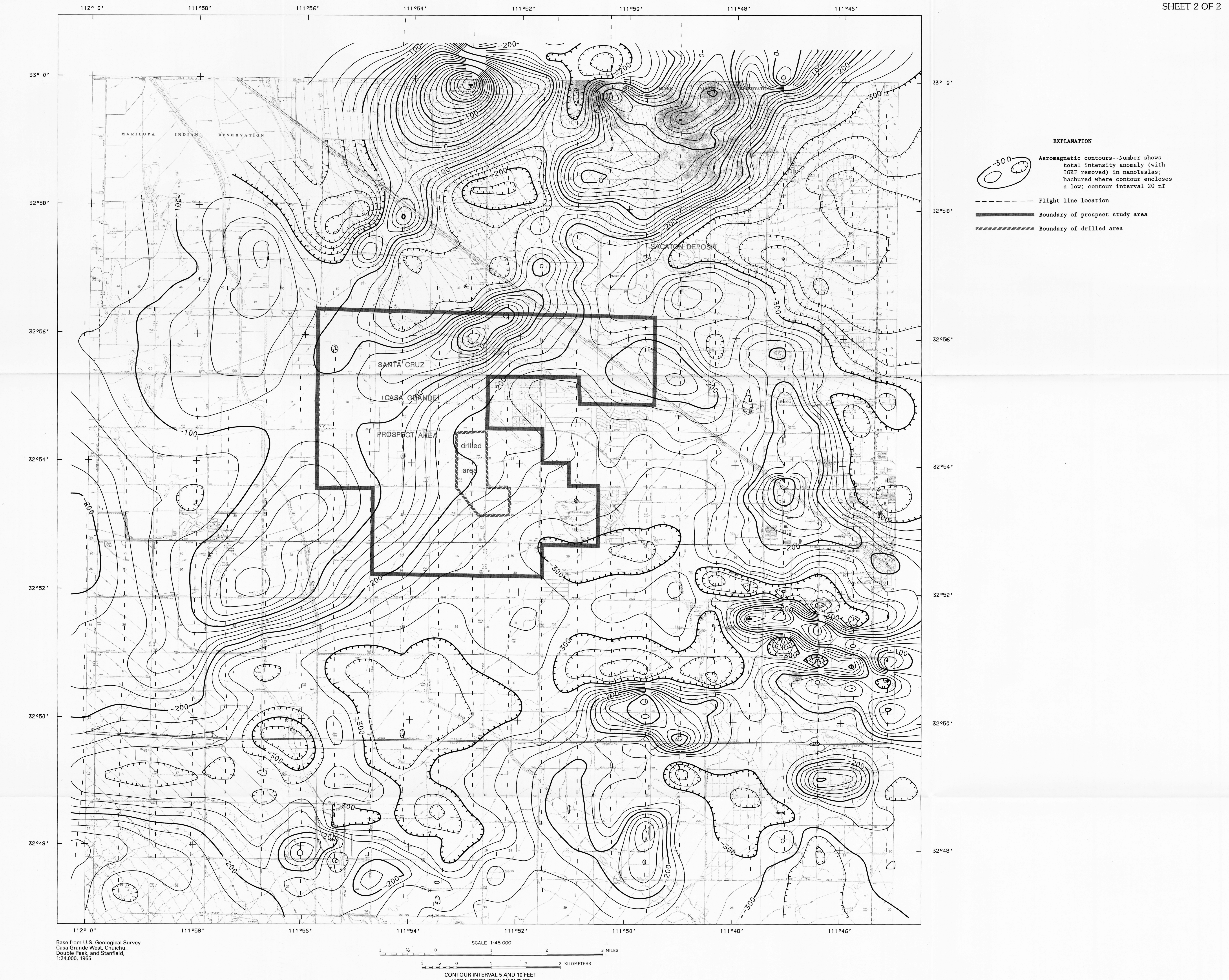
MAP B.--CASA GRANDE MAGNETIC ANOMALY MAP AT 600 FEET (183 METERS) ABOVE TERRAIN. FLIGHT LINES ARE APPROXIMATELY 0.5 MILES (0.8 KILOMETERS) APART
