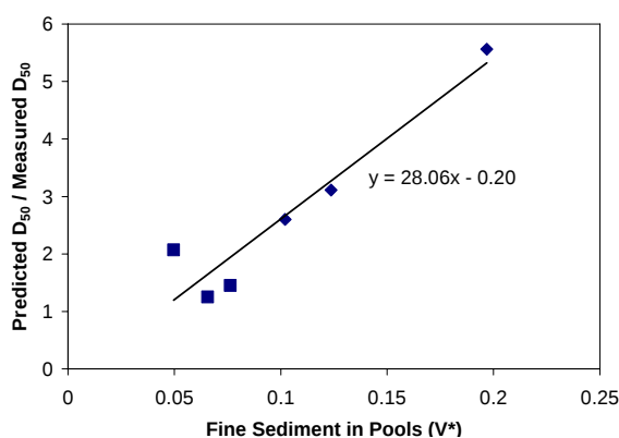
Figure 2 Ratio of predicted median grain size to fine measured median grain size, versus reach-averaged V^* .
