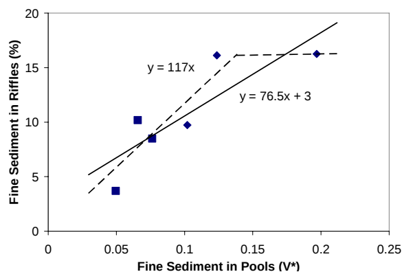
Figure 1 Percentage of riffle bed surface covered by sediment versus reach-averaged V^* . Two models are presented, a linear regression (solid line) and a broken-stick regression (dashed line).
