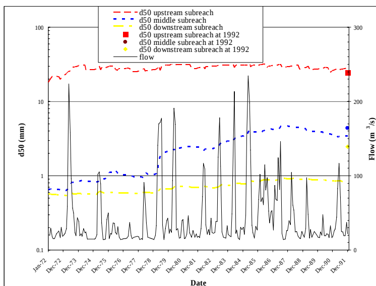
Figure 5 Change in median bed material size ( d_{50} ) during model simulation from 1972-1992.
