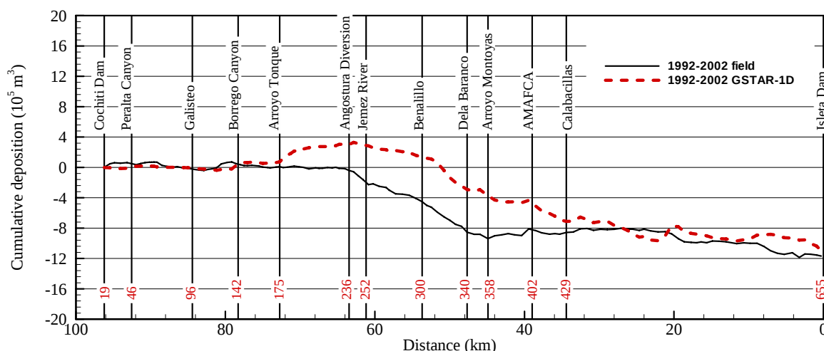
Figure 2 Cumulative total volume of sediment from 1992 to 2002.
