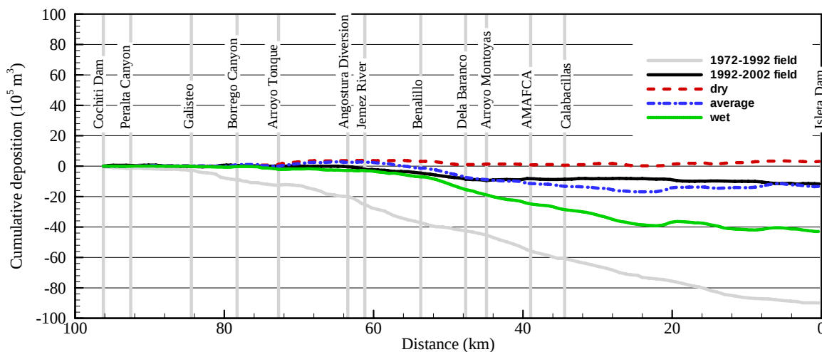
Figure 6 Cumulative main channel volume of sediment 2002-2022.
