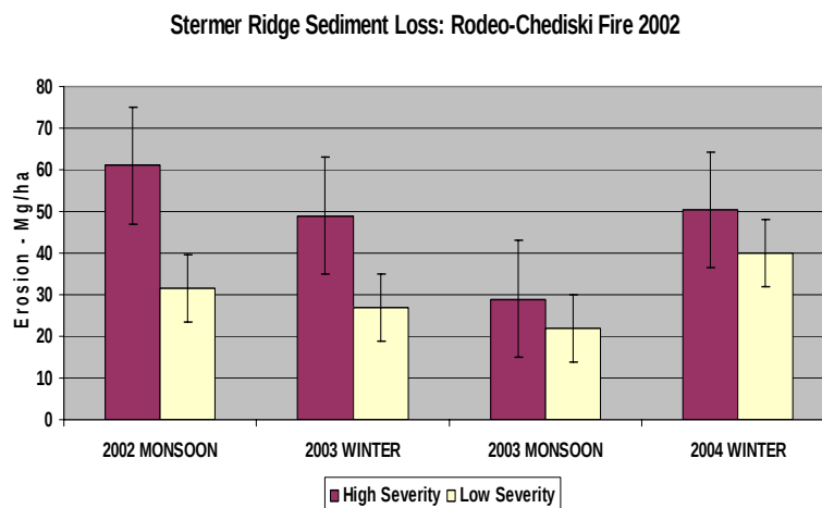
Figure 1 Sediment loss from Stermer Ridge Watersheds, Rodeo-Chediski Wildfire 2002, first four precipitation periods (Adapted from Garcia et al. 2005 and Stropki et al. In Press).
