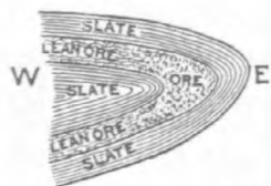
FIG. 14.—Sketch to illustrate the occurrence of ore bodies.
