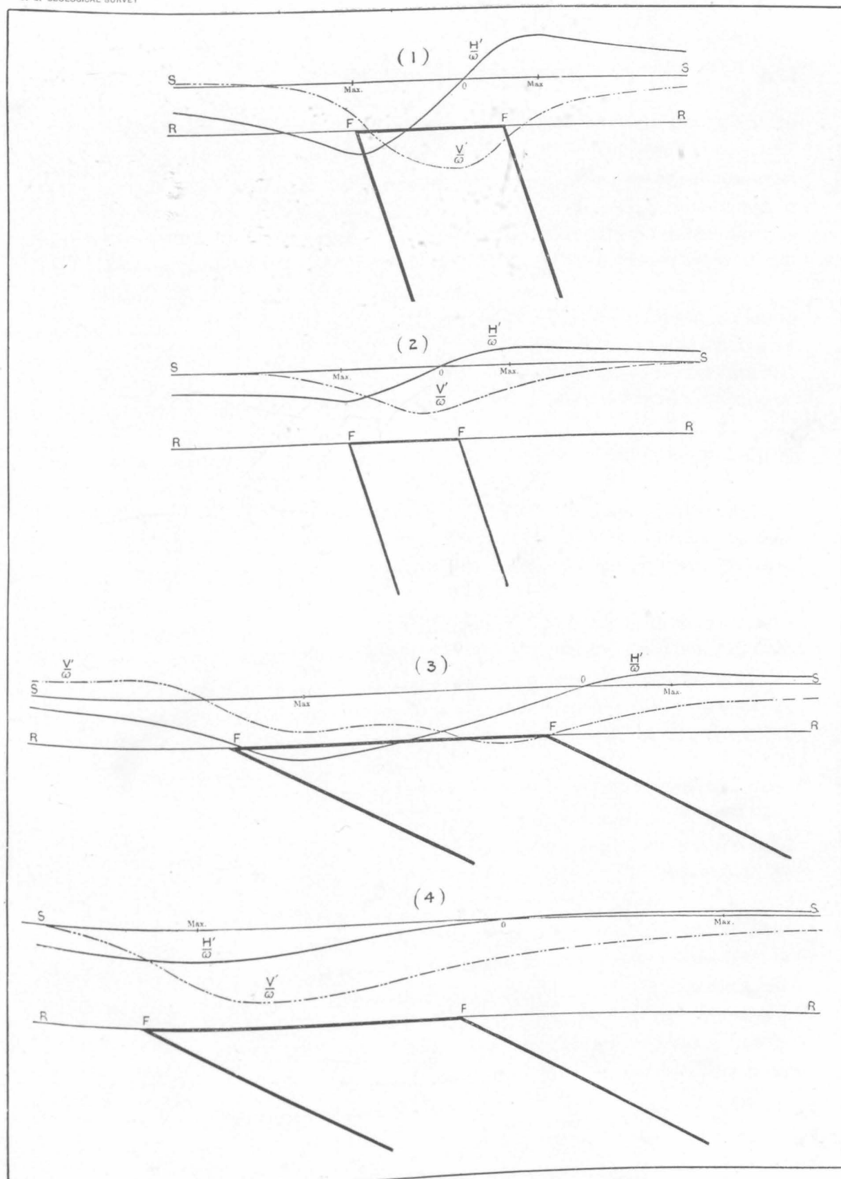
RELATIONS OF MAGNETIC BEDS TO VARIATION AND DIP.
