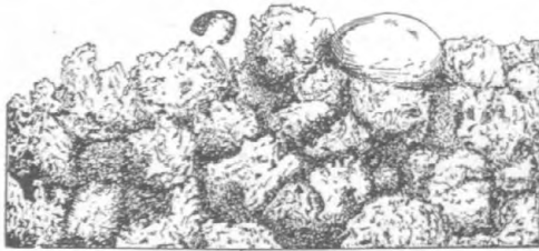
Fig. 10.—Reproduction of illustration of aa lava, after Dana (Characteristics of Volcanoes).
