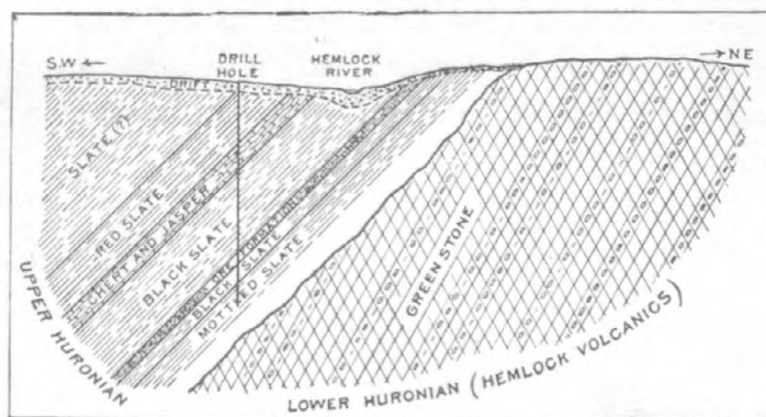
FIG. 11.—Profile section illustrating results of diamond-drill work.
