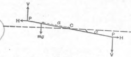
Fig. 17.—The forces acting on the dip needle.
