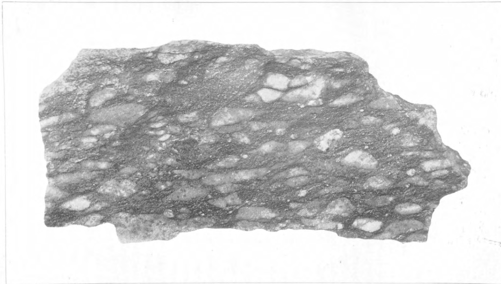
SCHIST CONGLOMERATE FROM DAM OF STURGEON RIVER, NEAR THE NORTHWEST CORNER OF SEC. 17, T. 42 N., R. 28 W.
