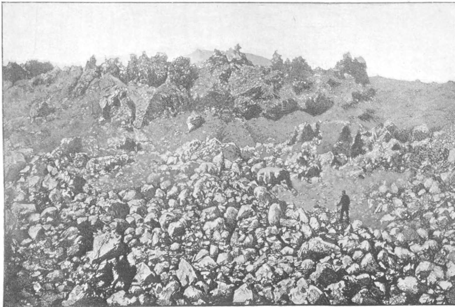
MOUNT GIORGIOS, VIEWED FROM ITS WEST FLANK, IN APRIL, 1866, ILLUSTRATING THE CHARACTERISTIC BLOCK LAVAS.
