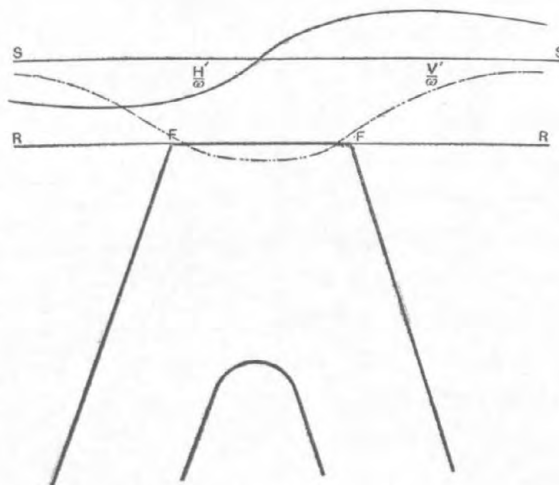
Fig. 20.—Truncated anticlinal fold with steeply dipping limbs.
