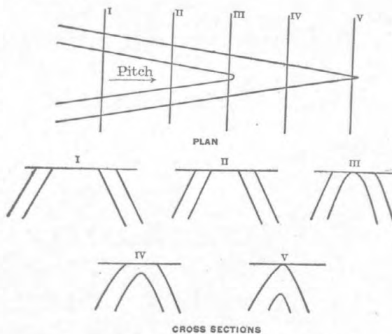
Fig. 23.—Plan and cross sections of a pitching anticline.
