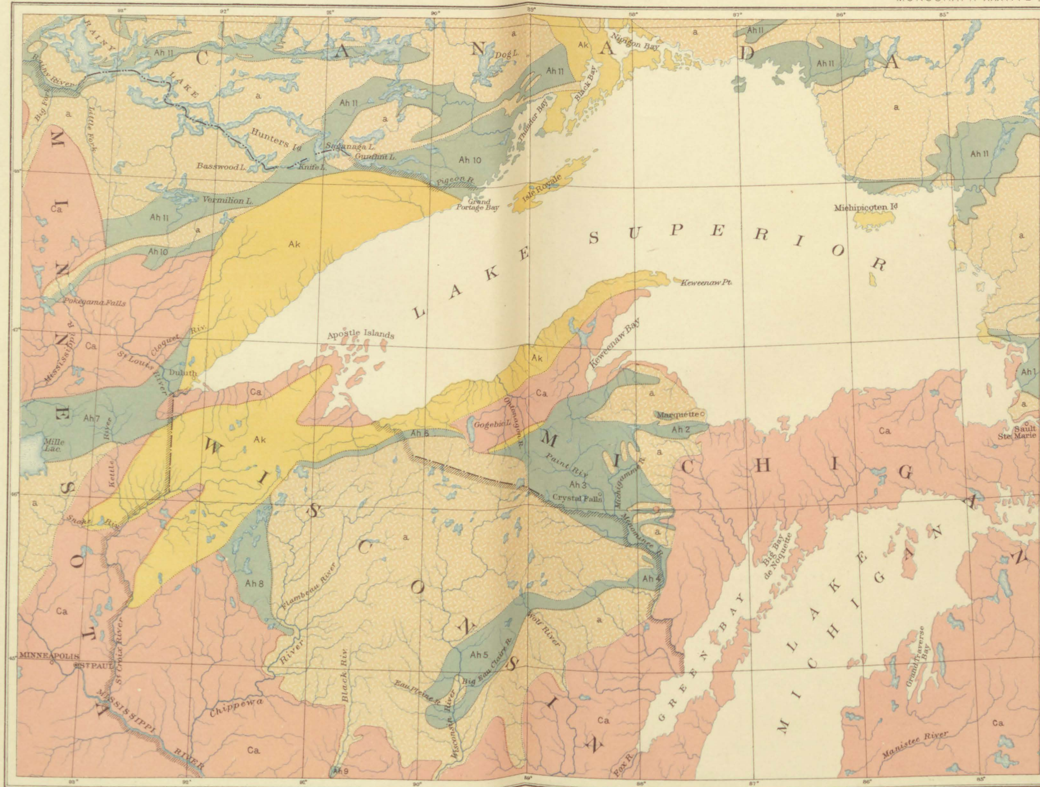
ARCHEAN ALGONKIAN POST-ALGONKIAN HURONIAN KEWEENAWAN a Ah Ak Ca GEOLOGIC MAP OF PART OF THE LAKE SUPERIOR REGION Compiled from Official maps of U. S. Minnesota, and Canadian Surveys
