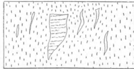
FIG. 4.—Granite-porphry with inclusions of gneissoid granite.
