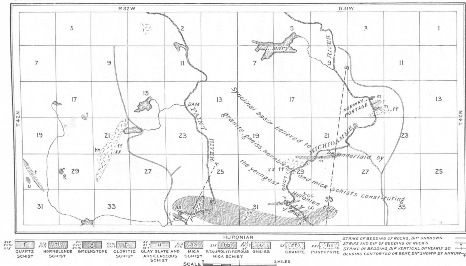
PORTION OF A GEOLOGICAL MAP OF THE MENOMINEE IRON REGIONS, BY T. B. BROOKS AND C. E. WRIGHT.
