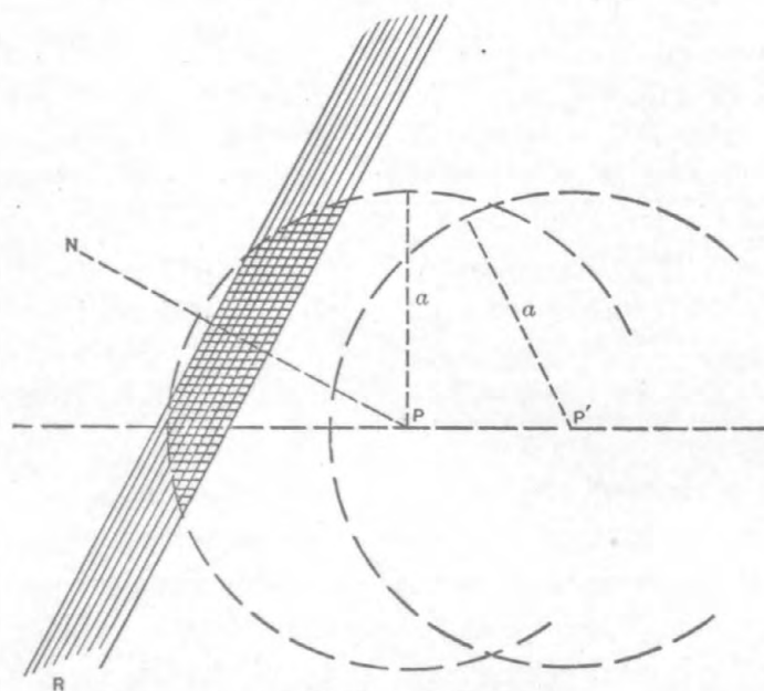
Fig. 16.—Circles of attraction.
