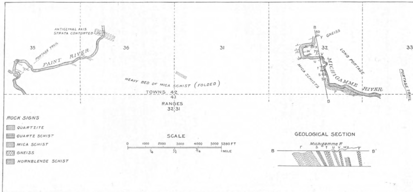
PORTION OF BROOKS'S PL. IX, VOL. III, WISCONSIN GEOLOGICAL SURVEY, SHOWING DETAILS ON PAINT AND MICHIGAMME RIVERS.
