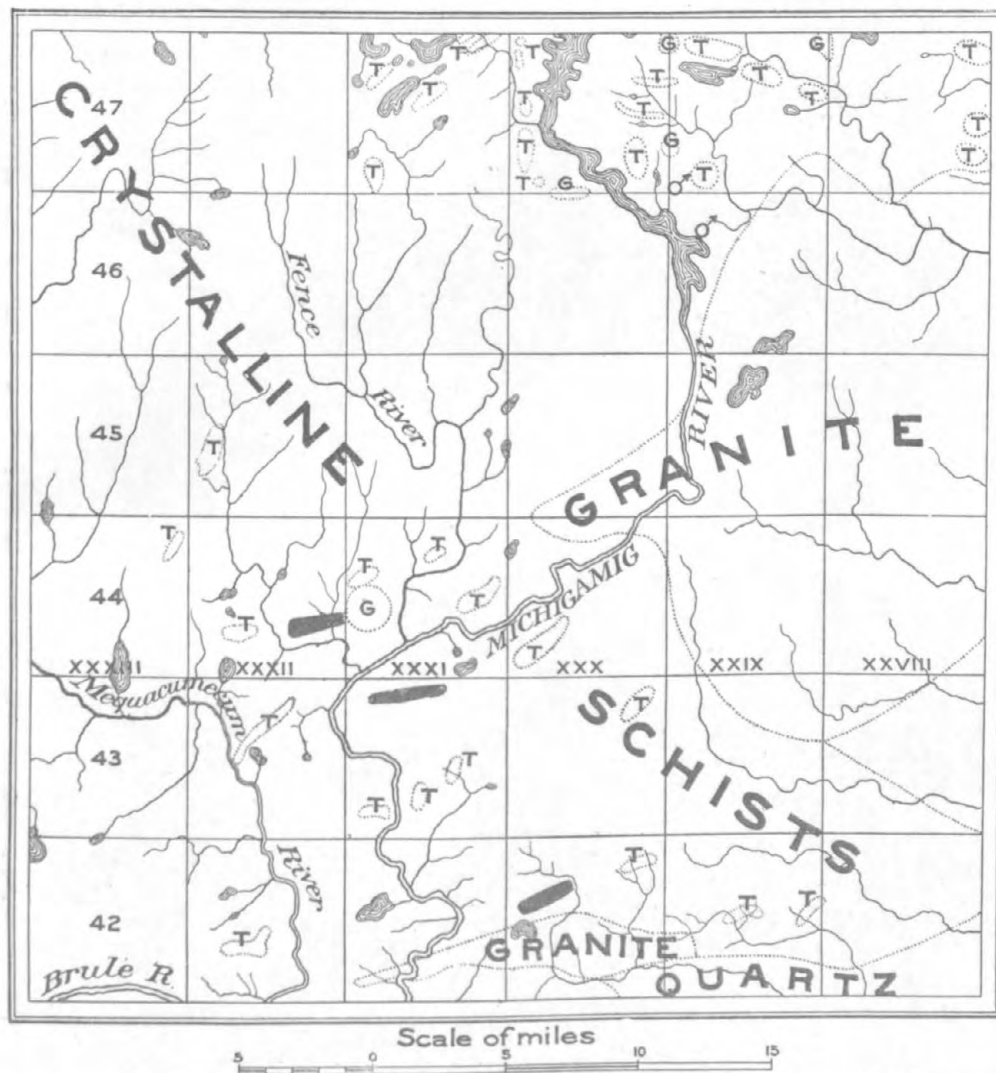
FIG. 2.—Enlarged reproduction of a portion of a map of the Lake Superior land district, by Foster and Whitney. G=granite; T=trappean rocks; ♂=iron; ■=beds of marble.
