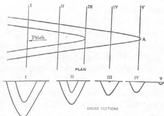
FIG. 21.—Plan and cross sections of a pitching syncline.
